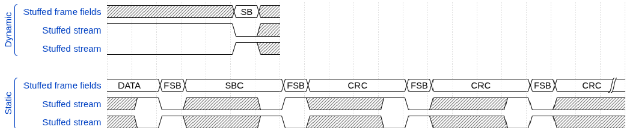
Figure 6: Dynamically and statically bit-stuffed stream examples. In frame fields encoded with dynamic bit-stuffing an opposite polarity stuff bit (SB) is inserted after five consecutive same-polarity bits. In frame fields encoded with static bit-stuffing (SBC and CRC in FD frames) a fixed stuff bit (FSB) is inserted after each fourth bit. A FSB is also inserted before the first bit of the SBC field.
