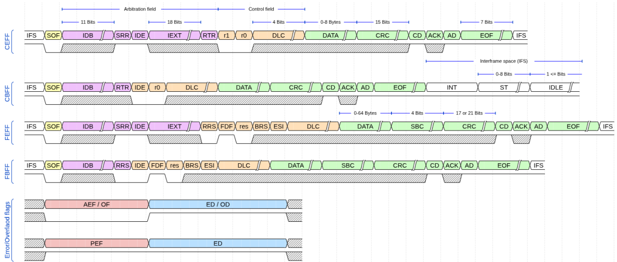
Figure 4: Frame and error flag formats for CAN-CC Base, CAN-CC Extended, CAN-DF Base and CAN-DF Extended. Widths of truncated multi-bit fields are tabulated in Table 4.
