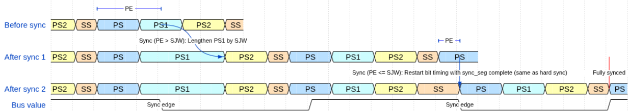
Figure 6: Resynchronization over two successive sync edges. PE is the phase error relative to SS. SJW is the Synchronization Jump Width.
