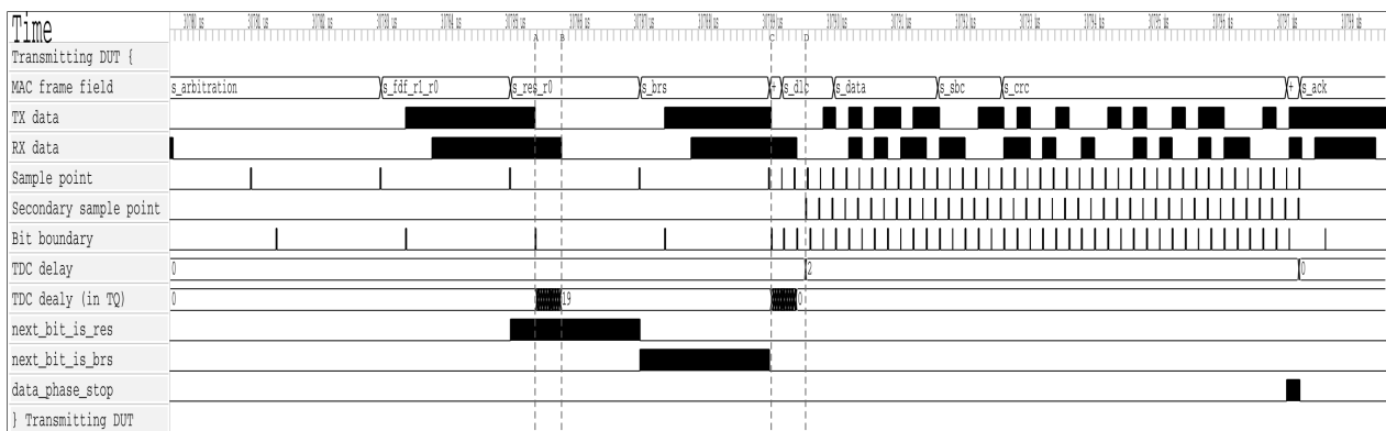
Figure 21: Dual bit rate switching and TDC measurement in a CAN FD MAC frame. The TDC measurement starts at the transmission of the dominant res bit edge (A) and stops when the echo returns at RX (B). At the transmission of the ESI bit (C) the measured TDC delay is counted down and the secondary sample point strobes starts when the count down terminates (D). TDC delay is the measured delay in how The MAC controls the initiation of the TDC delay measurement through next_bit_is_res and bit rate switching through next_bit_is_brs and data_phase_stop. Waveform from can_mac_pcs_fce_tb.
