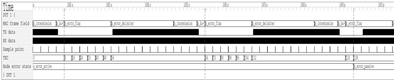
Figure 23: Active error frame sequence in can_mac_pcs_fce_tb following a forced bit error in the data field. DUT 1 detects first bit error at A after driving the dominant SOF bit and sampling recessive. DUT 1 starts transmission of the second error flag at B and goes error passive at C.
