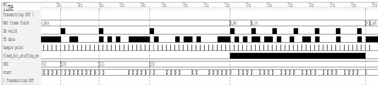
Figure 20: Dynamic and fixed bit stuffing in a CAN FD MAC frame. Three dynamic stuff bit insertions in the TX data stream (A, B, C). Seven fixed stuff bit insertions in the TX data stream between D and E. Waveform from can_mac_pcs_fce_tb.
