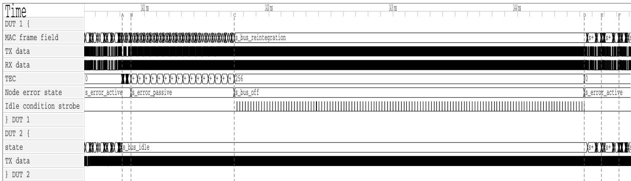
Figure 24: Bus-off recovery in can_fce_tb , showing the 128 idle-condition pulses required before TEC/REC reset and return to error active.
