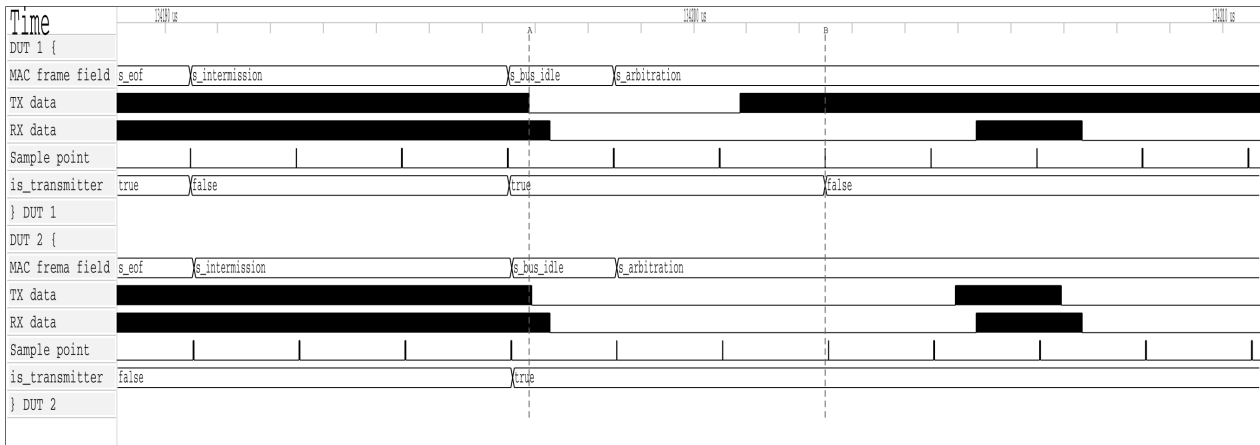
Figure 22: Arbitration loss in can_mac_pcs_fce_tb . Both nodes start transmitting ( is_transmitter = true ) at the same time (A). The DUT 1 node loses arbitration at B after transmitting recessive and sampling dominant and continues as receiver ( is_transmitter = false ). Waveform from can_mac_pcs_fce_tb .
