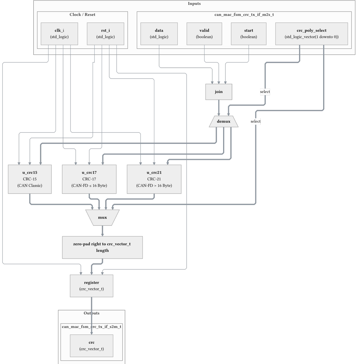
Figure 9: can_mac_crc_tx selection architecture. Three CRC engine instances run in parallel. The FSM drives crc_poly_select to gate valid and start per engine so that only the selected polynomial accumulates data. A registered output mux selects the active engine result and zero-pads it into the common crc_vector_t format.
