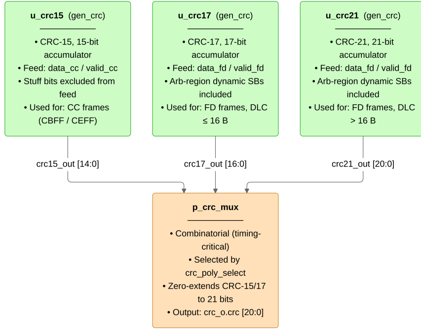
Figure 15: can_mac_crc dataflow with three parallel CRC engines. The output mux is combinatorial to satisfy the ISO \text{IPT} \leq 2 \text{ t}_q constraint at minimum prescaler.
