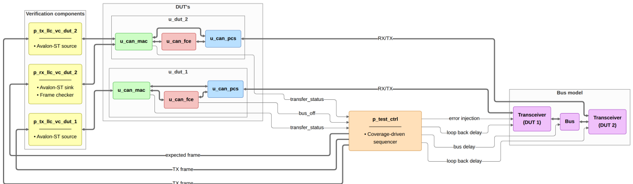
Figure 18: can_mac_pcs_fce_tb integration testbench. Two can_mac_pcs_fce instances connect through a dominant-wins bus model. Avalon-ST VCs drive and sample the MAC interfaces. p_test_ctrl sequences test stimuli, injects bit errors via dut_1_rx_recessive , and reads pass/fail status from the TX status and bus-off monitors.
