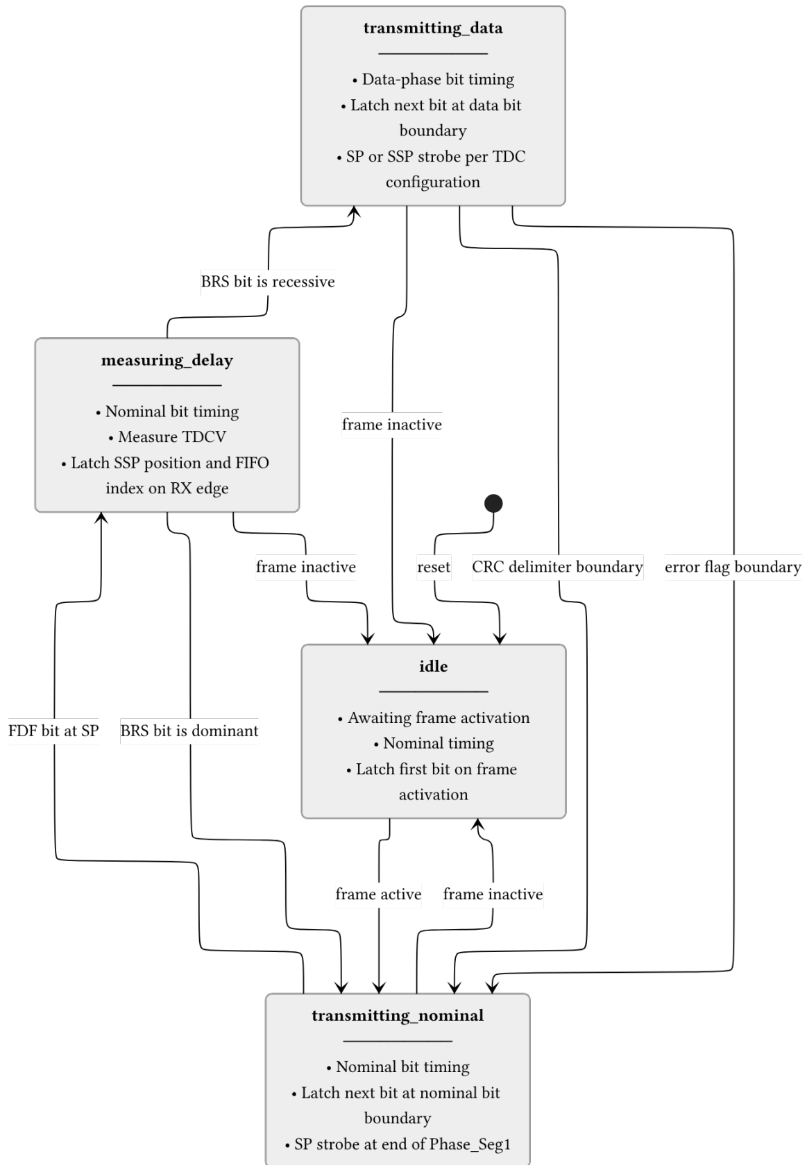
Figure 7: PCS TX FSM state transitions. The measuring_delay state is entered on the FDF sample point to measure TDCV (Transmitter Delay Compensation Value, ISO ref.: 7.3.4). The BRS bit boundary determines whether data-phase timing is used. All non-idle states return to idle when the frame becomes inactive.
