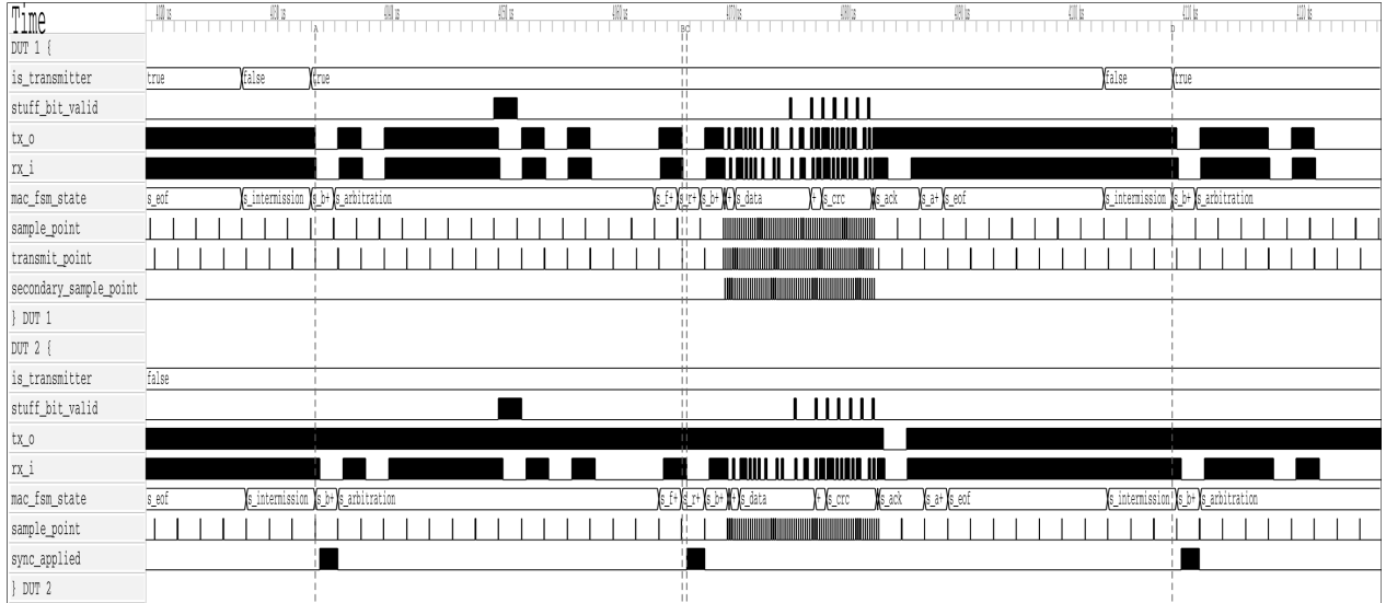
Figure 19: Two-node simulation of a complete FD frame in can_mac_pcs_fce_tb, showing the full field sequence from s_arbitration through s_eof on both transmitter and receiver. Secondary sample point pulses confirm TDC is active during the data phase. Resynchronization events are visible on DUT 2 via sync_applied.
