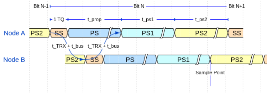
Figure 5: CAN bit time segments (SS, PS, PS1, PS2) and Sample Point (SP). The two-node layout illustrates the round-trip propagation delay ( t_{TRX} + t_{bus} each way) that PS must cover for correct arbitration.
