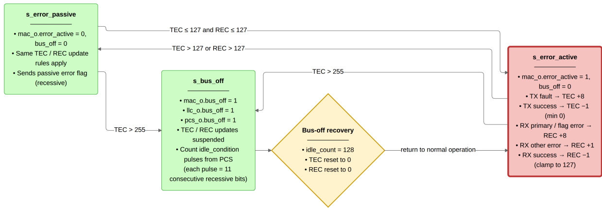
Figure 16: can_fce FSM (ISO 11898-1 sec. 8.1.4.4, Figure 43). s_error_active is the initial state after reset_i or llc_i.normal_mode . When TEC exceeds 127 or REC exceeds 127 the FCE moves to s_error_passive , clearing mac_o.error_active . If TEC exceeds 255 from either active or passive state, the FCE enters s_bus_off , asserting bus_off to the MAC, LLC, and PCS. Recovery counts 128 idle_condition pulses from the PCS (each pulse represents 11 consecutive recessive bits); on the 128th pulse TEC and REC are reset to zero and the FSM returns to s_error_active .
