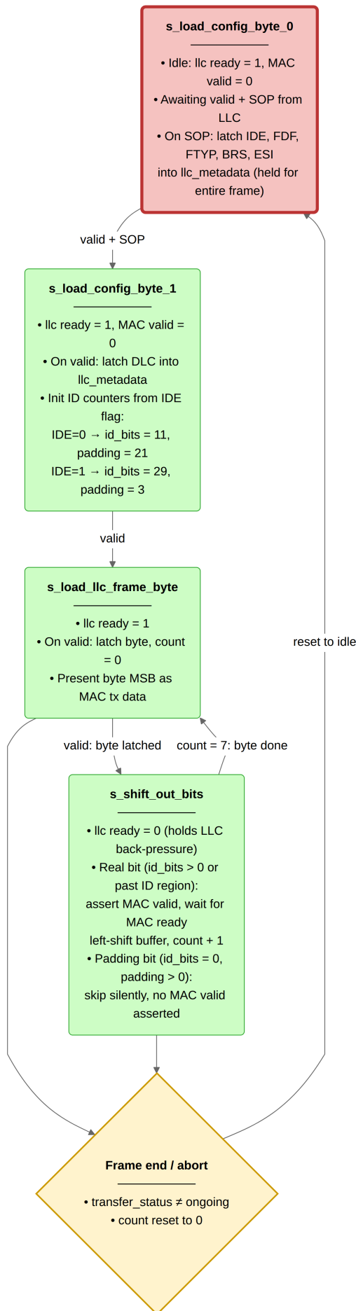
Figure 13: can_mac_ser (4 states). Config bytes carry frame metadata (IDE, FDF, FTYP, BRS, ESI, DLC); these are latched once and held stable for the entire frame. In s_shift_out_bits real ID and data bits are driven one per MAC FSM ready pulse, while unused padding bits in the 32-bit ID field are skipped silently. Any transfer_status ≠ ongoing signal from the MAC FSM returns the serializer
