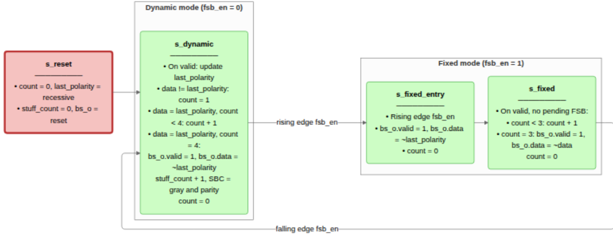
Figure 14: can_mac_bs (2 modes). Dynamic mode counts consecutive identical bits and emits an inverse stuff bit on the 5th ( count = 4 ), updating the Gray-coded SBC. Fixed mode is entered on the rising edge of fsb_en , which immediately emits the initial FSB; thereafter one FSB is emitted every 4 real bits ( count = 3 ). The falling edge of fsb_en cancels any pending FSB and returns to dynamic mode. stuff_count and the SBC output are maintained continuously across both modes.
