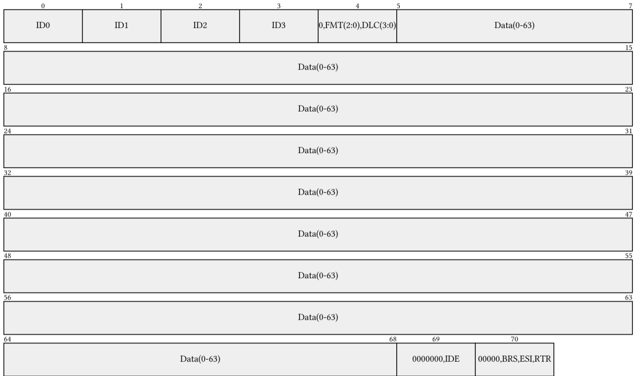
Figure 10: Revised LLC frame format with FD support, shown at maximum length (71 bytes). The FMT field selects frame type; BRS and ESI repurpose reserved bits in the final byte. ID byte encoding is defined in Table 4.
