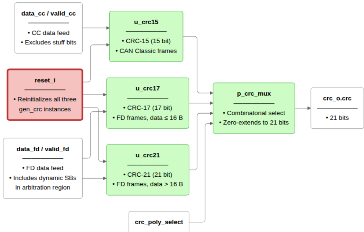
Figure 15: can_mac_crc dataflow. Three gen_crc instances accumulate in parallel on every clock: u_crc15 is fed by data_cc/valid_cc (CC bit stream, stuff bits excluded); u_crc17 and u_crc21 are both fed by data_fd/valid_fd (FD bit stream, dynamic stuff bits included in the arbitration region). The combinatorial mux p_crc_mux selects the active engine result based on crc_poly_select and zero-extends it to the common 21-bit output. reset_i reinitializes all three engines simultaneously.
