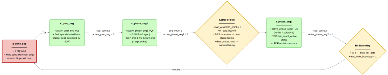
Figure 17: can_pcs bit-timing segment machine (ISO 11898-1 sec. 7.2-7.3). The four segments cycle continuously from reset. s_sync_seg is 1 TQ fixed; a dominant edge here triggers hard synchronization, restarting from s_prop_seg . Soft synchronization in s_prop_seg and s_phase_seg1 extends phase_seg1 by up to SJW TQs; in s_phase_seg2 it shortens by up to SJW TQs. The SP strobe fires at the end of s_phase_seg1 ; the BRS recessive condition at that SP switches active_prop_seg , active_phase_seg1 , and active_phase_seg2 to data-phase generics. The SSP fires one TQ before the SP when ssp_active is set. The TX bit is driven and the bit boundary is signalled at the end of s_phase_seg2 .
