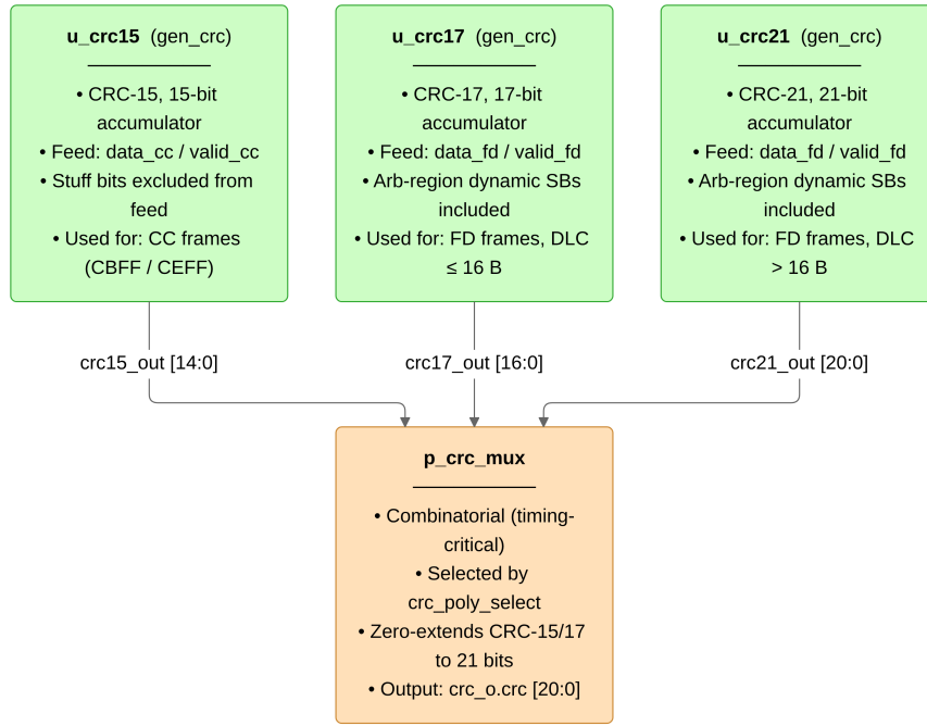
Figure 15: can_mac_crc dataflow with three parallel CRC engines. The output mux is combinatorial to avoid one cycle of read latency at the FSM.
