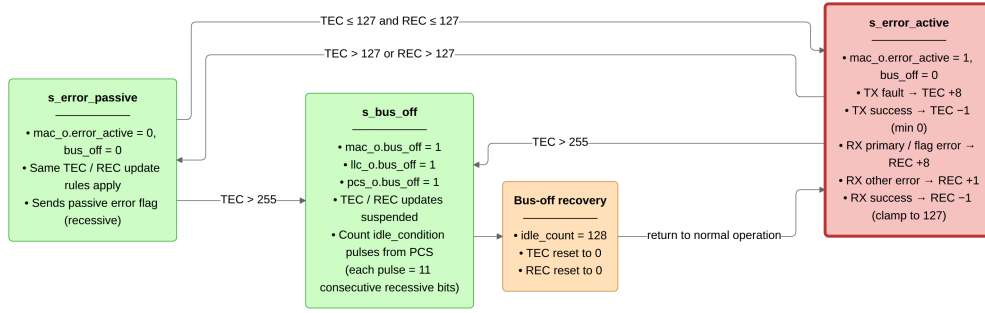
Figure 16: can_fce FSM governing the error active, error passive, and bus off node states per ISO 11898-1 sec. 8.1.4.4.
