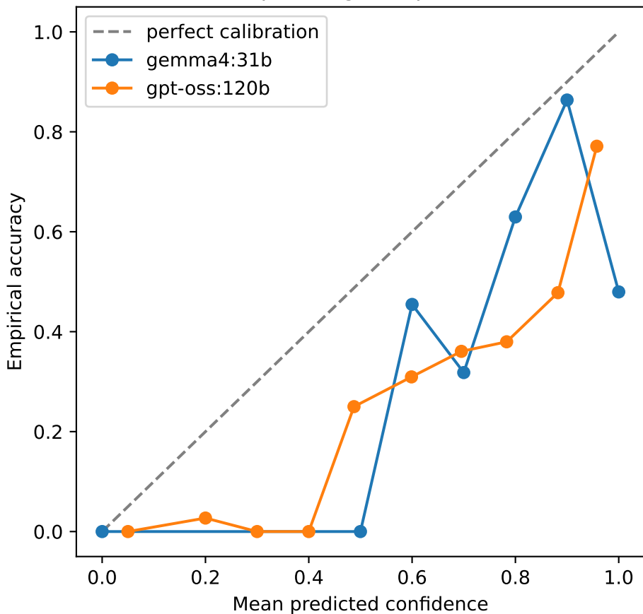
Calibration (sample-weighted pooled across tasks)
