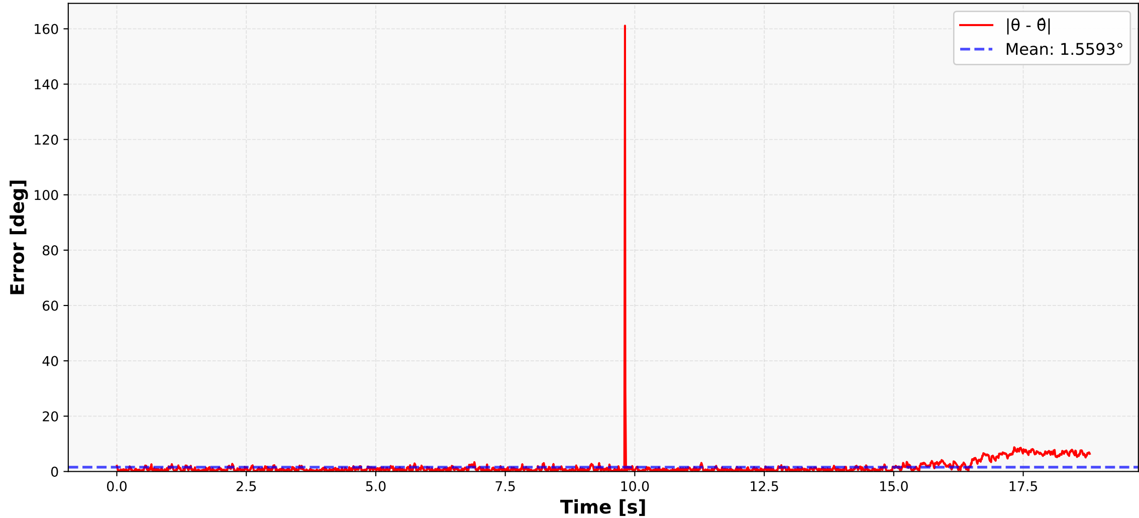
Heading (Yaw) Error vs Time
