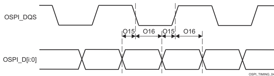
Figure 6-97. OSPI0 Timing Requirements – PHY Data Training, DDR with DQS
