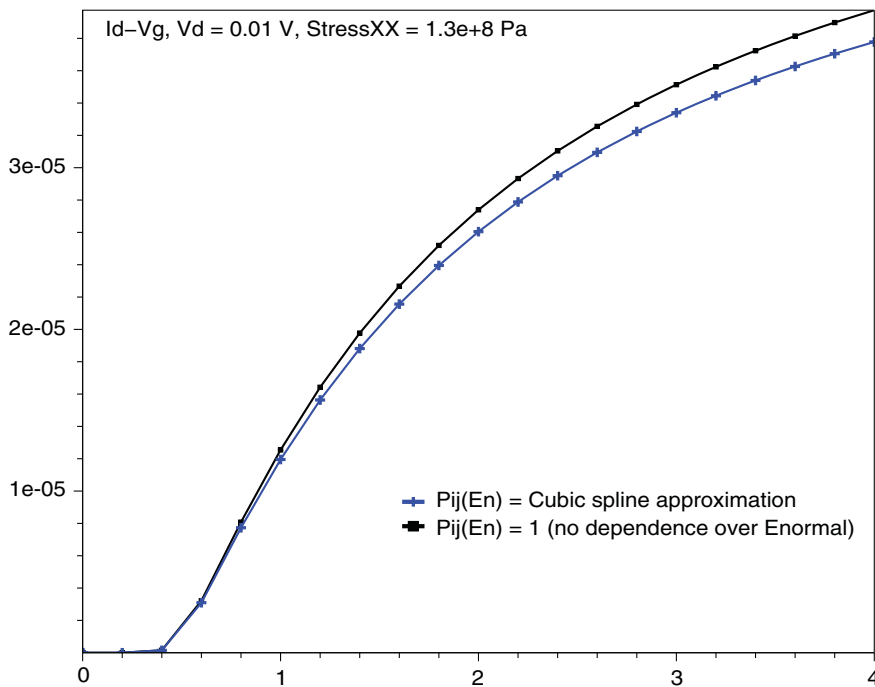
Figure 58 I_d - V_g curve, with Enormal -dependent piezo prefactors, shifts downwards
