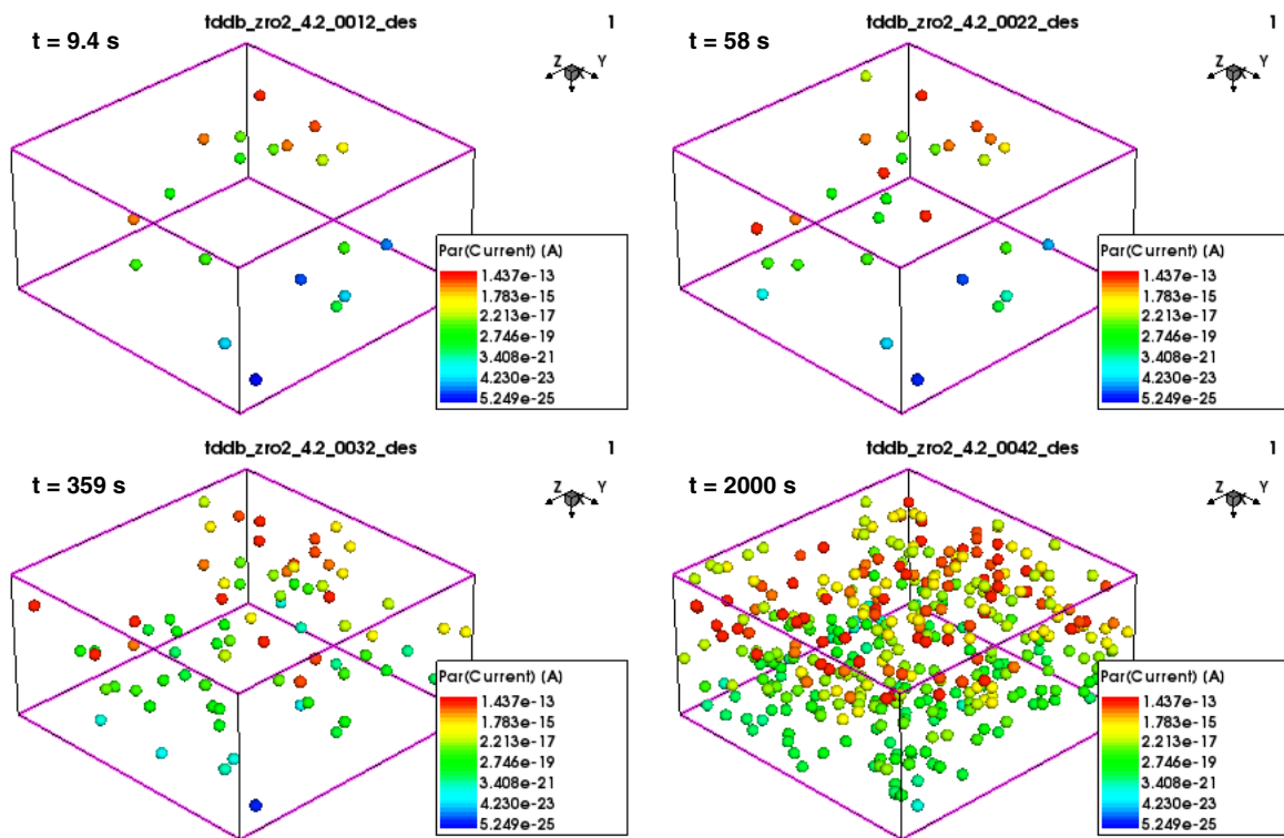
Figure 79 Defects in the MIM structure with V(\text{anode}) = 4.2 \text{ V} at times (upper left) 9.4 s, (upper right) 58 s, (lower left) 359 s, and (lower right) 2000 s
