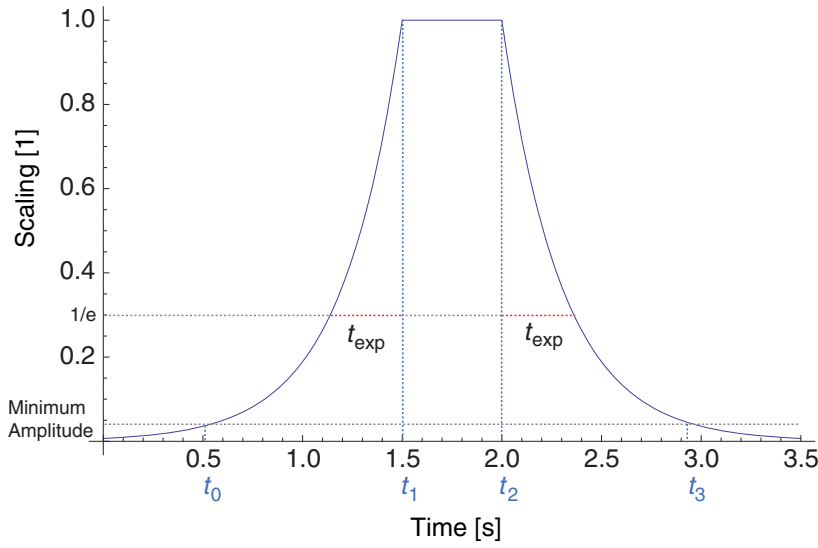
Figure 25 Rise and decay times based on an exponential function
