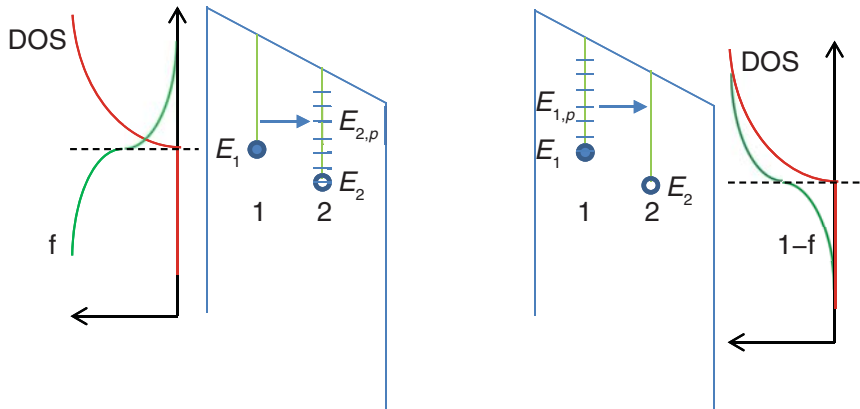
Figure 74 (Left) Capture and (right) emission between two defects
