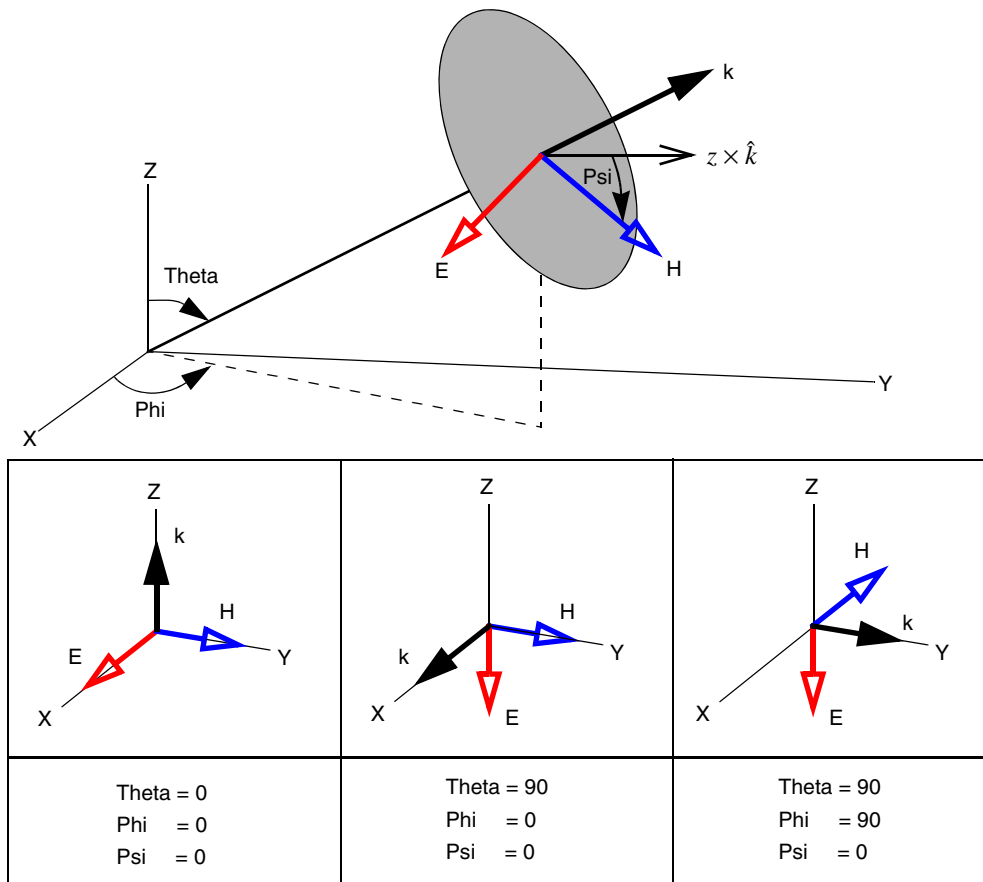
Figure 28 Definition of coordinate system for 3D plane wave excitation and examples of parameters of 3D plane wave
