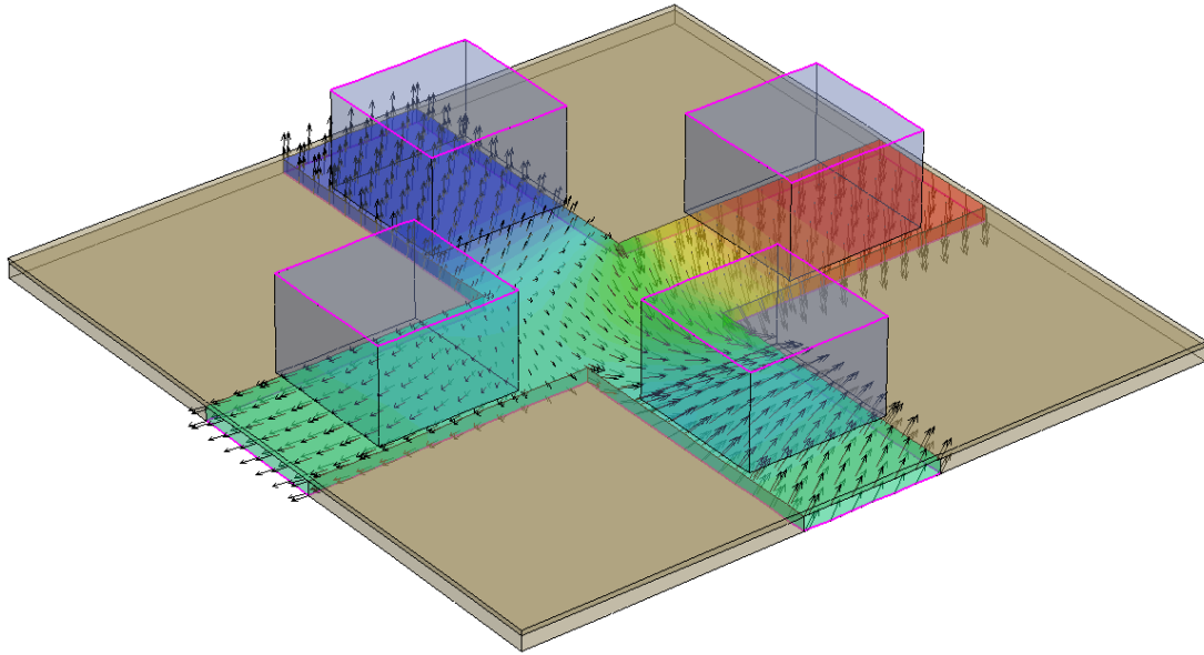
Figure 54 Snapshot of position-dependent magnetization direction in a spin-torque majority gate; the pinned layer is split into four pieces, and the MTJs with different applied voltages compete for switching of the cross-shaped free layer
