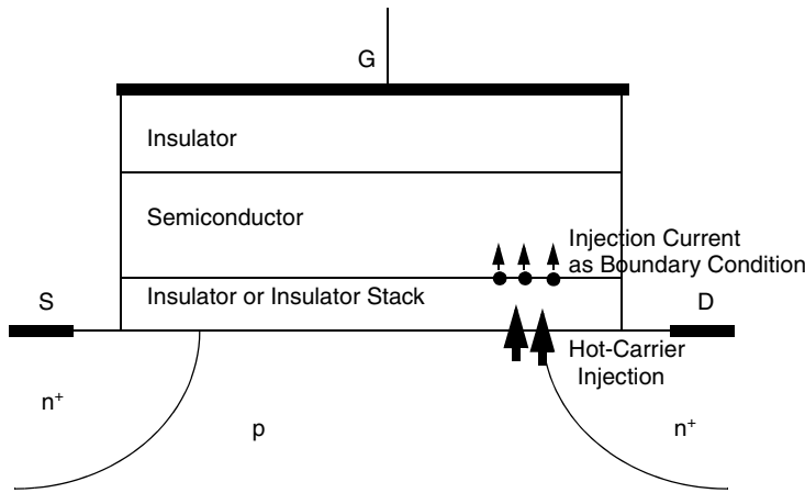
Figure 51 Injection of hot-carrier current in a MOSFET structure
