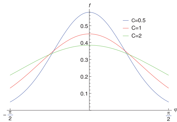
Figure 40 ADF of type Gauss
