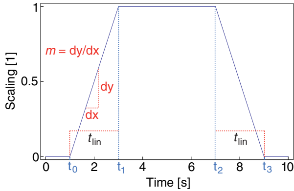
Figure 23 Rise and decay times based on a linear function
