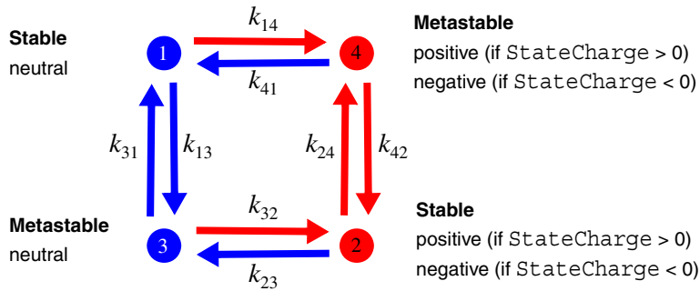
Figure 93 State diagram for the eNMP transition rates PMI
