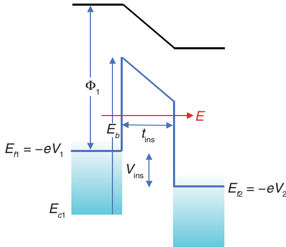
Figure 73 Direct tunneling in a MIM structure
