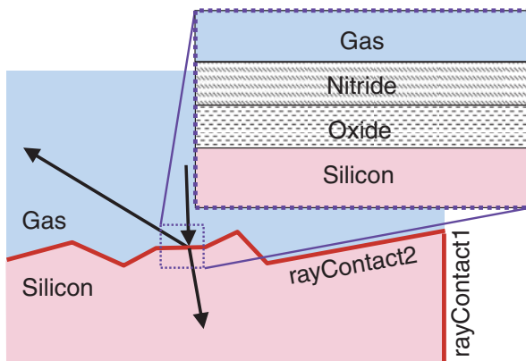
Figure 35 Illustration of thin-layer-stack boundary condition for simulation of an antireflection-coated solar cell
