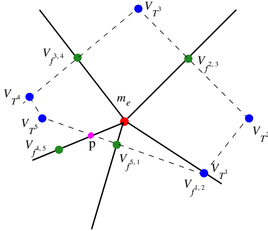
Figure 82 Element 5 is an obtuse element; the face of the Voronoï box is a polygon (V_{T^1}, V_{T^2}, V_{T^3}, V_{T^4}, V_{T^5}, V_{T^1}) , and all vertices are Voronoï element centers
