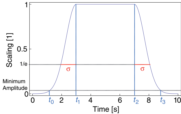
Figure 24 Rise and decay times based on a Gaussian function
