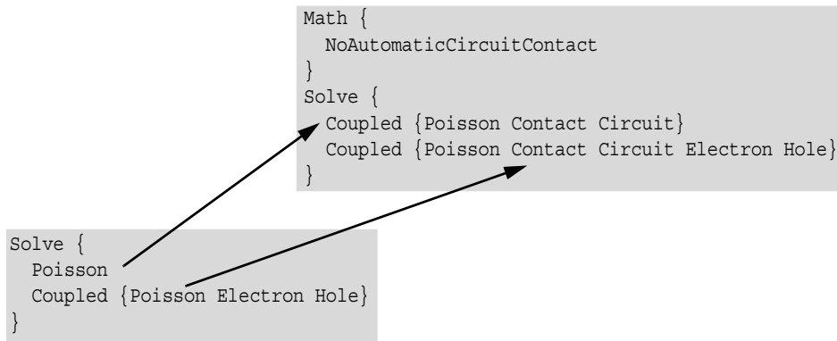
Figure 10 Translating default solve syntax to a NoAutomaticCircuitContact form
