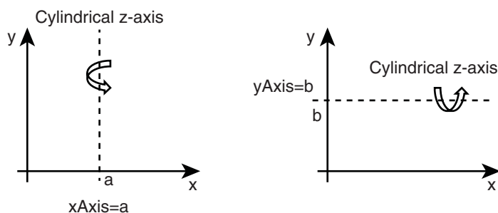
Figure 4 Cylindrical z-axis can be shifted along the axis of definition with the xAxis or yAxis option
