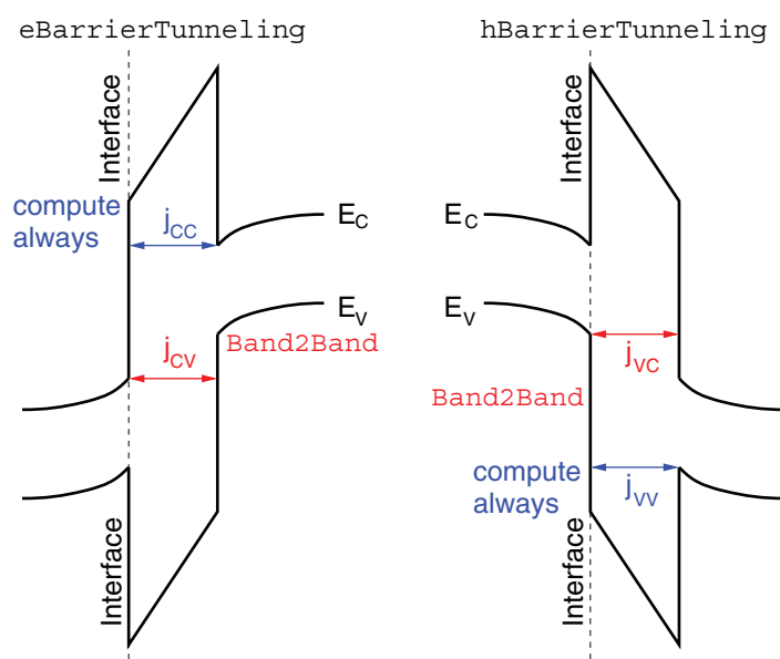
Figure 48 Various nonlocal tunneling current contributions
