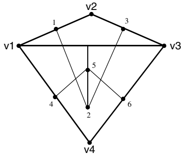
Figure 86 Violation of total-volume conservation for non-Delaunay mesh
