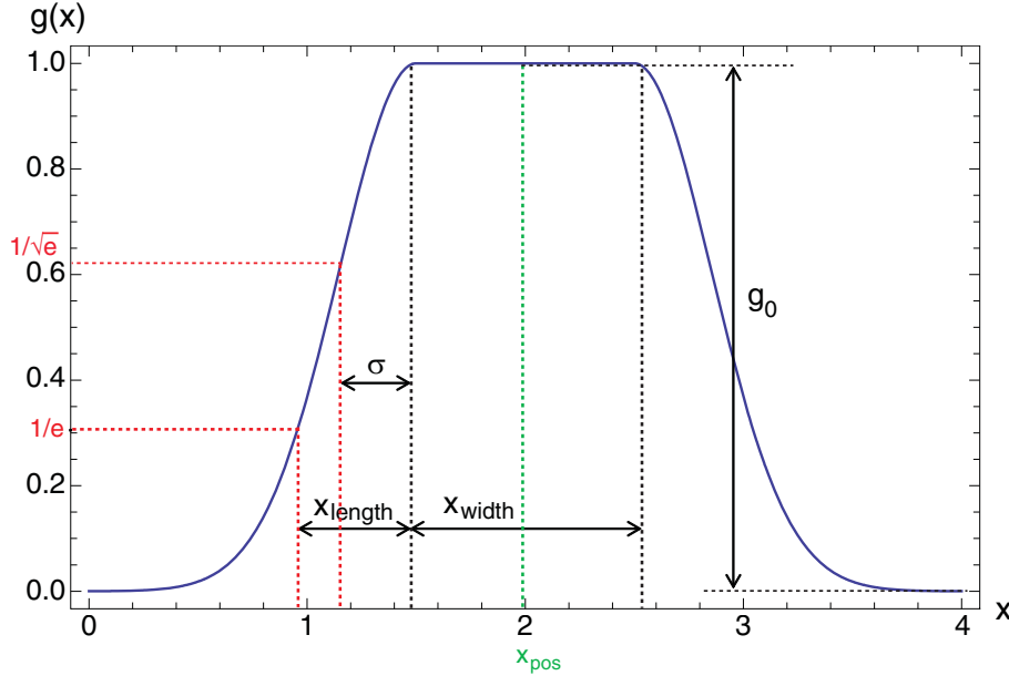
Figure 30 Gaussian spatial intensity distribution, showing the definition of key parameters
