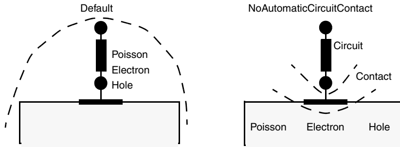
Figure 15 Range of equation keywords Circuit, Contact, Poisson, Electron, and Hole
