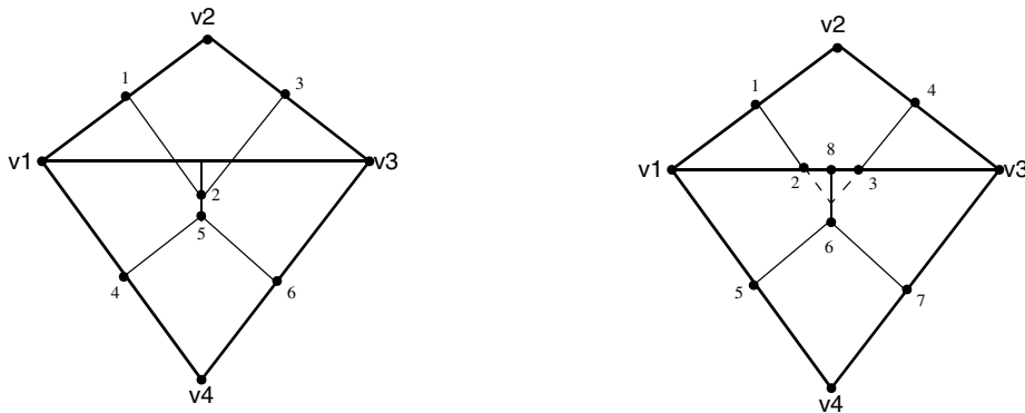
Figure 87 Algorithm truncation obtuse element: (left) Voronoï polygons before truncation – P1(v1, 1, 2, 5, 4, v1) , P2(v2, 1, 2, 3, v2) , P3(v3, 3, 2, 5, 6, v3) , P4(v4, 4, 5, 6, v4) ; (right) Voronoï polygons after truncation – P1(v1, 1, 2, 8, 6, 5, v1) , P2(v2, 1, 2, 3, 4, v2) , P3(v3, 4, 3, 8, 6, 7, v3) , P4(v4, 5, 6, 7, v4)
