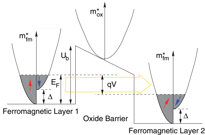
Figure 53 Schematic band diagram of an MTJ
