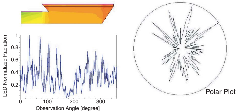
Figure 68 (Upper left) LED internal optical intensity, (lower left) normalized radiation intensity versus observation angle, and (right) polar radiation plot computed by Setaurus Device in 2D LED simulation
