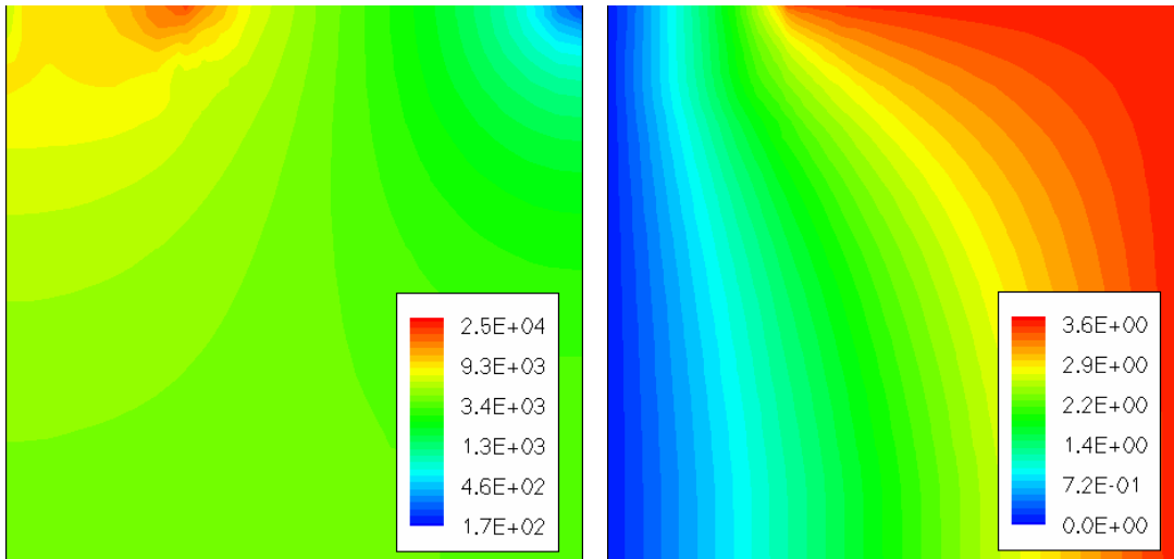
Figure 18 (Left) Total current density [ \text{Acm}^{-2} ] and (right) current potential [ \text{Acm}^{-1} ]
