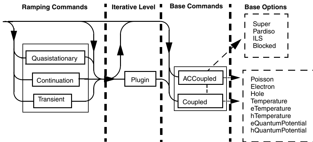
Figure 14 Different levels of Solve statements
