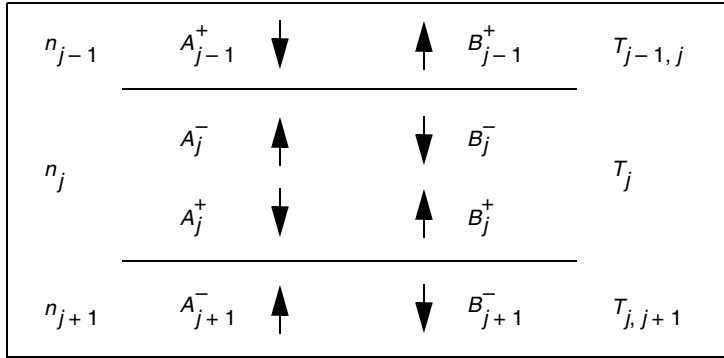
Figure 38 Wave amplitudes in a layered medium and transfer matrices connecting them
