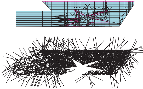
Figure 33 Applying the reflecting boundary condition in a 2D LED simulation; the boundary is drawn as a star inside the device
