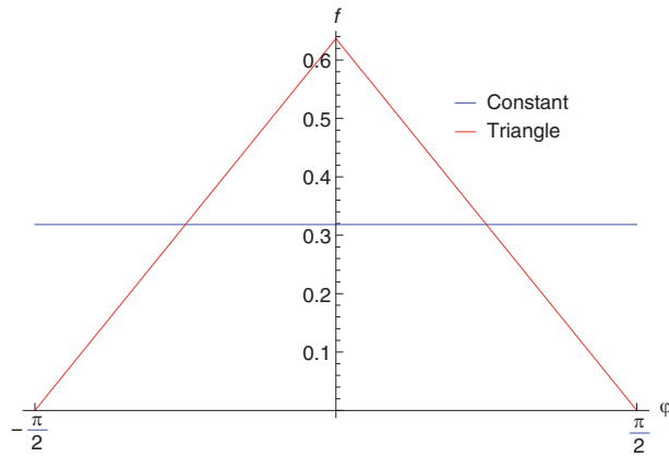
Figure 39 ADF of type Constant and Triangle
