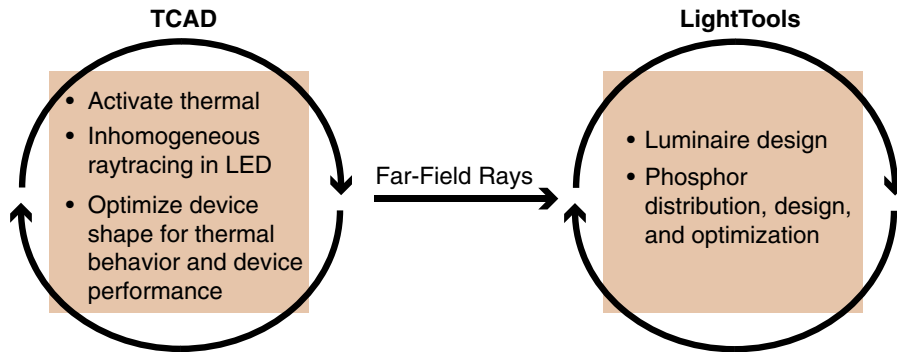
Figure 70 Secondary LED design flow to optimize luminaire design by LightTools and coupled to Sentaurus Device LED device simulation
