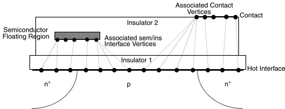
Figure 50 Mapping of hot interface vertices to associated contact or semiconductor–insulator interface vertices
