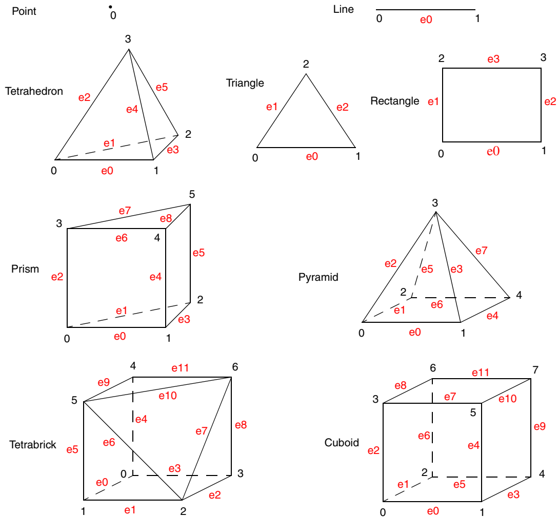
Figure 92 Vertex and edge numbering
