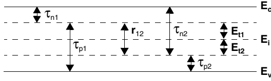
Figure 20 Notation for CDL recombination including all capture and emission processes
