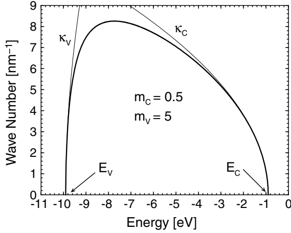
Figure 49 Comparison of two-band and single-band dispersion relations
