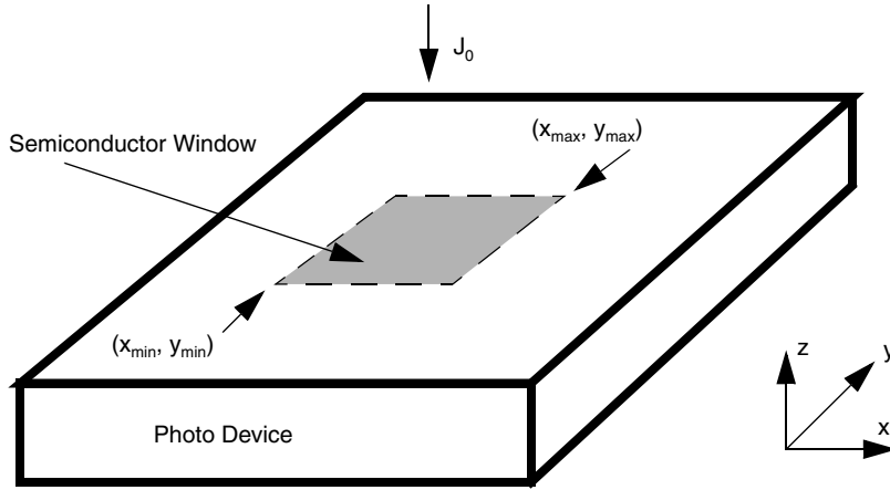
Figure 44 Intensity distribution of an optical beam modeled by a rectangular illumination window
