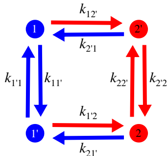
Figure 22 State diagram for the eNMP model
