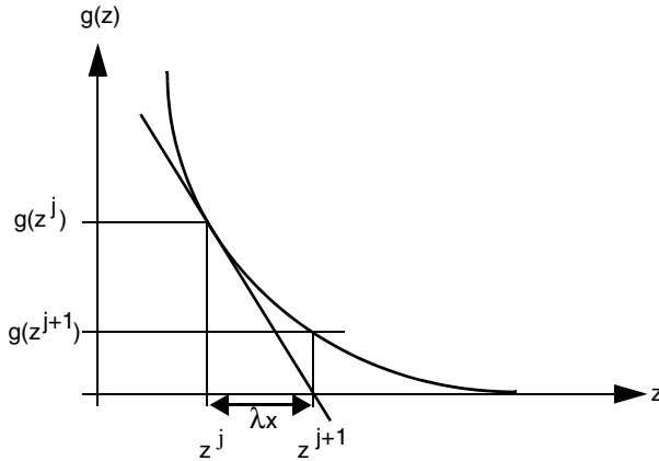
Figure 91 Newton iteration
