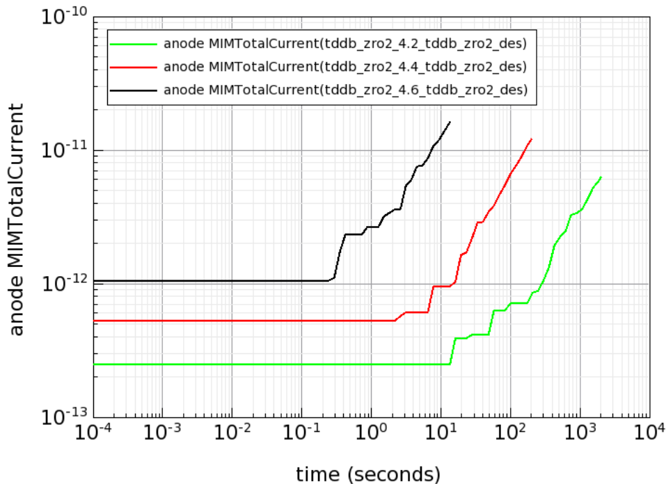
Figure 78 MIM current versus time for V(\text{anode}) = 4.2 V, 4.4 V, and 4.6 V
