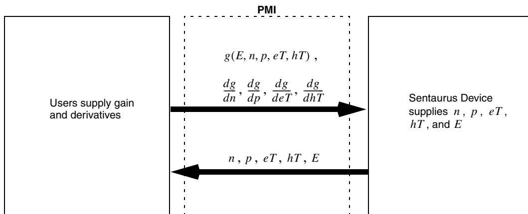
Figure 71 Illustration of the gain PMI concept
