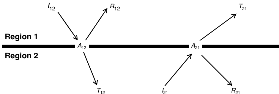
Figure 36 Distinguishing directional photon flux
