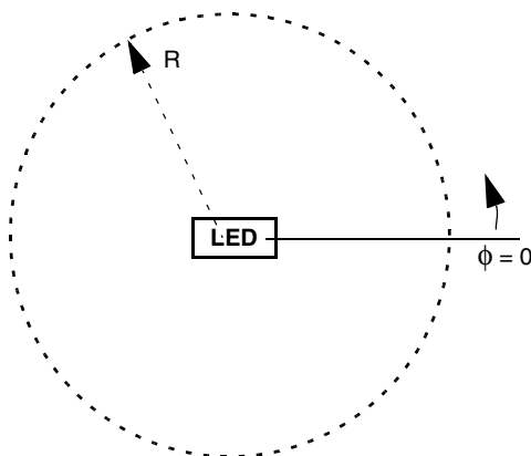
Figure 67 Measuring the radiation pattern in a circular path around LED at observation radius, R
