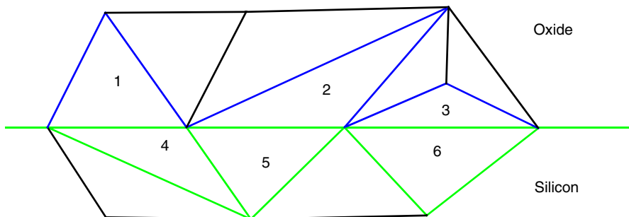
Figure 90 Blue (1, 2, 3) and green (4, 5, 6) elements are oxide and silicon interface elements, respectively. Elements 2 and 4 are non-Delaunay elements, not interface non-Delaunay elements. Only element 3 is an interface non-Delaunay element.
