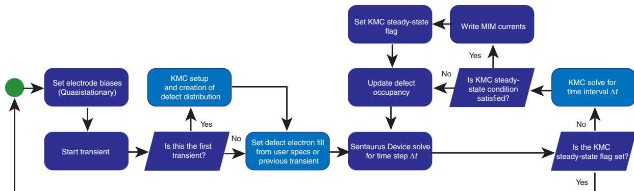
Figure 76 Typical Sentaurus Device/KMC flow for MIM leakage current simulations
