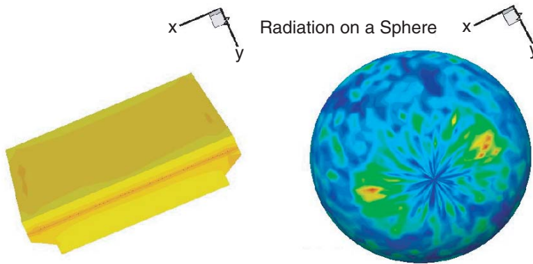
Figure 69 (Left) LED internal optical intensity and (right) normalized radiation intensity projected on a sphere of 3D LED simulation
