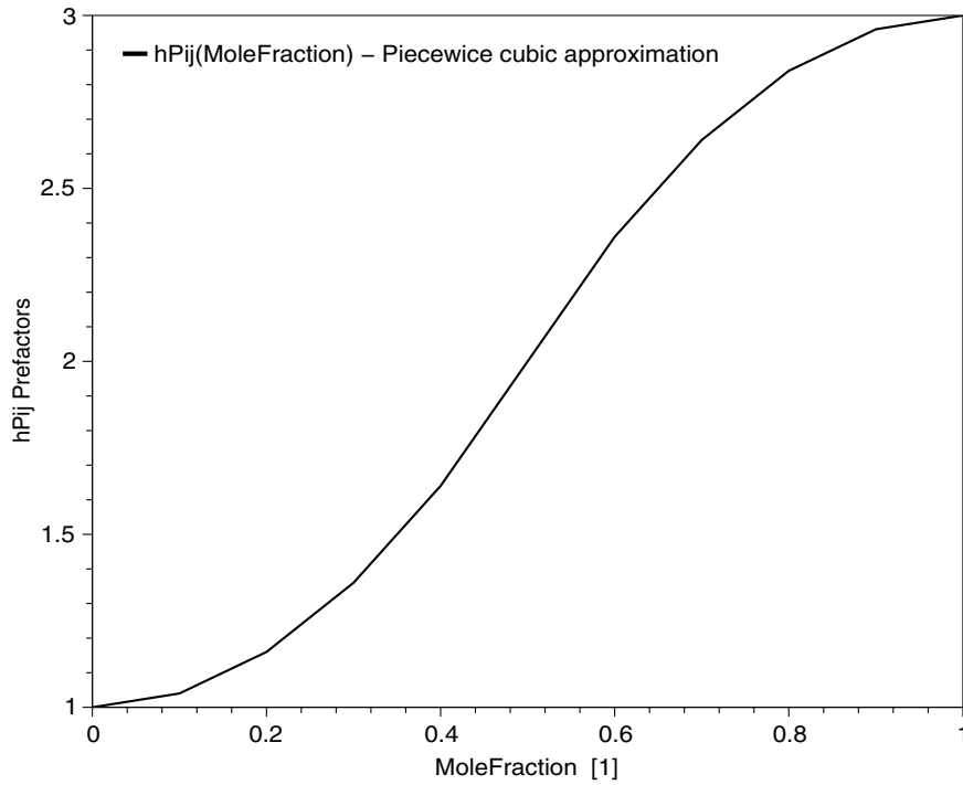
Figure 57 Example of piecewise cubic approximation
