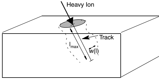
Figure 47 A heavy ion penetrating a semiconductor; its track is defined by a length and the transverse spatial influence is assumed to be symmetric about the track axis
