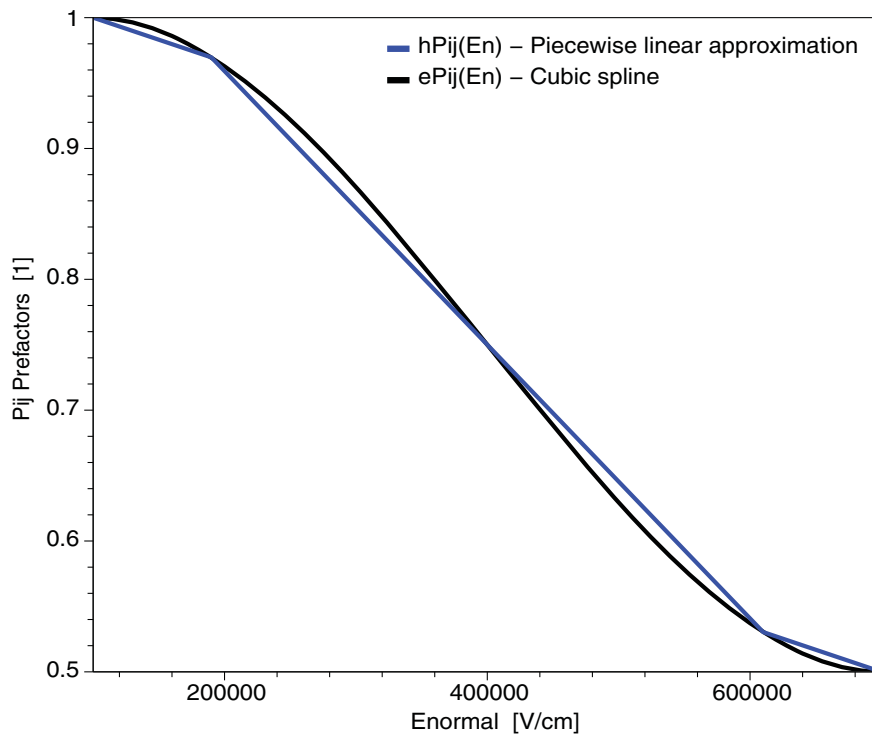
Figure 56 Example of cubic spline and piecewise linear approximation of piezo prefactors
