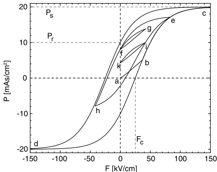
Figure 52 Example polarization curve
