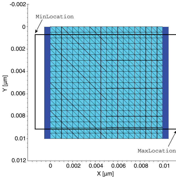
Figure 72 Defining the KMC simulation space in a Sentaurus Device structure
