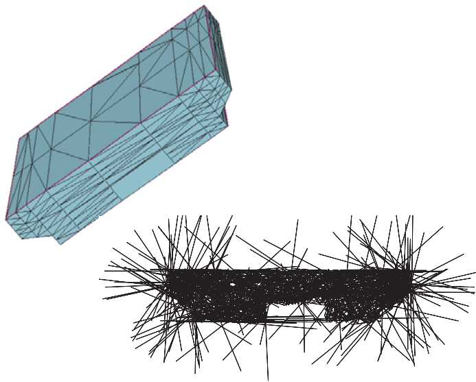
Figure 34 Applying the reflecting boundary condition in a 3D LED simulation; the boundary is drawn as a hollow rectangular waveguide inside the device
