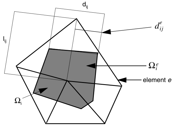
Figure 80 Single box for a triangular mesh in two dimensions
