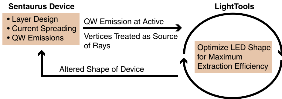
Figure 66 LED design flow to optimize extraction efficiency by LightTools and coupled to Sentaurus Device LED device simulation
