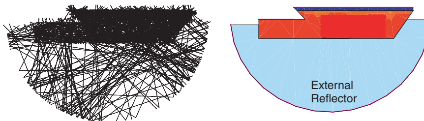
Figure 62 Using the reflecting boundary condition to define a reflector for LED raytracing
