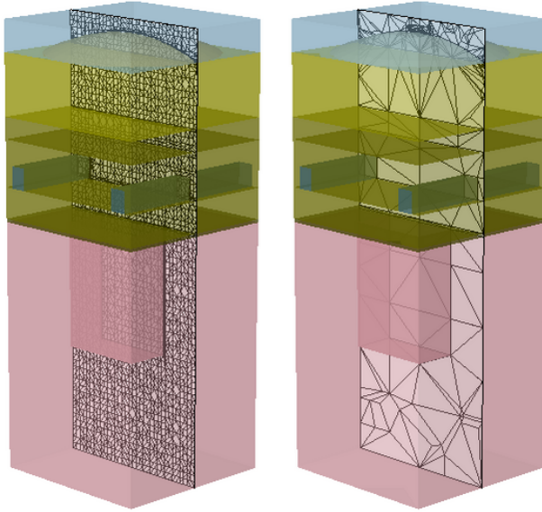
Figure 37 Comparison of two grids used in a 3D dual-grid CMOS image sensor simulation; the figures show cuts through the device center; ( left ) the electronic equations are solved on a fine grid and ( right ) a coarse grid is used for raytracing
