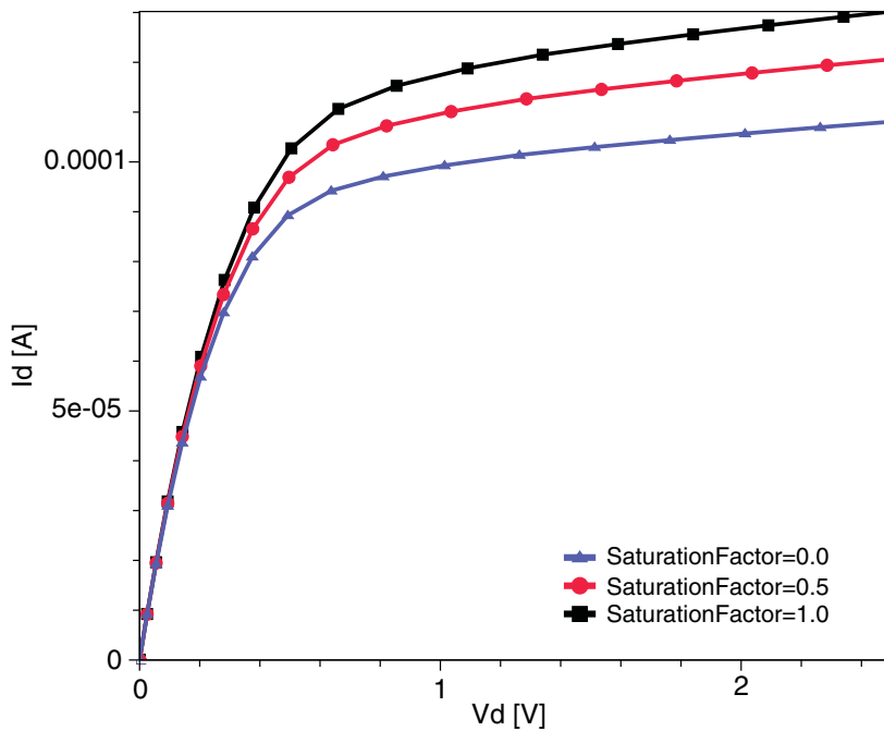
Figure 59 Dependency of I_d - V_d curves on SaturationFactor, with V_g = 1.5 V, and Stress = (0.6e9, 0, 0, 0, 0, 0)
