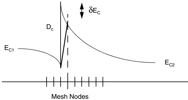
Figure 5 Band edge at a heterointerface with and without double points
