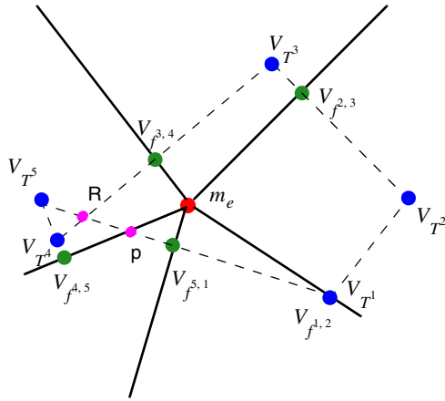
Figure 83 Element 5 is a non-Delaunay element; the face of the Voronoï box is a polygon (V_{T^1}, V_{T^2}, V_{T^3}, R, V_{T^1}) , and vertex R is not a Voronoï element center
