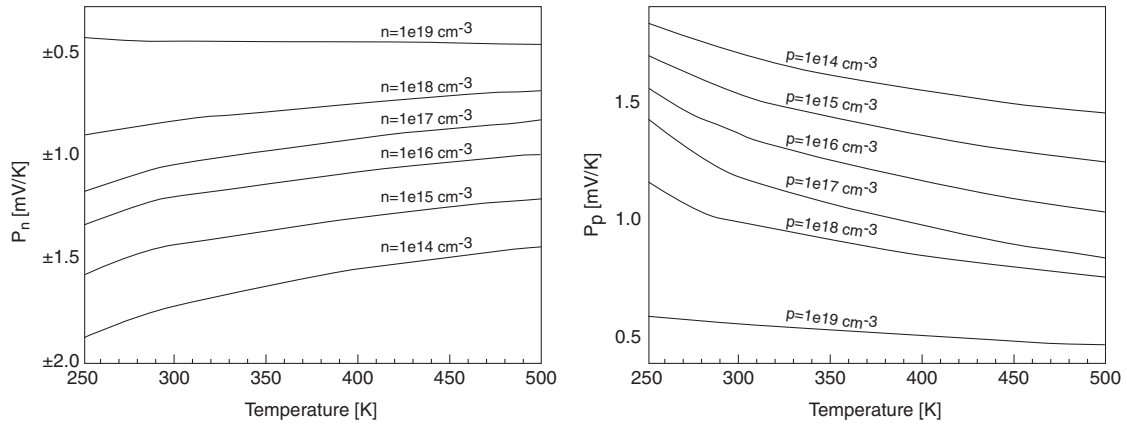
Figure 60 Thermoelectric powers ( left ) P_n and ( right ) P_p as a function of temperature and carrier concentration
