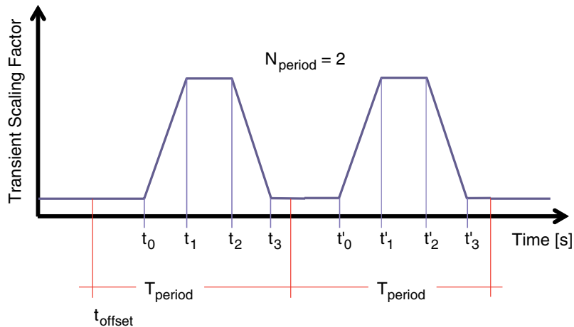
Figure 27 Extension of a predefined time dependency to a periodic signal where T_{\text{period}} , N_{\text{period}} , and t_{\text{offset}} correspond to WaveTPeriod , WavePeriods , and WaveTPeriodOffset
