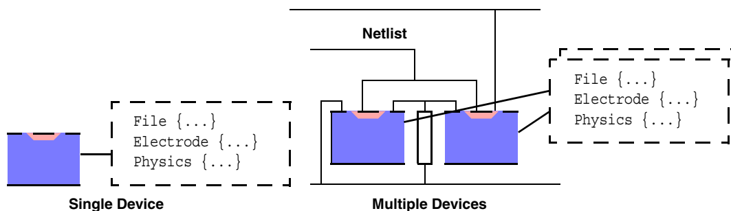
Figure 7 Each device in a multidevice simulation is connected with a circuit netlist
