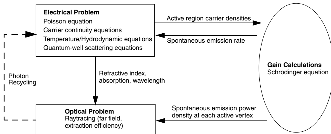
Figure 61 Flowchart of the coupling between electronics and optics for an LED simulation
