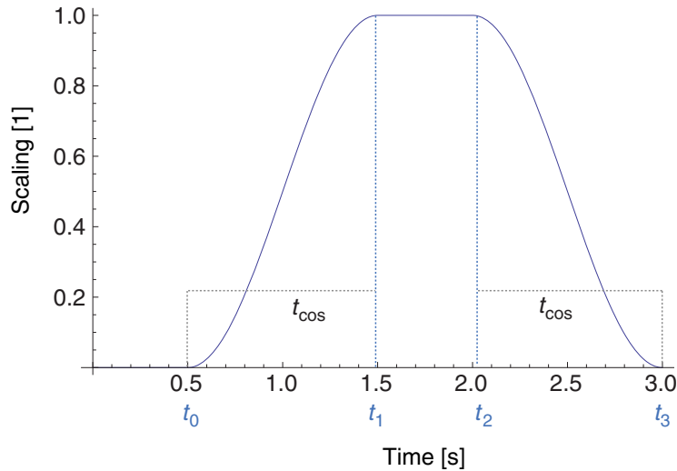
Figure 26 Rise and decay times based on a cosine function
