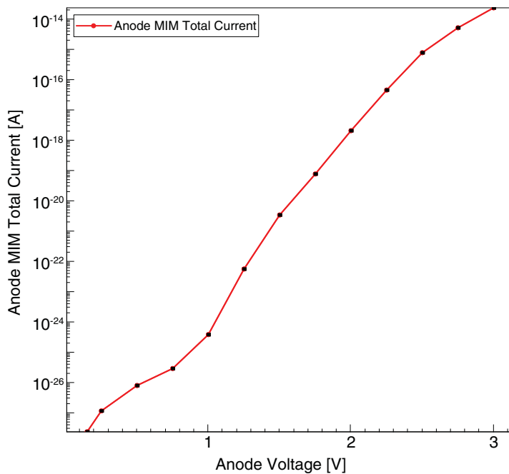
Figure 77 Approximate steady-state leakage current in a KMC-MIM simulation
