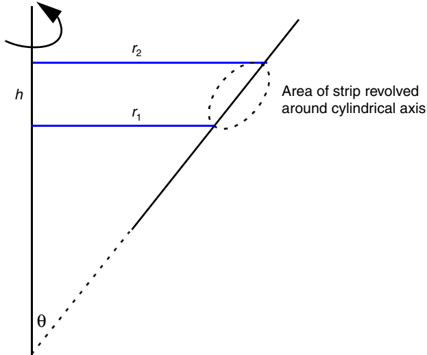
Figure 32 An illumination window subtended at an angle \theta from the cylindrical axis, forming a conical surface of revolution
