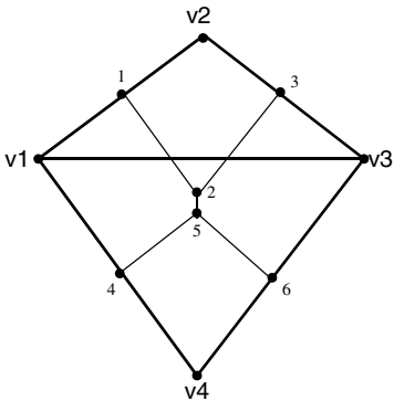
Figure 85 Total-volume conservation for Delaunay mesh
