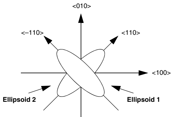
Figure 55 Sketch of Intel two-ellipsoid model; one ellipsoid is aligned along \langle 110 \rangle and the other along \langle -110 \rangle
