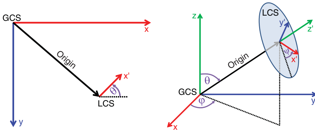
Figure 29 Coordinate system used in the illumination window for (left) two dimensions and (right) three dimensions
