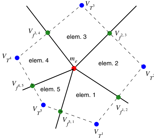
Figure 81 Face of the Voronoi box for Delaunay mesh without obtuse elements: view of mid-perpendicular plane at edge e with Voronoi element centers V_{T^i} and the Voronoi face center V_{f^{i,i+1}} between elements T^i and T^{i+1}
