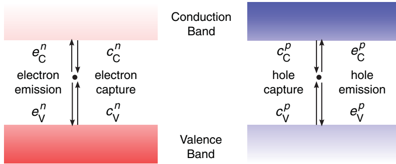
Figure 21 Trap occupation dynamics: (left) electron picture and (right) hole picture
