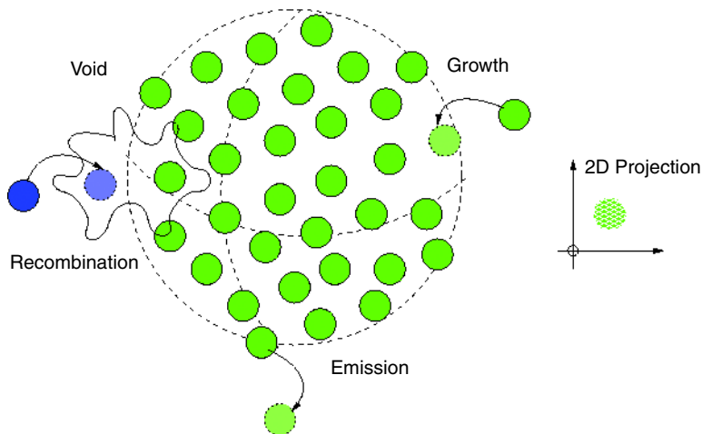
Figure 46 Voids are big cluster vacancies with a spherical shape that grow trapping neutral vacancies and shrink by recombination and vacancy emission
