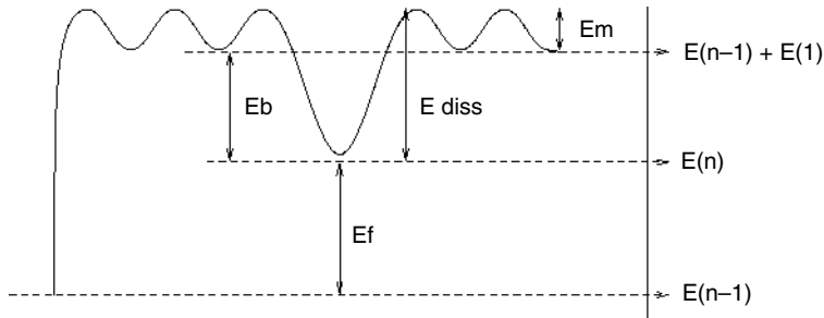
Figure 39 Energies involved in emission of an interstitial from an n -sized cluster
