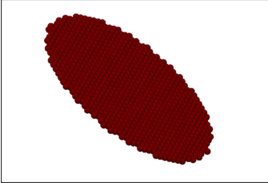
Figure 43 A dislocation loop taken from a Sentaurus Process KMC simulation
