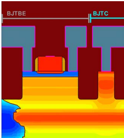
Figure 139 Two-dimensional TCAD simulation results using composite simulation domain consisting of the 2D domains BJTBE and BJTC
