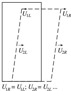
Figure 83 Periodic boundary condition
