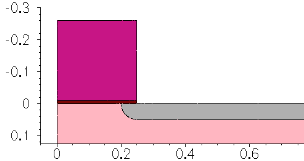
Figure 93 Single-material isotropic etching
