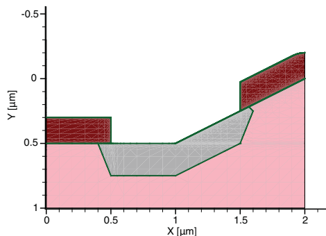
Figure 108 Basic trapezoidal etching example where the surface is nonplanar
