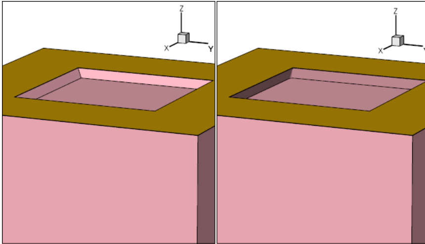
Figure 111 Three-dimensional trapezoidal etching: ( left ) angle=45 thickness=0.3 and ( right ) angle=110 thickness=0.44
