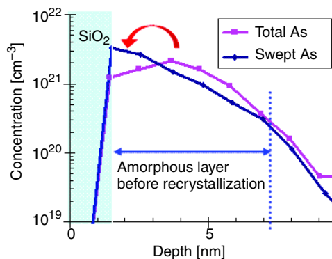
Figure 53 Impurity sweep example showing that arsenic has been pushed through the surface during recrystallization or SPER
