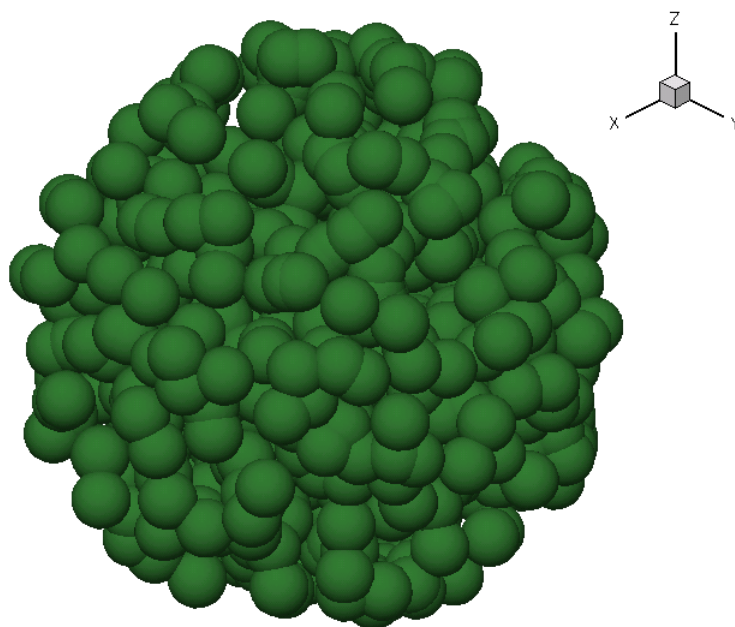
Figure 45 Voids are simulated with a spherical shape; this one contains 654 vacancies
