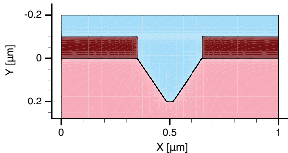
Figure 114 Piecewise linear etching
