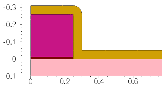
Figure 115 Isotropic deposition
