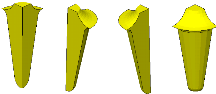
Figure 124 STI concave corner-shaped polyhedra in different directions: (from left to right) left back, right back, left front, and right front
