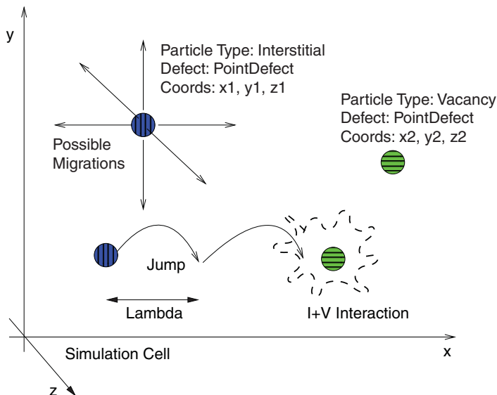
Figure 33 Point defects diffuse by jumping a distance \lambda in any orthogonal direction and can interact with neighbor particles
