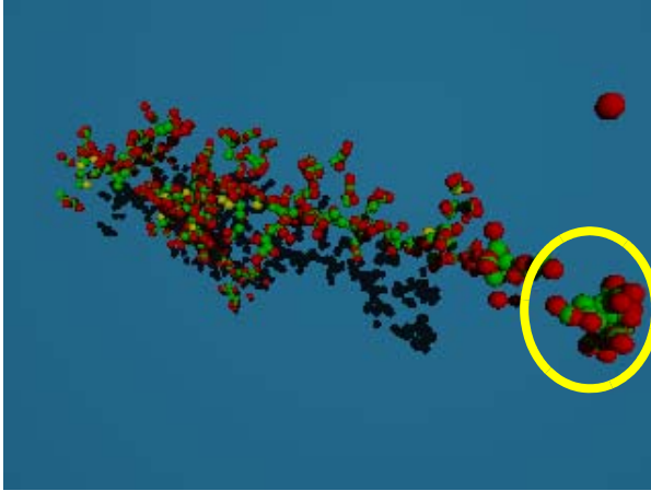
Figure 38 APs formed in Senterius Process KMC after some implanted as cascades: interstitials are red, vacancies are green, arsenic is yellow
