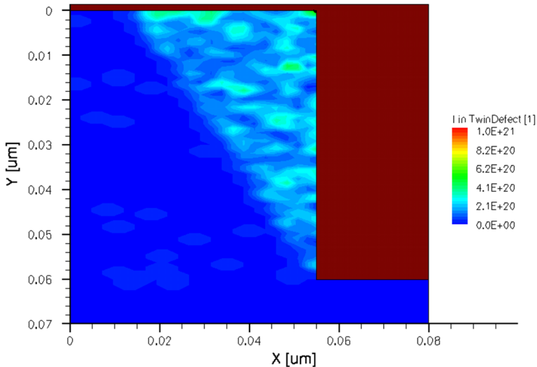
Figure 52 Concentration of twin defects representing defective silicon formation when SPER is in an amorphous region close to SiO 2 (silicon is blue, SiO 2 is brown)
