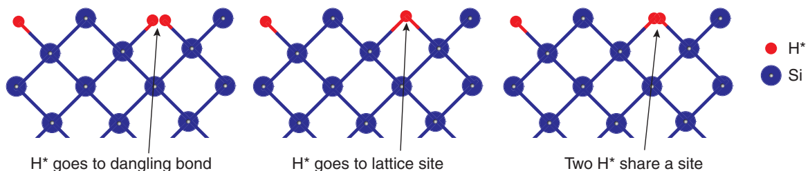
Figure 74 Illustration of how the shared occupancy model mimics dangling bonds and is a more physically correct approach than a model without shared occupancy: ( left ) the physical situation when H* occupies a dangling bond; ( middle ) in the Coordinates.Reactions model without shared occupancy, H* consumes both dangling bonds; and ( right ) shared occupancy allows two H* to share the same lattice site, mimicking two dangling bonds
