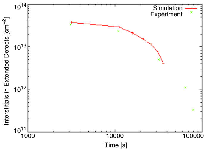
Figure 71 Dissolution of {311} extended defects at 670°C after a silicon into silicon implantation of 40 keV, 5 \times 10^{13} \text{ cm}^{-2}
