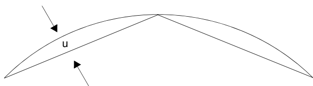
Figure 132 The curved surface represents the extracted new boundary and the piecewise linear segments represent the simplified boundary incorporated into the simulation mesh; the accuracy argument ensures that u \leq \text{accuracy}
