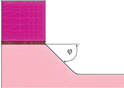
Figure 105 Fourier etching with etch wall angle of 45^\circ
