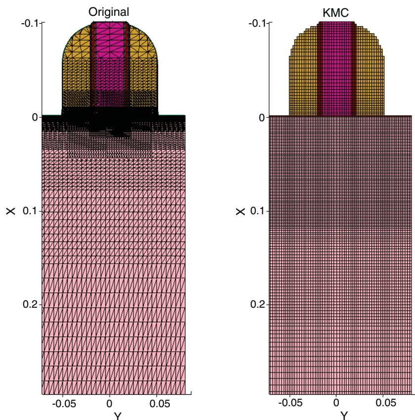
Figure 31 Interface between materials has a Manhattan structure in Sentaurus Process KMC; each element is assigned to a material and elements are always rectangular
