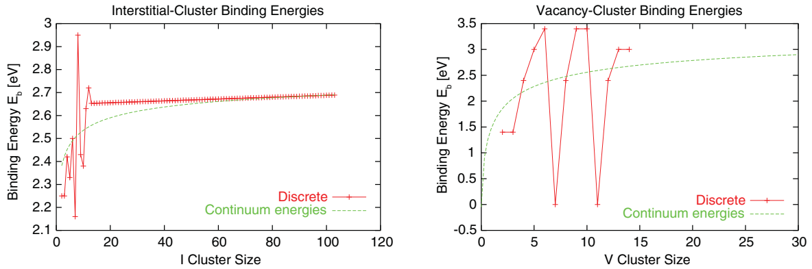
Figure 40 (Left) Interstitial-cluster binding energies and (right) vacancy-cluster binding energies; discrete values are assigned in the parameter database and the continuum energies are computed using Eq. 703
