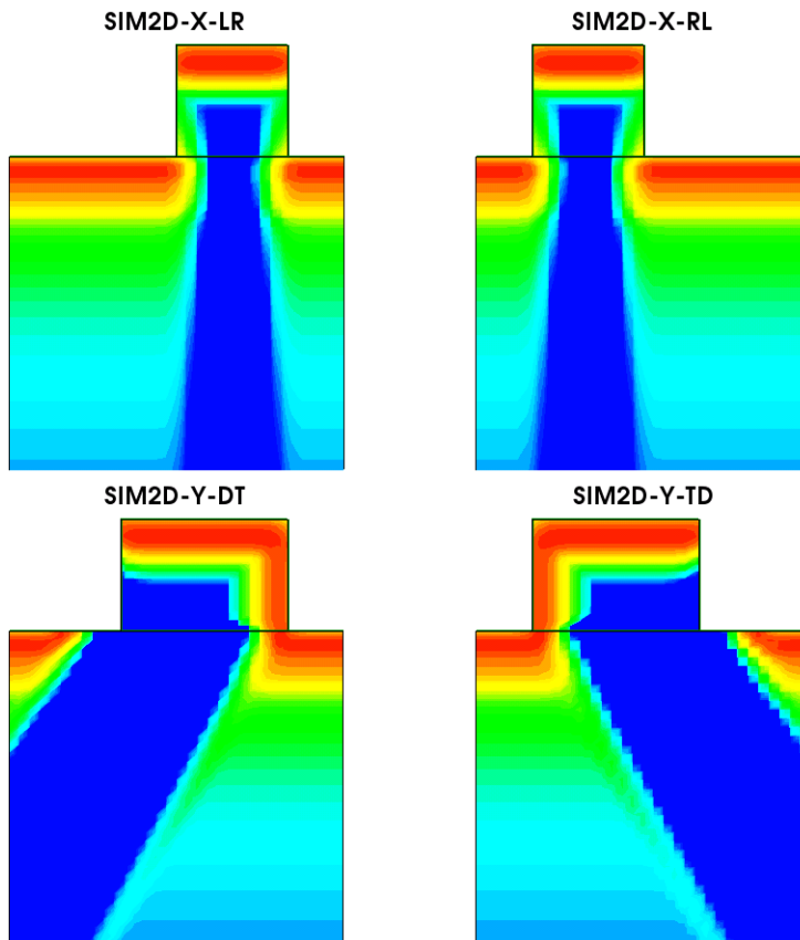
Figure 155 Two-dimensional implanted profile for selected slice angles as mentioned in Table 98
