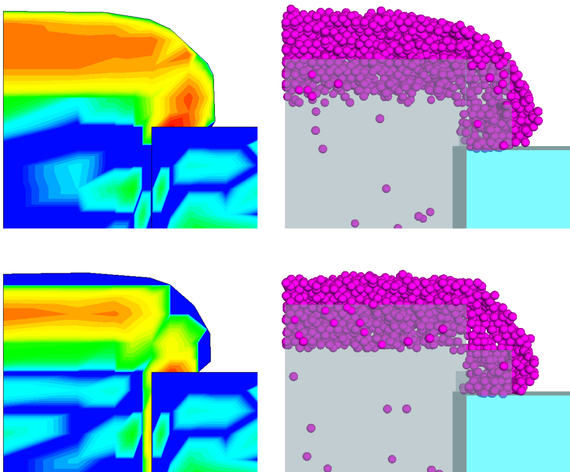
Figure 27 Impact of atomistic interfaces on a high-concentration P-epi step: ( left column ) plots show KMC doping concentration on the continuum finite-element structure and ( right column ) plots show phosphorus atoms. Top-row plots were created with Atomistic.Interfaces switched on, and bottom-row plots were created with Atomistic.Interfaces switched off. The upper-left plot has nonzero phosphorus along the outer surface, and the lower-left plot shows areas with zero concentration in many places along the outer surface.
