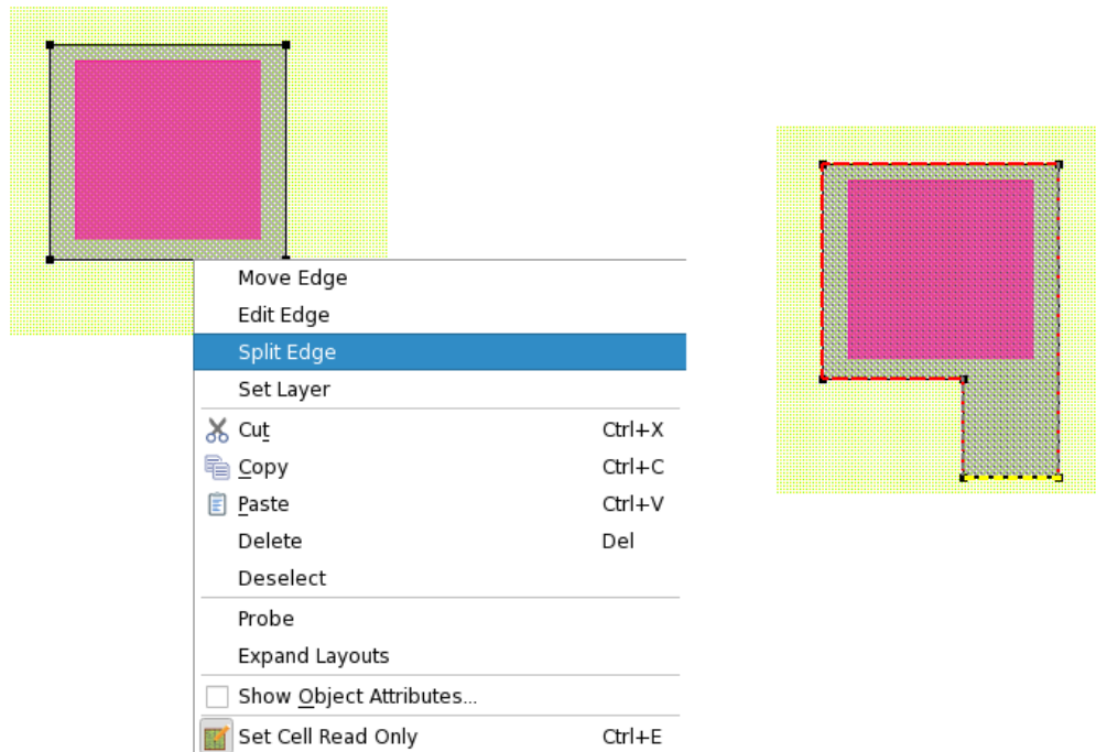
Figure 146 Procedure for converting a rectangle to a polygon
