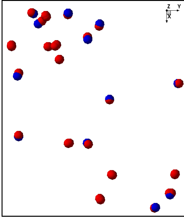
Figure 54 Bl_2 impurity clusters created using Sentaurus Process KMC; blue is boron and red is interstitial
