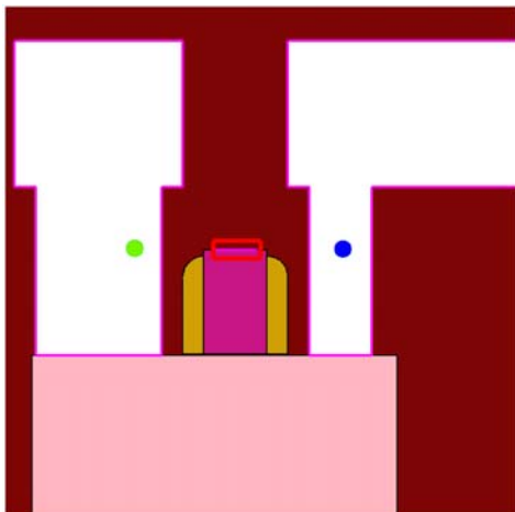
Figure 152 Final boundary after TCAD simulation showing gate (red), drain (blue), and source (green)
