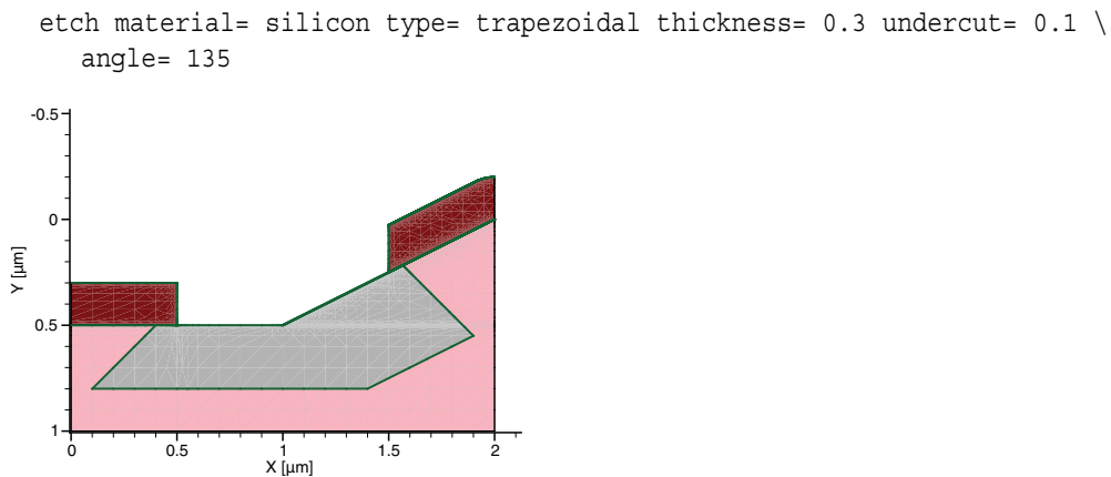
Figure 110 Trapezoidal etching example generating a wide trench bottom
