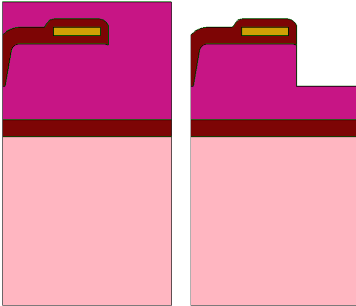
Figure 97 Two-dimensional anisotropic etching with material providing protection: (left) original structure and (right) result after etching
