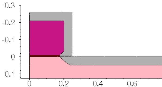
Figure 94 Multimaterial isotropic etching
