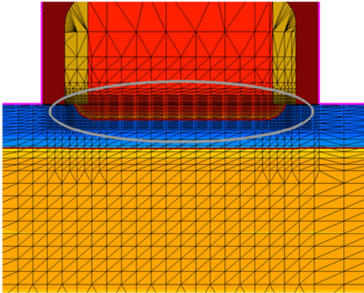
Figure 149 Example of meshing in the emitter region of a BJT with extend = 0.1 μm
