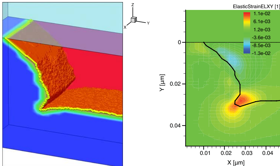
Figure 50 Recrystallization of a rectangular-shaped amorphous region using the LKMC model
