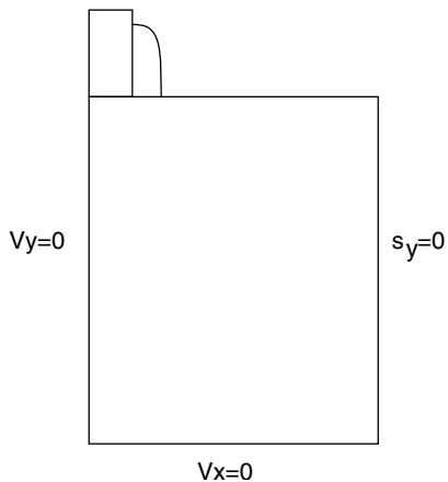
Figure 82 HomNeumann boundary condition on right boundary plane
