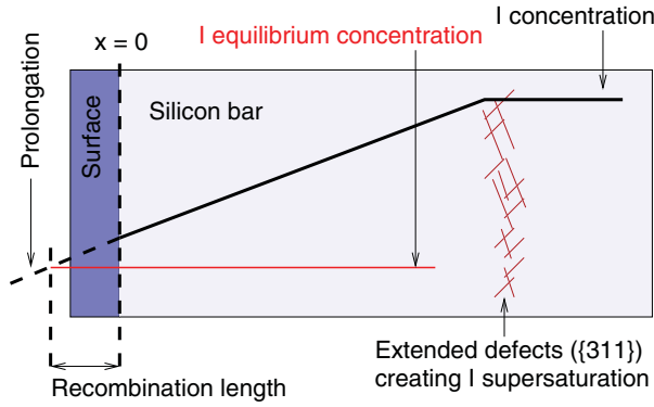
Figure 63 Recombination length is the distance between the interface and the point in which the prolongation of the point-defect concentration joins its equilibrium concentration
