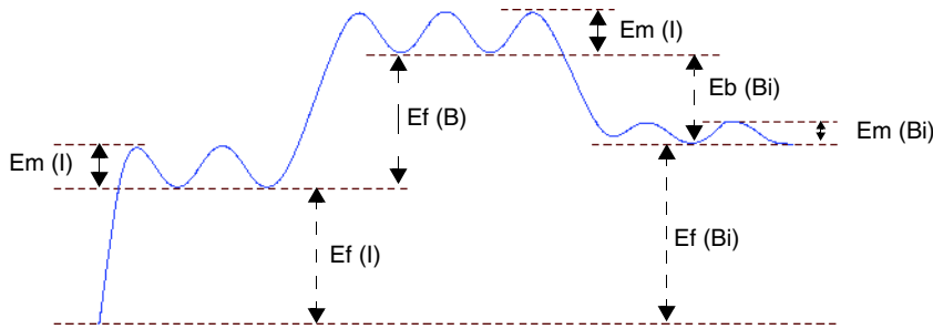
Figure 35 Energies involved in the kick-out mechanism for B^- + I^0 = Bi^- . Migration energy of the interstitials and boron–interstitial are specified in the parameter database as Em. The binding energies are Eb, and the I formation energy is specified as Eform. The formation energy for dopants in pure silicon is assumed to be 0 because the dopants are already in the simulation; the dopants are not created by the system.
