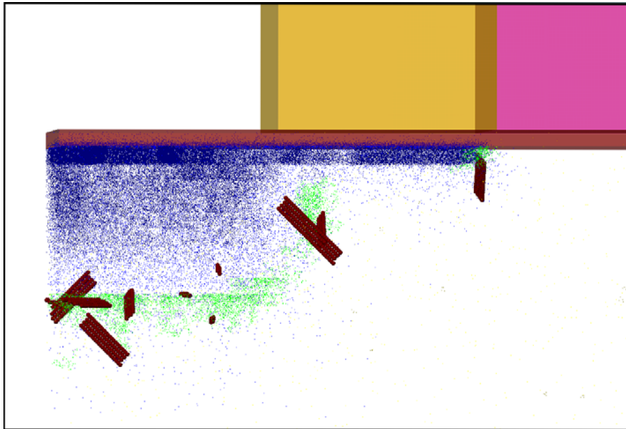
Figure 41 {311} defects are simulated as parallel stripes (rows) of I particles lying in a {311} plane: red is silicon interstitials in {311}; green is I and V in APs; and blue is arsenic
