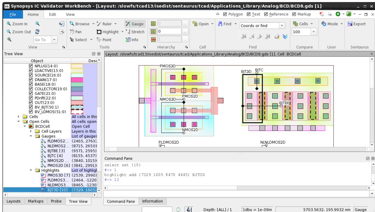
Figure 137 Adding Sentaurus markups to a layout
