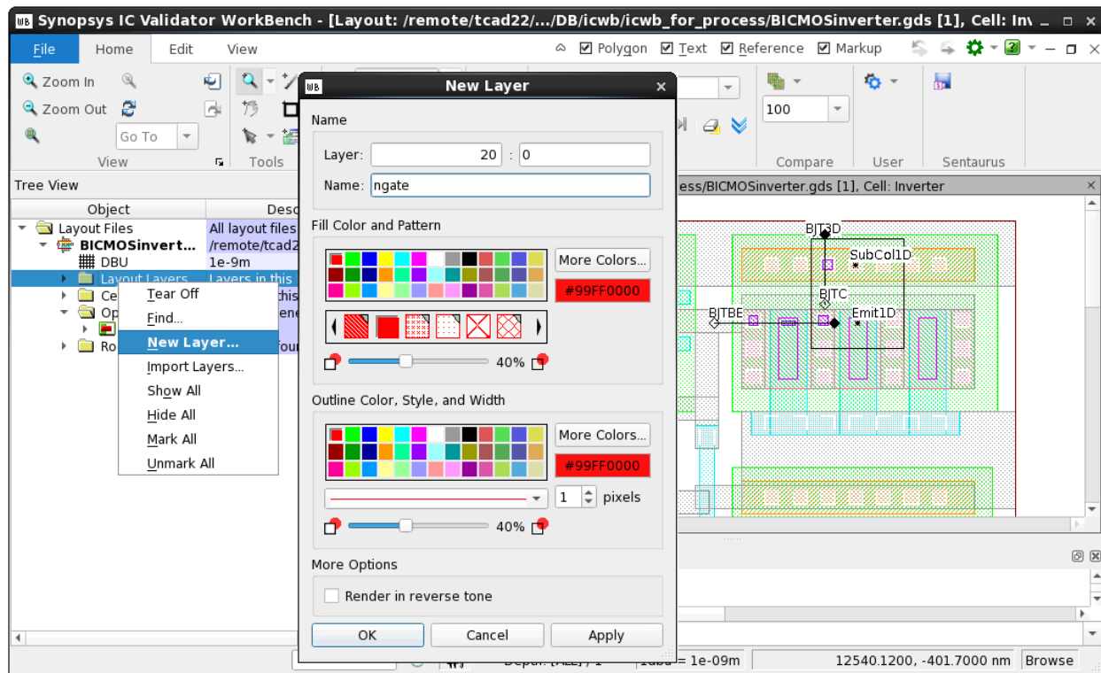
Figure 144 Defining a layer and its attributes: choosing New Layer and specifying the attributes of the layer
