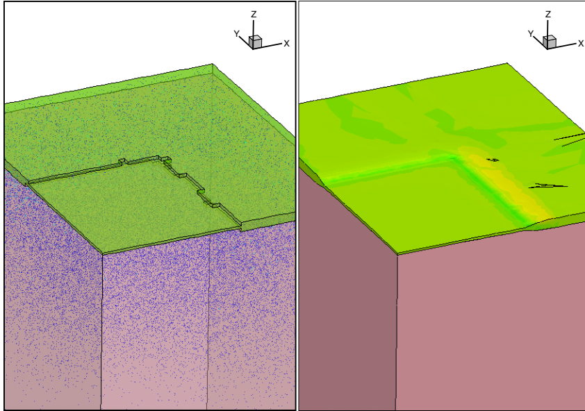
Figure 65 Example of Sentaurus Process KMC coupled with an oxidation in three dimensions: ( left ) KMC simulation in which the internal mesh is coupled to ( right ) continuum oxidation simulation
