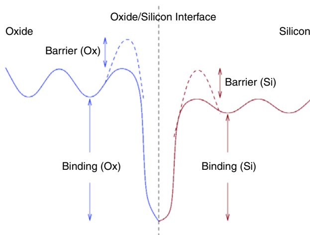
Figure 64 Dopants reaching the interface might be trapped there with a different binding energy for each interface side; energy barriers for capture and emission also can be present
