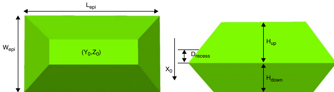
Figure 130 Parameters for generating epitaxial diamond-shaped polyhedron
