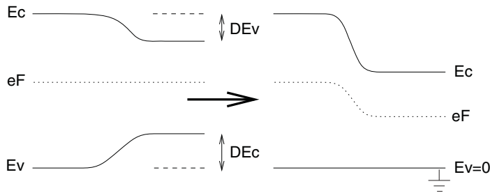
Figure 61 Bandgap narrowing; Sentaurus Process KMC assumes the valence band has zero energy
