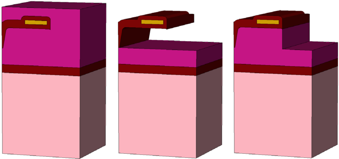
Figure 98 Three-dimensional anisotropic etching with material providing protection: (left) original structure, (middle) default behavior leaving a floating region, and (right) behavior with aniso.etching.protect.materials option
