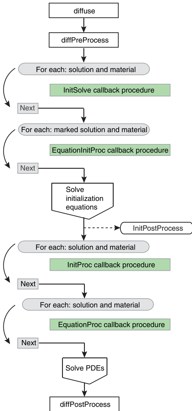
Figure 76 Flowchart with calls to callback procedures during execution of a diffuse command
