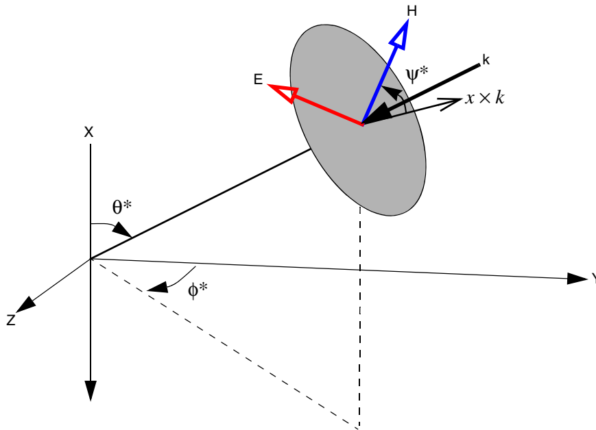
Figure 21 Definition of coordinate system for 3D plane wave excitation and examples of parameters of 3D plane wave: \theta^* , \phi^* , and \psi^* are the Incidence.Polar.Angle, Azimuthal.Angle, and Polarization.Angle, respectively
