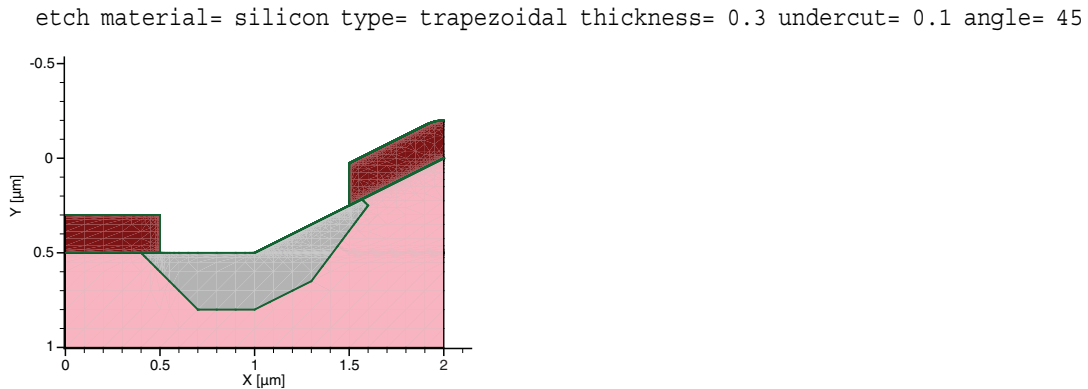
Figure 109 Trapezoidal etching example generating a narrow trench bottom
