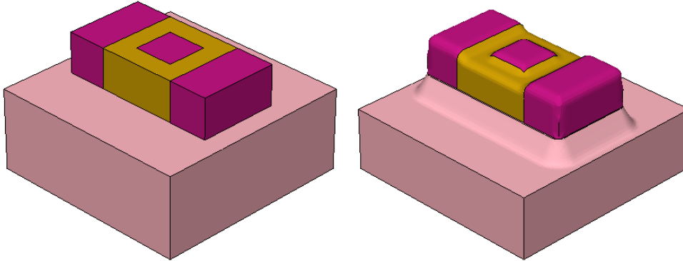
Figure 106 Three-dimensional multimaterial Fourier etching: ( left ) before etching and ( right ) after etching
