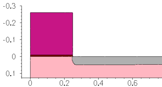
Figure 104 Fourier etching
