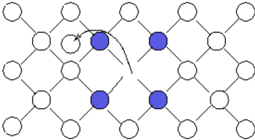
Figure 56 Example of FT mechanism: an As_4 cluster can emit an interstitial to become an As_4V impurity cluster: blue is arsenic and white is silicon
