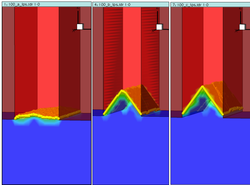
Figure 49 SPER evolution (blue is crystalline silicon; red is amorphous one) with time ( left to right ) 2, 4, and 6 minutes at 550°C of a thin (20 nm) silicon fin. The oxide (brown material) does not provide the correct template for the lattice atoms to form undistorted bonds, stopping the recrystallization and leading the way to the (111) planes. When the two (111) planes are formed, no further fast (100) SPER is possible, and the SPER occurs through the very slow and defect-prone (111) recrystallization.
