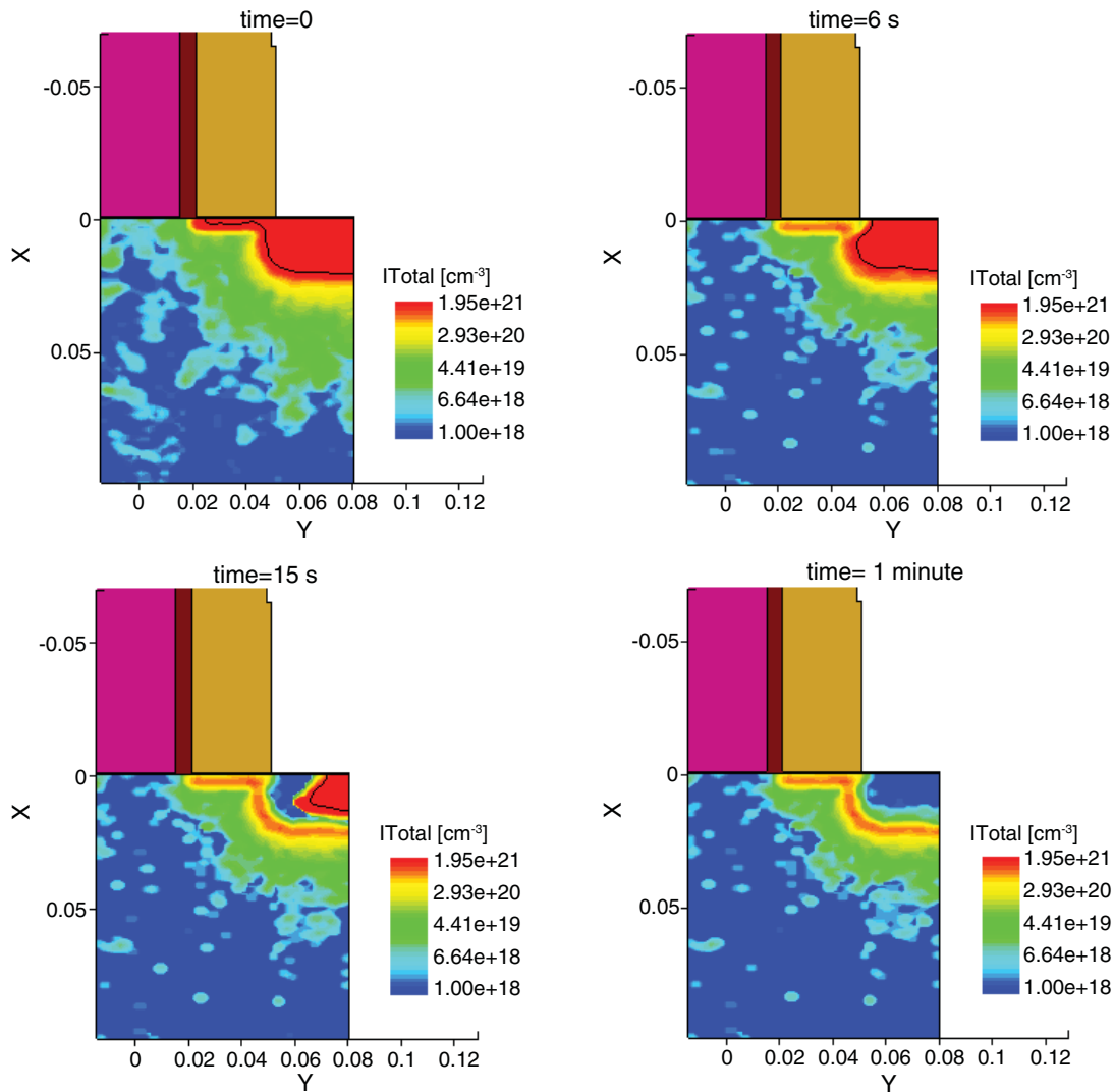
Figure 48 Source and gate of a transistor during SPER as simulated by Sentaurus Process KMC. The total concentration of interstitials is represented during the evolution of the recrystallization front. At the end, there is damage only near the initial amorphous/crystalline interface. The remaining damage can form end-of-range (EOR) defects.
