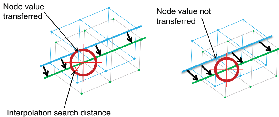
Figure 91 (Left) The new mesh (blue) has moved from its previous position, but the distance is smaller than Interpolation.Search.Dist, so values are interpolated from the green mesh to the blue mesh at the boundary. (Right) The distance is too large, so only those points in the blue mesh that are the same material as the green mesh are interpolated.
