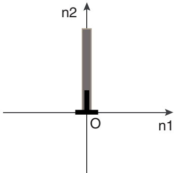
Figure 85 Edge dislocation located at the origin O; n1 is the Burgers vector and n2 is the direction of the half plane
