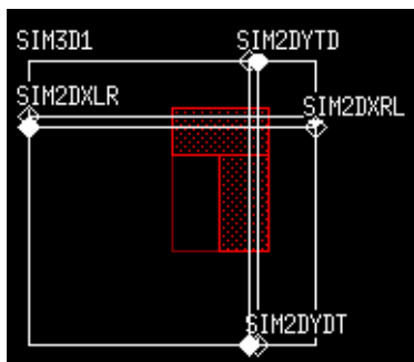
Figure 153 Structure layout where implantation is performed at highlighted L-shaped red region
