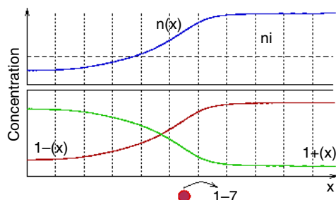
Figure 59 A mobile particle ( I^- ) sees different electronic properties when jumping from one element to a different one. Its charge state must be updated to reproduce the expected macroscopic concentration.
