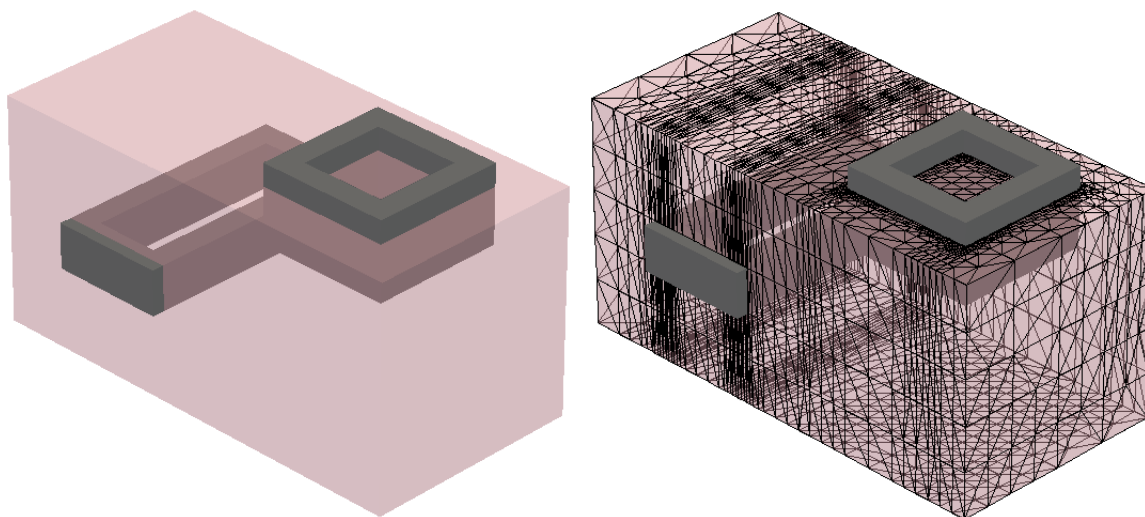
Figure 90 (Left) Three-dimensional structure with two refinement boxes and (right) corresponding mesh
