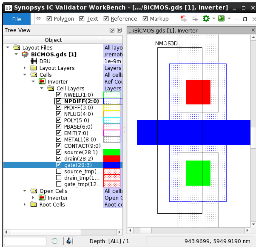
Figure 151 Auxiliary layers added for drain, gate, and source contacts are represented by rectangles of solid color in the layout
