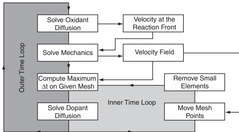
Figure 79 Flowchart for simulation of material growth
