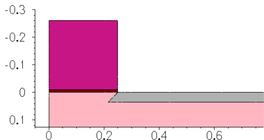
Figure 101 Directional etching with undercut
