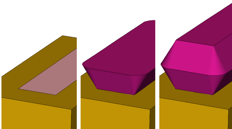
Figure 120 Trapezoidal deposition: ( left ) before deposition, ( middle ) first deposition step with angle=120, and ( right ) second deposition step with angle=60
