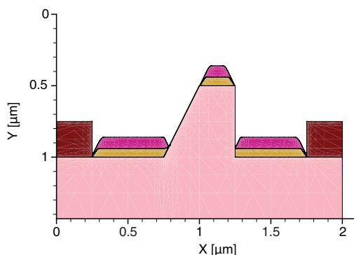
Figure 119 Two-dimensional Fourier deposition for demonstration purposes, nitride is deposited selectively on silicon using Fourier deposition and, then, an additional Fourier deposition step adding polysilicon selectively on nitride is performed
