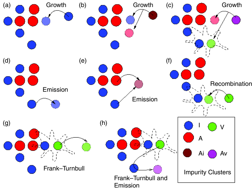
Figure 55 Impurity clusters are disordered agglomerations of dopants and silicon point defects that trap and emit particles; Frank–Turnbull mechanisms and IV recombinations also are possible (light colors represent the reaction product, for example, light red and light blue in (b) represent the A atom and interstitial incorporation after Ai splits into A and I)
