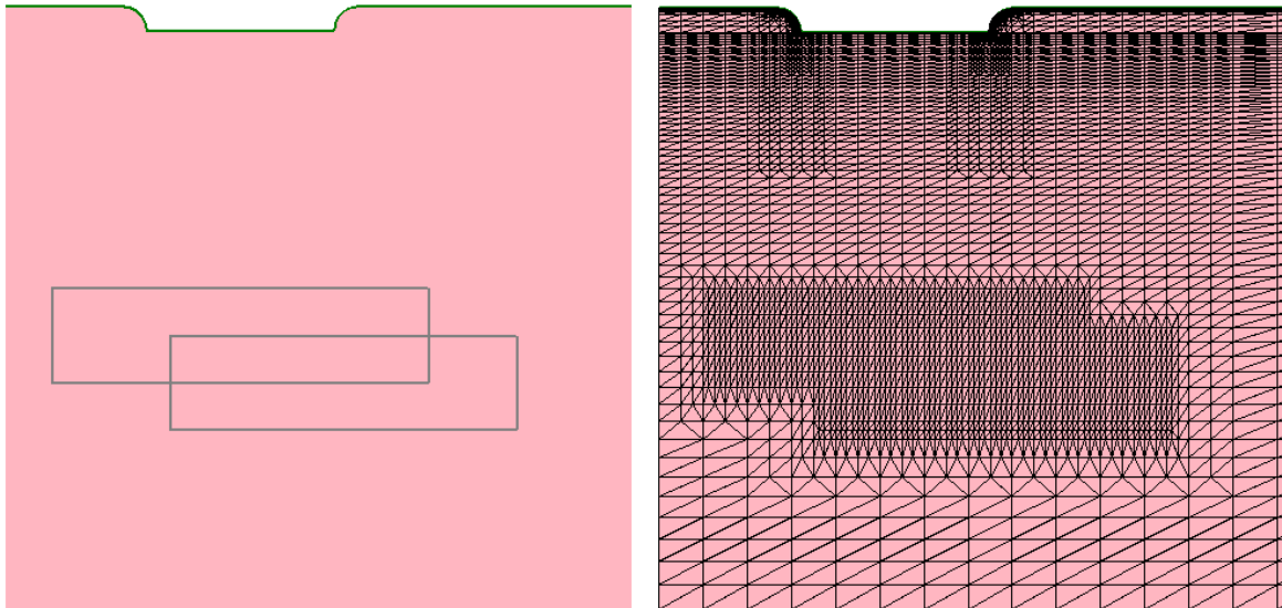
Figure 89 (Left) Two-dimensional structure with two refinement boxes and (right) corresponding mesh
