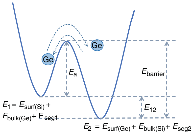
Figure 73 Energy diagram for surface segregation reaction in SiGe
