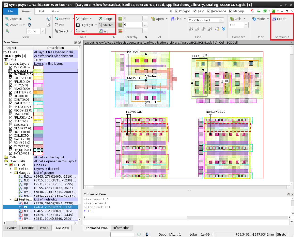
Figure 135 ICVWB main window with toolbar buttons specific to TCAD Sentaurus indicated by red boxes
