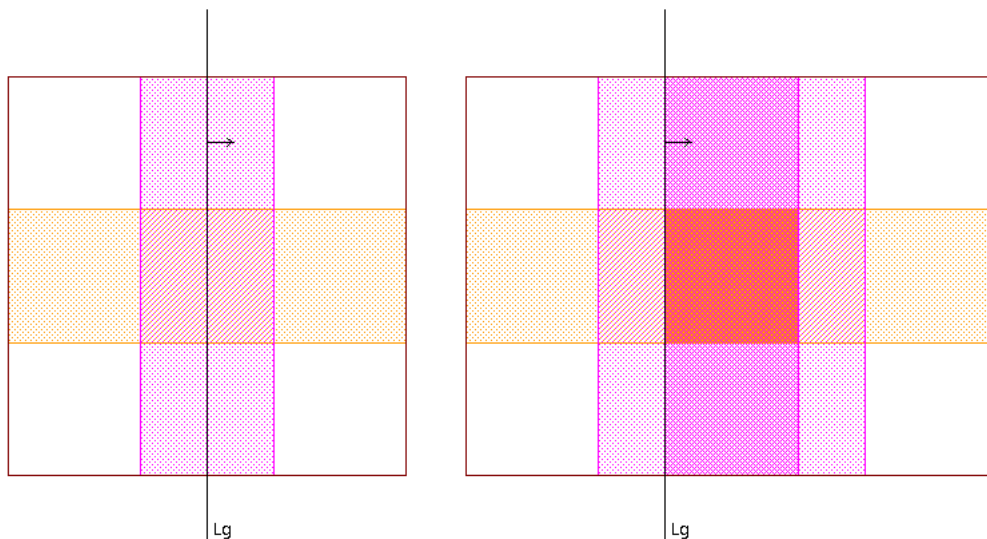
Figure 140 (Left) Snapshot of sample ICVWB layout with stretch line and (right) effective layout seen by Sentaurus Process when the layout is loaded with a positive stretch amount
