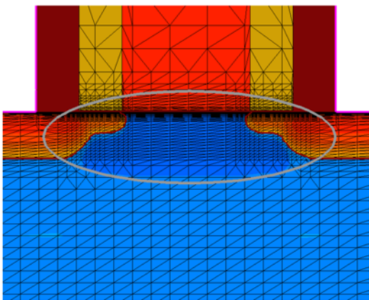
Figure 150 Example of meshing in channel region of an NMOS device with extend = 0.1 μm
