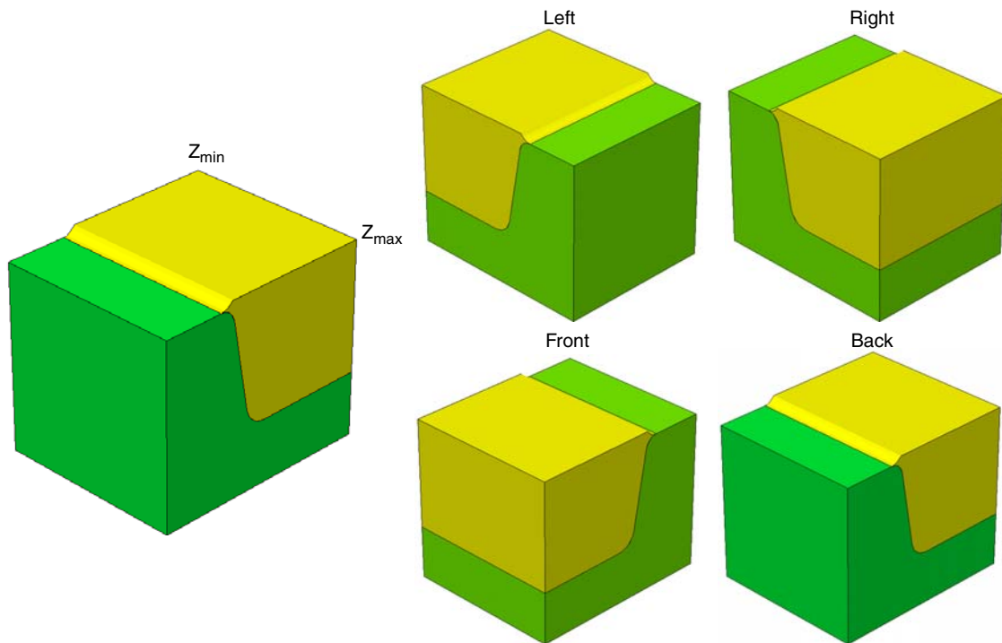
Figure 122 STI-shaped polyhedra in different directions
