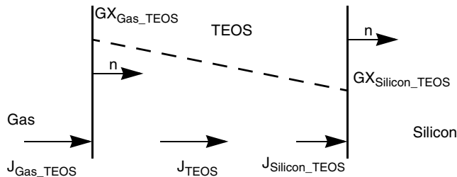
Figure 75 Flux, ambient concentration, and motion of growth front during growth process
