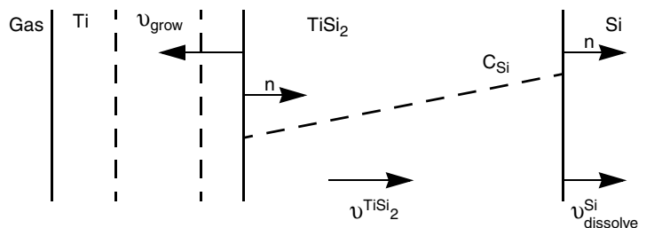
Figure 78 Velocities in 1D silicidation process
