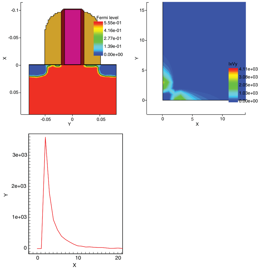
Figure 67 Visualization of a TDR file saved with the concentrations and histogram options: ( upper left ) 2D representation of Fermi level concentration, ( upper right ) 2D histogram of amorphous pockets and dopant clusters, and ( lower left ) histogram for clusters
