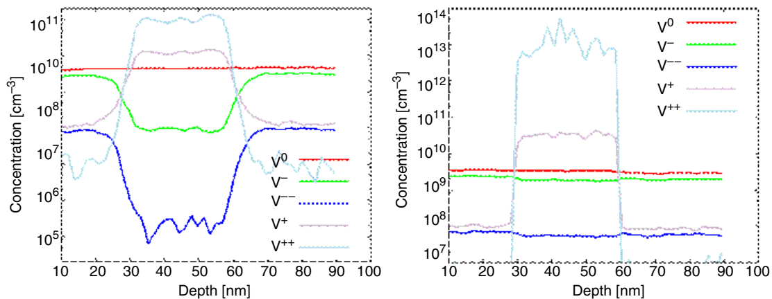
Figure 58 Simulated vacancy profiles for a p-sample (from 30 to 60 nm) for different vacancy charge states: ( left ) smoothing out the charge concentration and ( right ) incorrect results without smoothing
