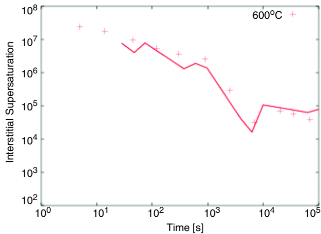
Figure 70 Supersaturation evolution with time, after a silicon implantation ( 2 \times 10^{13} dose, 40 keV energy) annealed 1 \times 10^5 s at 600°C. (Experimental points modified from [52] to use the same B diffusivity.) Points are experiments, lines are KMC.
