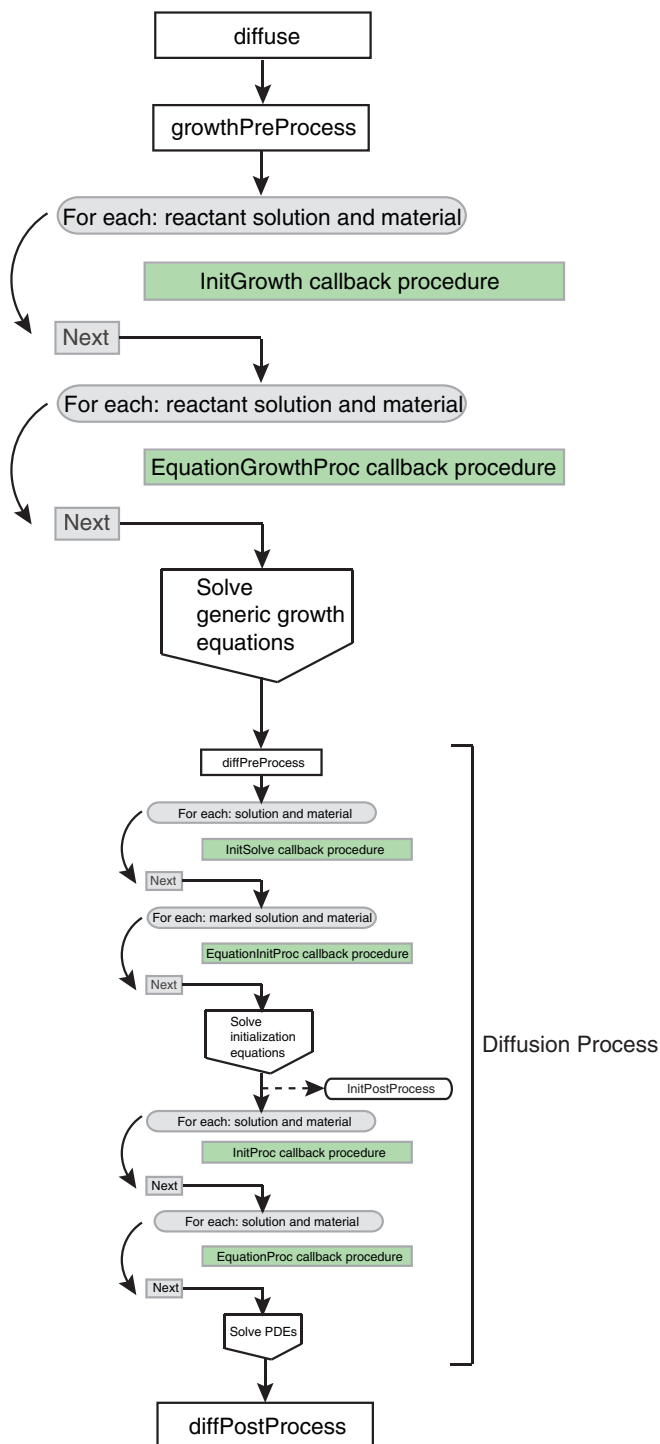
Figure 77 Flowchart with calls to callback procedures during execution of a diffuse command, including generic material growth
