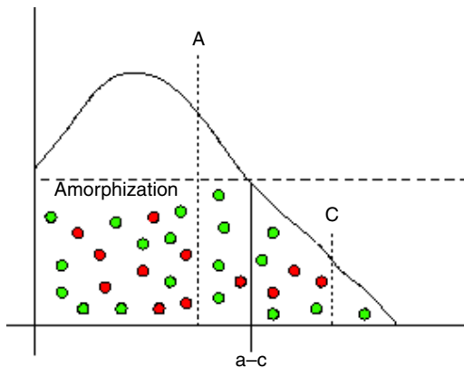
Figure 47 Damage concentration profile after an implantation
