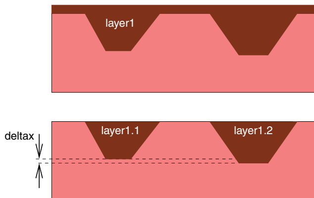
Figure 3 Illustration of region-naming rules
