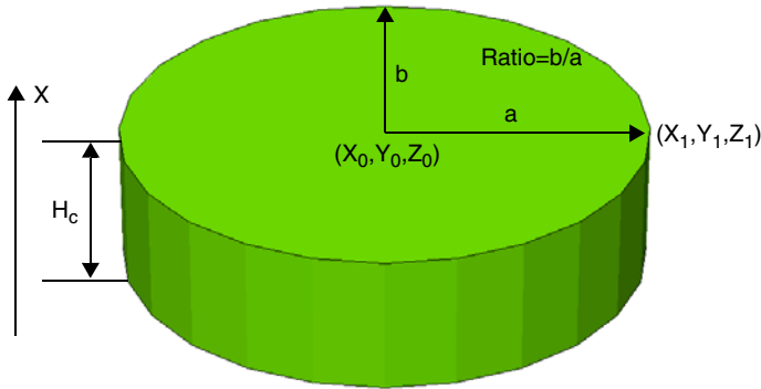
Figure 128 Elliptic cylinder-shaped polyhedron
