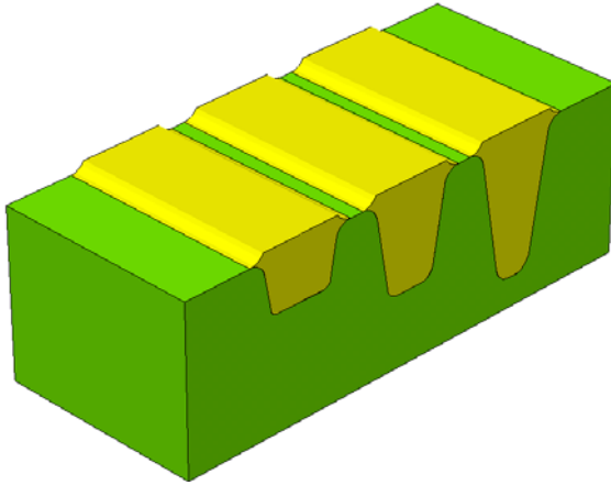
Figure 123 STI-shaped polyhedra with different T_{sti} and R_b
