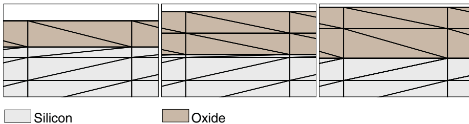
Figure 80 Meshing strategy during thermal oxidation
