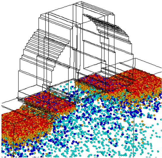
Figure 68 Visualization of individual defects of a 3D MOSFET device simulated by Sentaurus Process KMC
