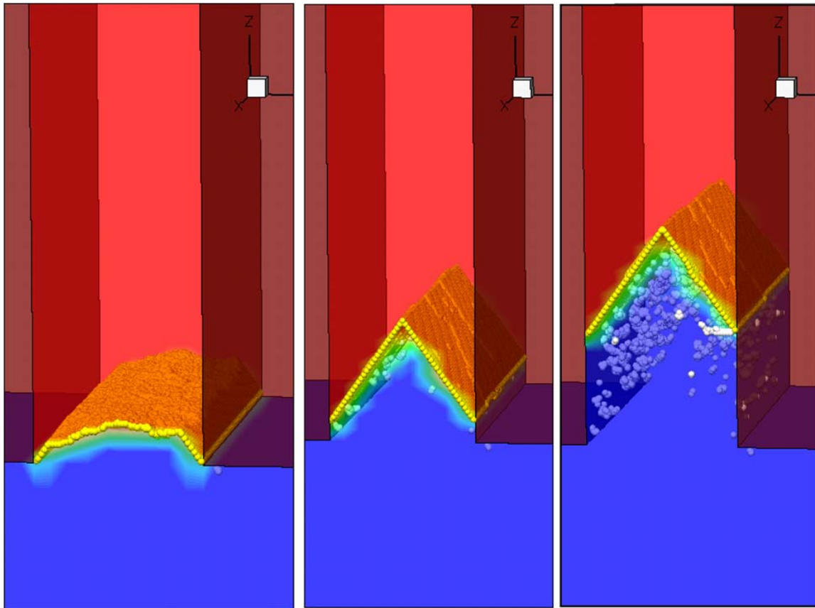
Figure 51 Evolution of a thin (20 nm width) amorphized silicon fin (amorphous is red, crystalline is blue) annealed at 600°C; arrow-shaped a/c interface is represented by yellow atoms and formation of defects (twins) is shown as white spheres
