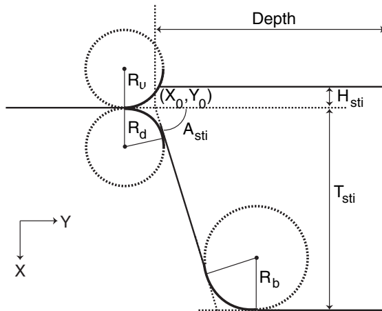
Figure 121 Parameters for generating STI-shaped polyhedron
