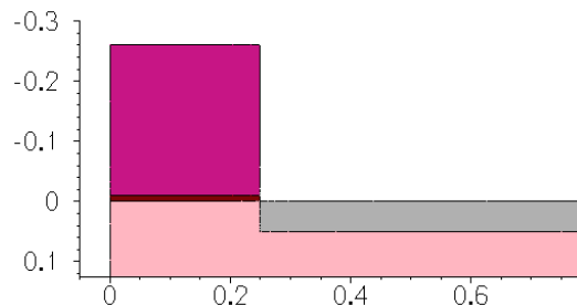
Figure 99 Anisotropic etching
