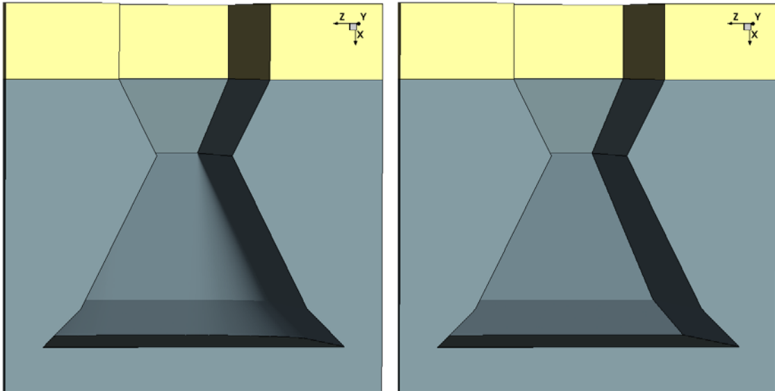
Figure 113 Trapezoidal etching produced using offset.steps= {{0.1 -0.05 -0.05} {0.2 0.1 0.1} {0.05 0.05 0.05}} and with (left) trapezoidal.algorithm=offset and (right) trapezoidal.algorithm=straight.skeleton
