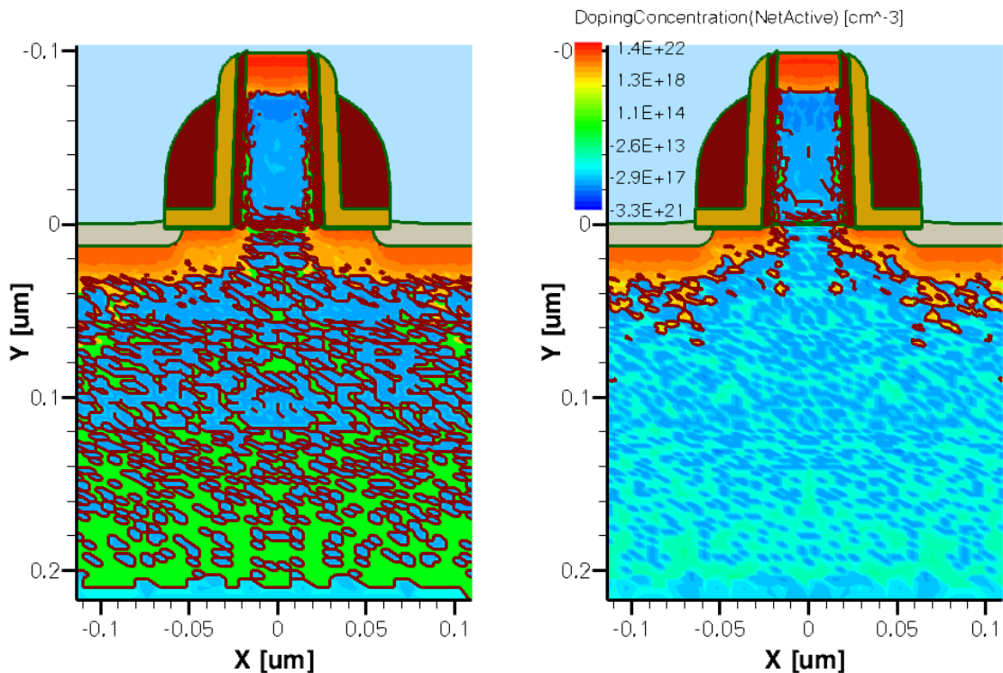
Figure 66 Comparison of NetActive concentration in simulations performed with (left) Smooth.Field set to 0 (disabled) and (right) Smooth.Field set to 1
