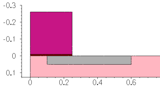
Figure 102 Polygonal etching
