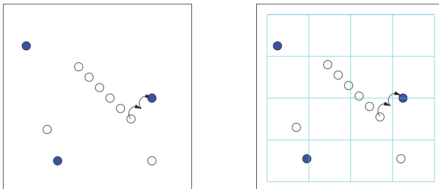
Figure 30 Sentaurus Process KMC divides ( left ) the space into ( right ) small rectangular elements; these elements are used for neighbor search, amorphization, and charge models
