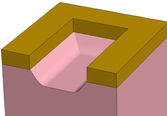
Figure 107 Crystallographic etching
