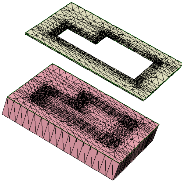
Figure 86 Mask edge-based refinement shown on the mask and in silicon
