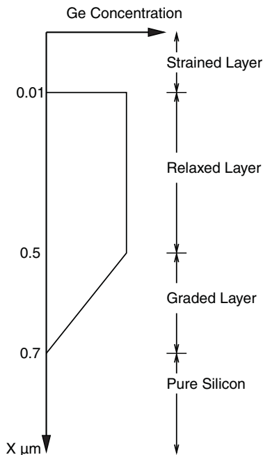
Figure 84 Simple SiGe wafer for customizing the lattice spacing
