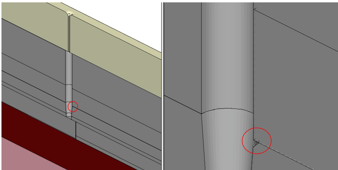
Figure 92 (Left) Example of artifact in geometry and (right) magnification of artifact (circled region)
