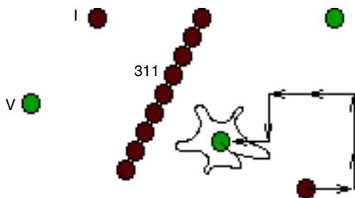
Figure 29 Nonlattice KMC method tracks only atoms in defects; lattice silicon atoms are excluded
