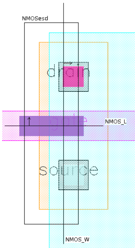
Figure 141 Adding stretch lines in a layout to vary gate width and gate length
