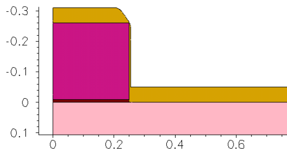
Figure 118 Crystallographic deposition: vertical direction is \langle 100 \rangle , lateral direction is \langle 011 \rangle
