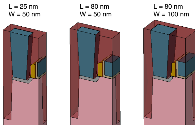
Figure 142 Effect of stretch on 3D NMOS structure showing variation in width and length
