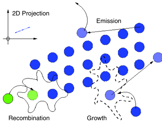
Figure 42 Recombination of defects in a {311} defect
