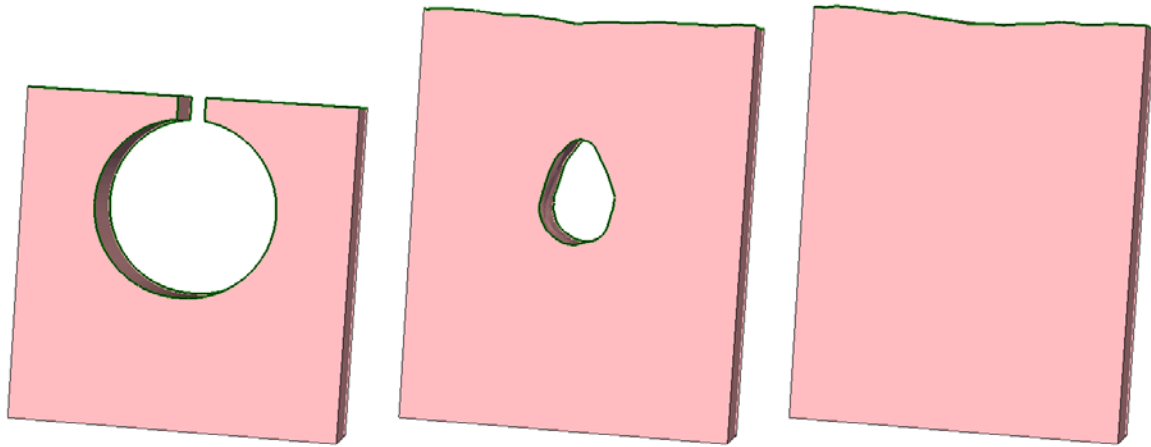
Figure 72 Simple example showing the effect of visibility: ( left ) the starting structure is a cavity with a small opening; ( middle ) during deposition with visibility switched on, growth occurs everywhere until the hole is filled, leaving a bubble; and ( right ) with visibility switched off, growth continues until no gas sites remain
