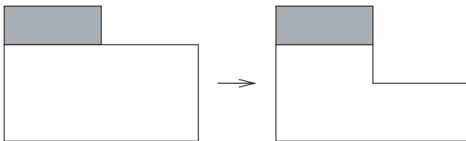
Figure 95 Anisotropic etching
