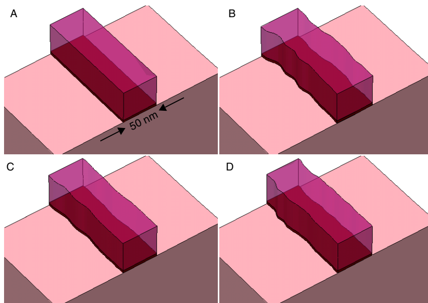
Figure 131 Example of 3D structure with LER applied using different values of standard deviation \delta and correlation length \lambda : (A) no LER applied, (B) LER applied with \delta = 4 nm and \lambda = 20 nm, (C) LER applied with \delta = 2 nm and \lambda = 20 nm, and (D) LER applied with \delta = 2 nm and \lambda = 12 nm
