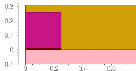
Figure 117 Fill deposition
