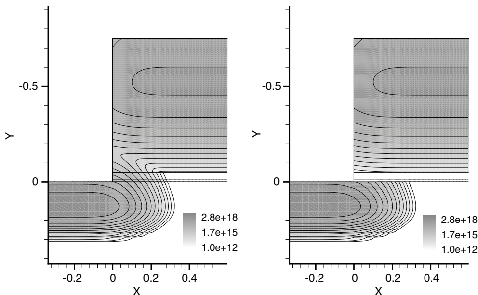
Figure 16 Boron implantation at a vertical mask edge ( left ) with backscattering and ( right ) without backscattering; tilt angle is 0° and energy is 35 keV
