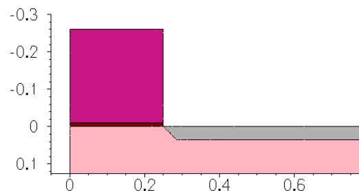
Figure 100 Directional etching (angled wall)
