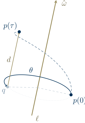
Figure 1: Chasles' theorem. Whatever path the body takes from p(0) to p(\tau) , the net displacement can always be reproduced in two steps about a single line \ell : rotate through \theta = \|\omega\|\tau about \ell (navy), carrying p(0) to q , then translate by d parallel to that same axis (gold). Because the slide is along the very axis of the turn, the two steps commute, and performing them together traces the dashed screw path. The axis direction is \hat{\omega} ; in general \ell does not pass through the origin.
