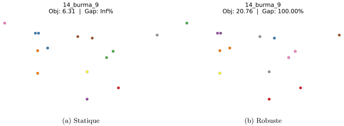
Figure 6: Instance : 14_burma_9
