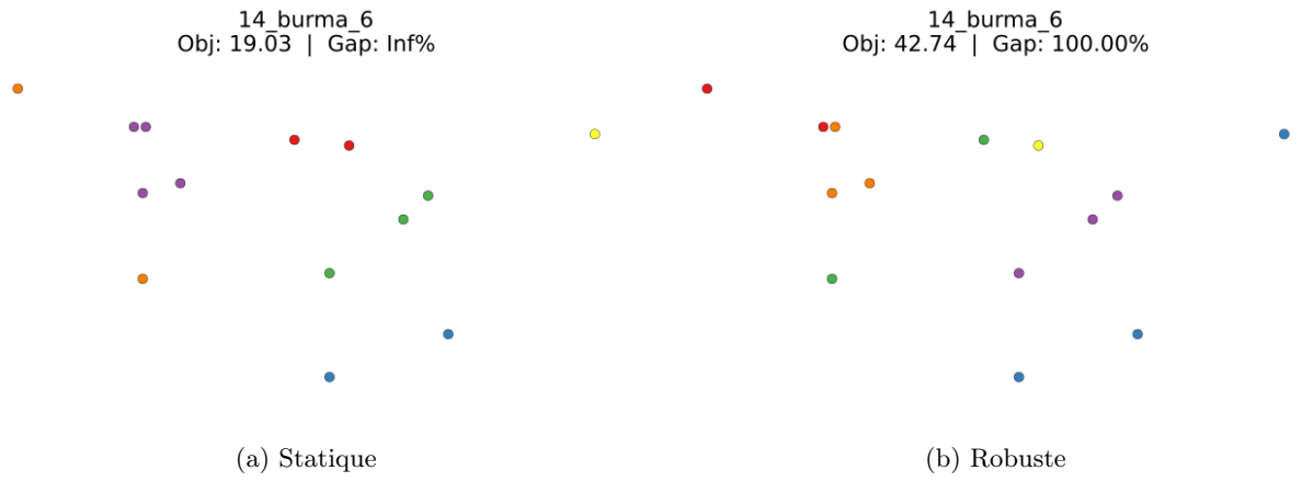
Figure 5: Instance : 14_burma_6
