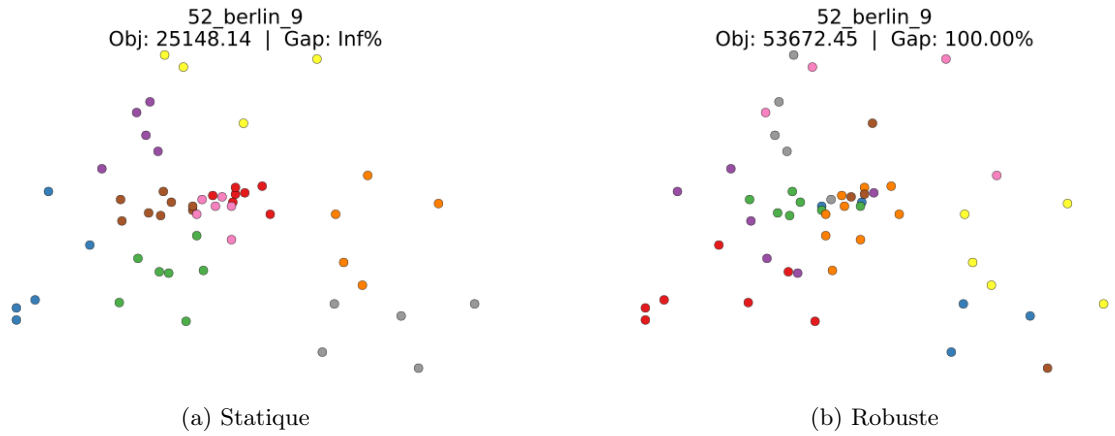
Figure 33: Instance : 52_berlin_9
