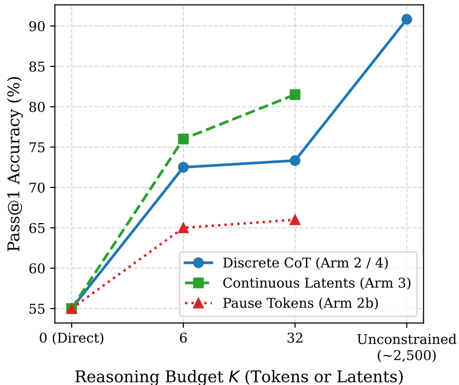
(b) MATH-500 Hard Subset (Levels 3-5, 240 Evals)
