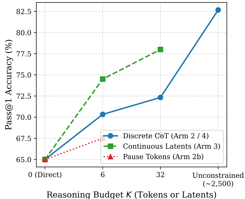
(a) GSM8K Arithmetic (600 Evals)
