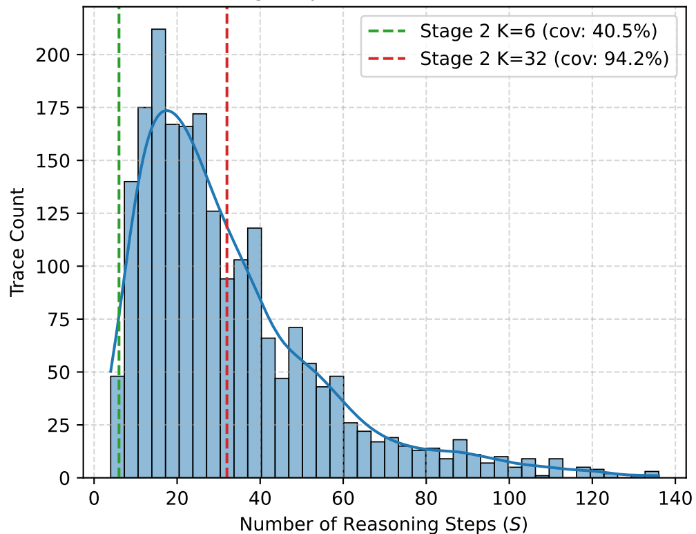
(a) Reasoning Step-Count Distribution (N=2,070)
