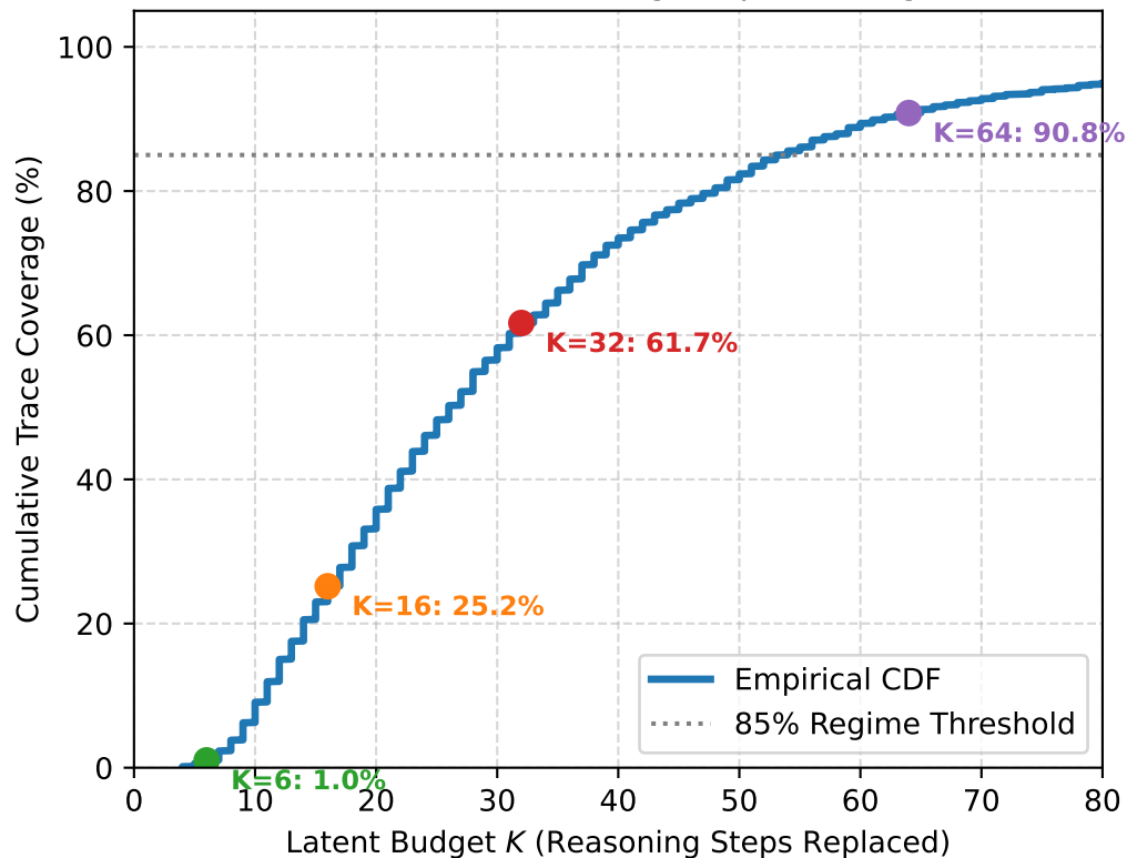
(b) Cumulative Reasoning Step Coverage CDF
