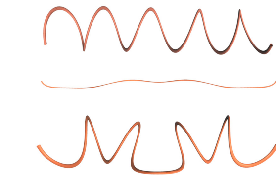
Figure 2: Helical perversion in experiment and simulation: starting from the natural shape of a Slinky® (top) we first remove writhe by pinching the flat cross-section between two fingers and traveling from one end to the other, arriving at a fully stretched, almost flat ribbon (middle). By bringing the ends together, a persistent perversion forms (bottom), whose shape is surprisingly different from the natural shape.
