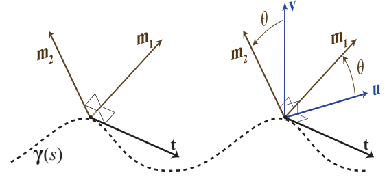
Figure 3: Adapted framed curve (Left) The configuration of an elastic rod is represented by a curve \boldsymbol{\gamma}(s) and a material frame \{\mathbf{t}(s), \mathbf{m}_1(s), \mathbf{m}_2(s)\} . (Right) The material frame is encoded by an angle of rotation \theta relative to the natural Bishop frame \{\mathbf{t}(s), \mathbf{u}(s), \mathbf{v}(s)\} .
