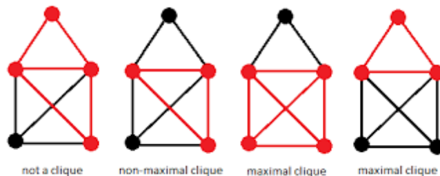
Figure 3. Cliques maximales.
