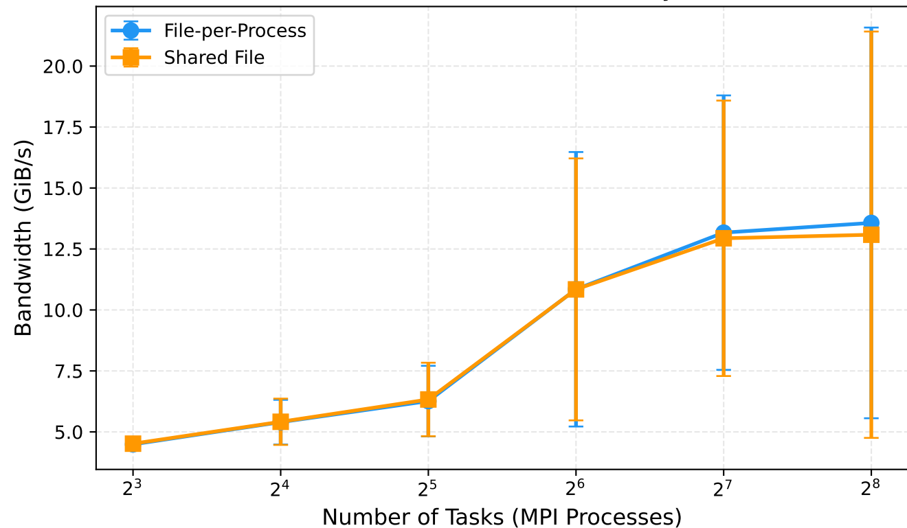
Read Bandwidth Scalability
