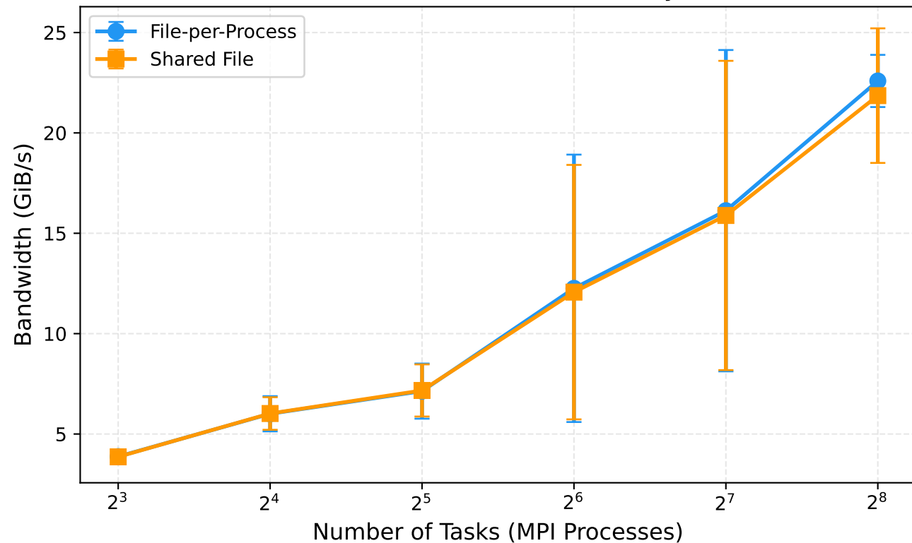
Write Bandwidth Scalability
