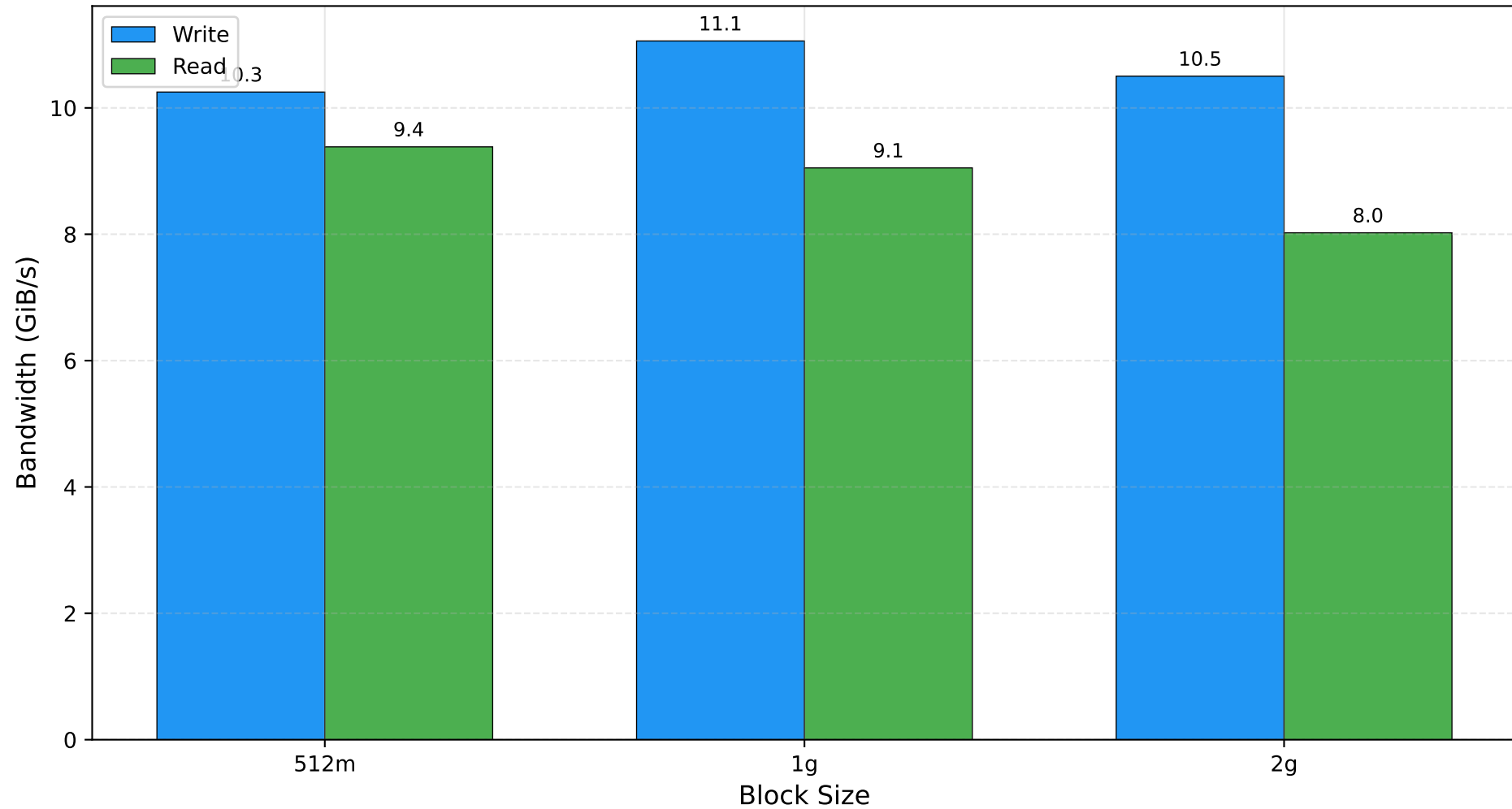
2025.11.27-09.29.18-large_scale - Shared File Bandwidth by Block Size
