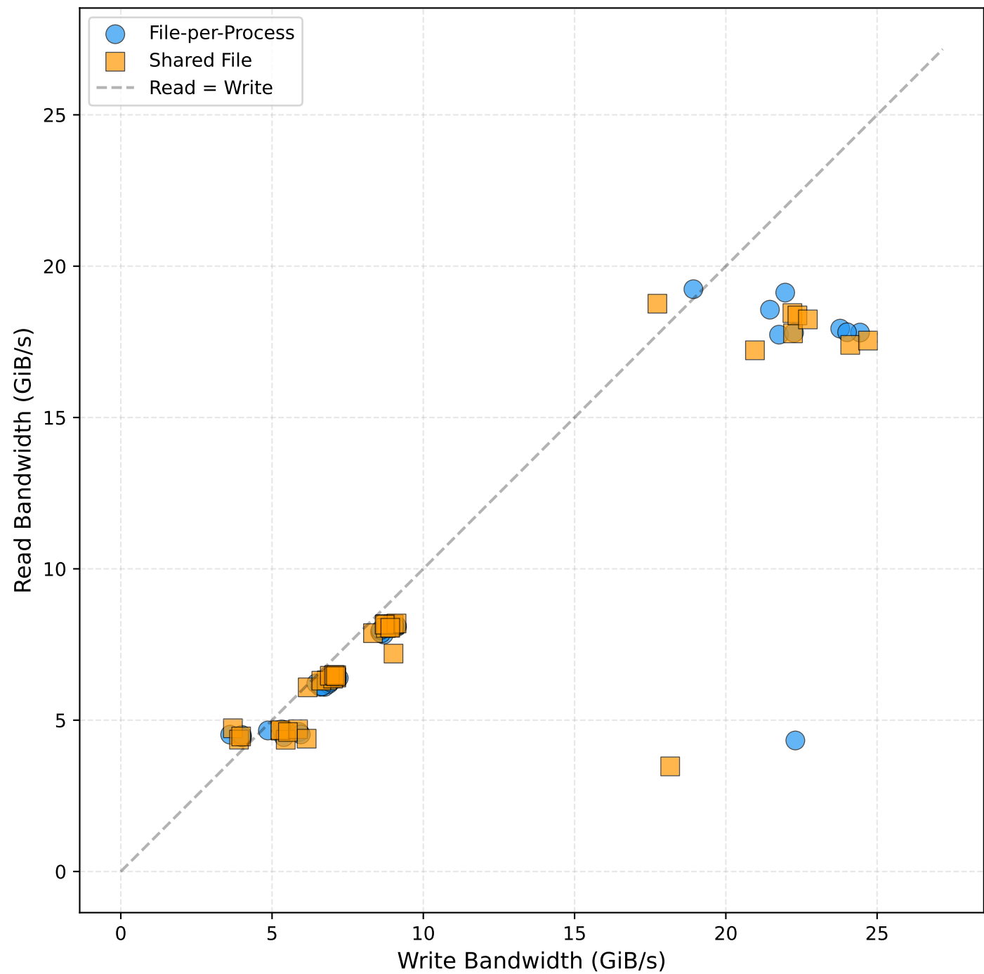
2025.11.27-09.29.18-large_scale Read vs Write Bandwidth
