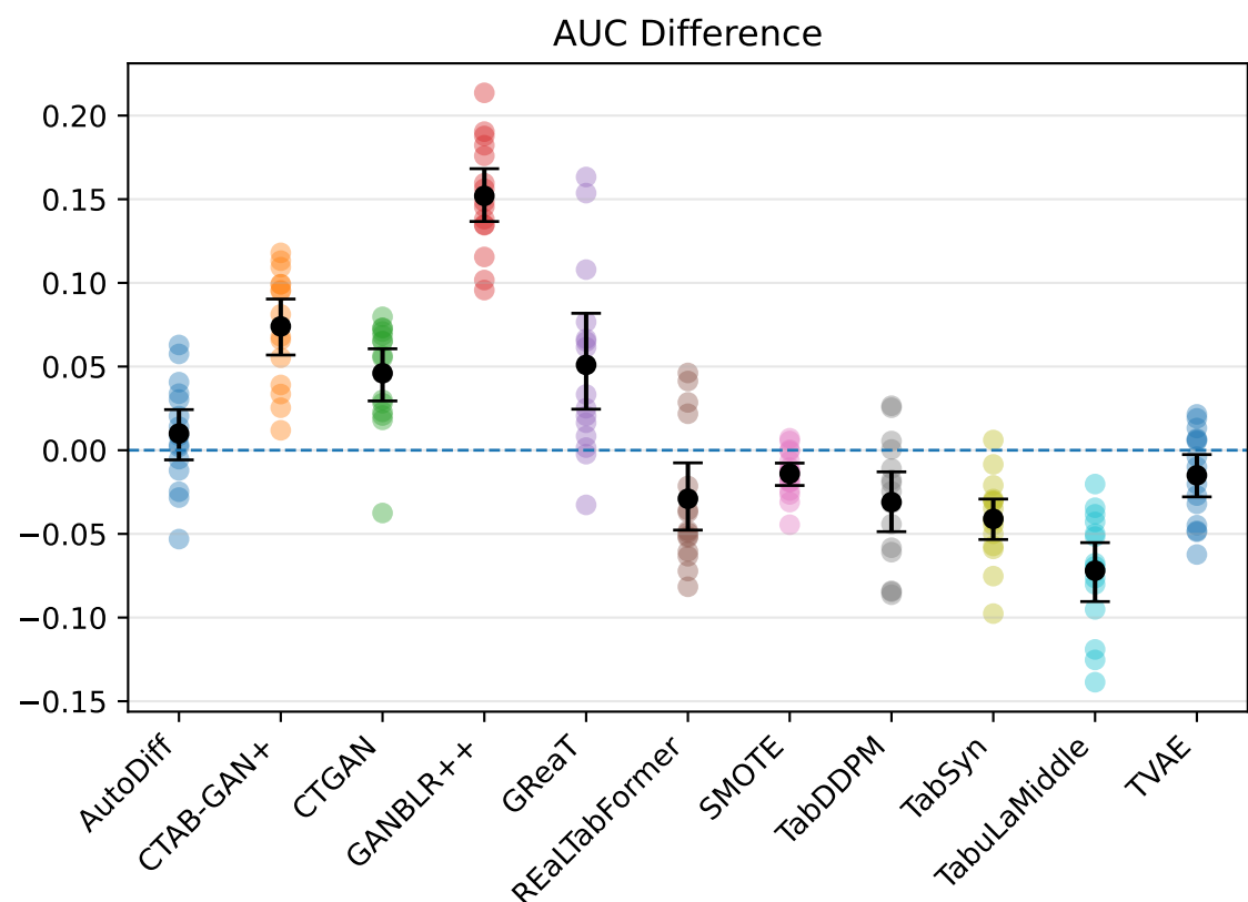
Utility Metrics with Confidence Intervals (Negative means better results)
