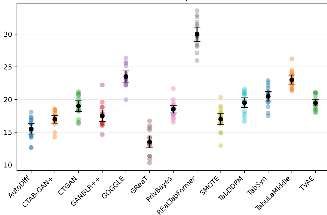
Runtime
