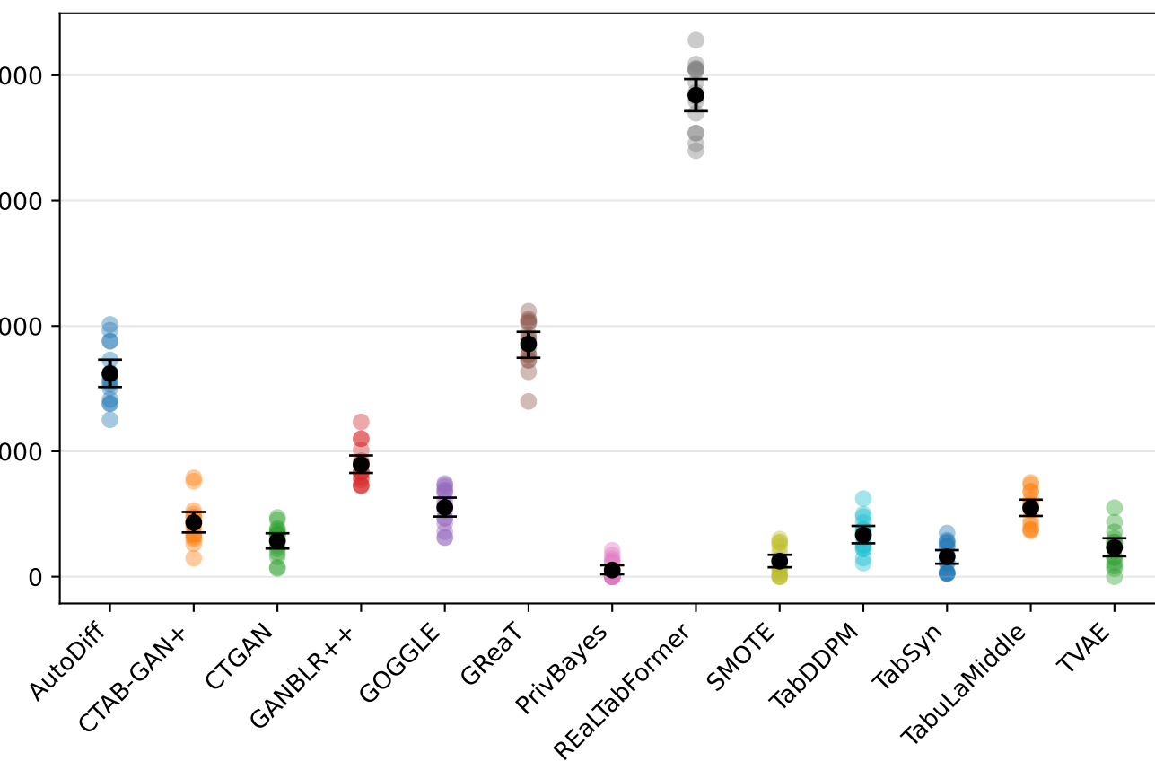
Runtime
