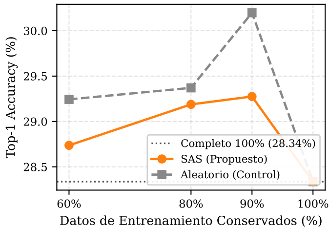
(c) CPC
