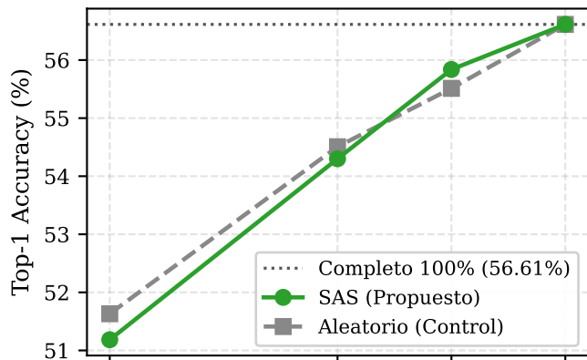
(c) CPC
