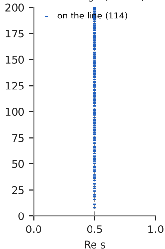
(c) L(s, \chi_{-3}) : mirror and merge (mod 3)
