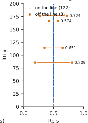
(b) Davenport-Heilbronn: mirror, no merge
