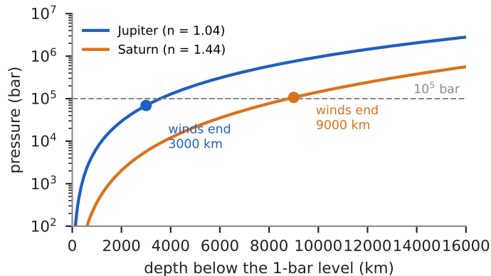
(b) the winds of both planets end near 10^5 bar
