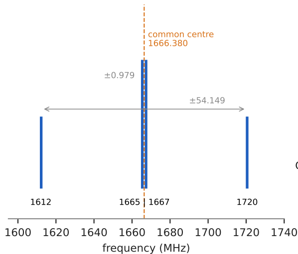
(c) 3I's OH lines: two pairs, one centre (1612+1720 = 1665+1667)
