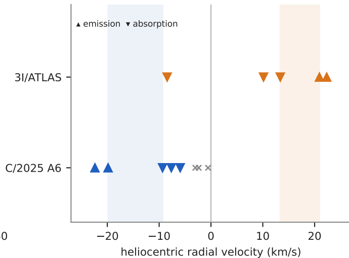
(d) OH flips where the inversion crosses zero (shaded)
