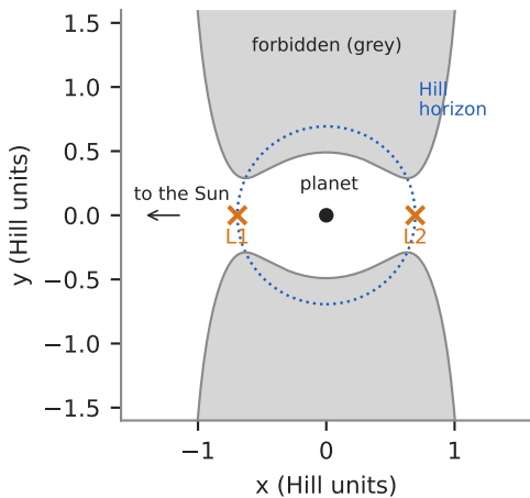
(a) two throats, one centre (same for every giant)
