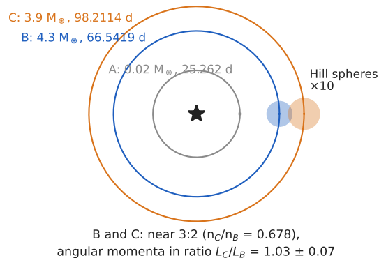
(e) PSR B1257+12: a centre, a balanced pair and a small third
