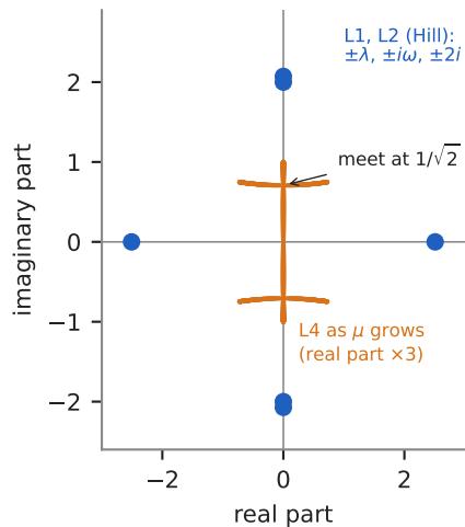
(b) the axis as horizon: throat pair off it, triangle on it
