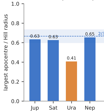
(c) moons reach two thirds of the horizon (not Uranus)
