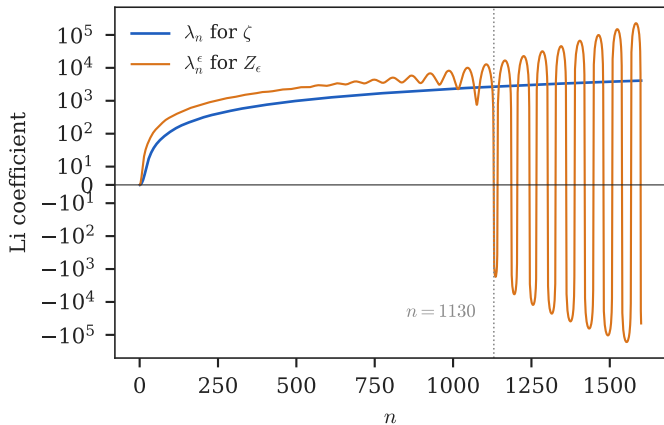
(a) Li coefficients, n \leq 1600
