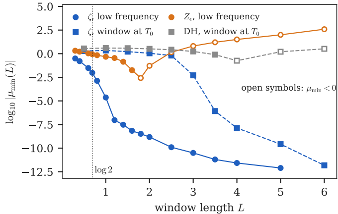
(b) smallest eigenvalue of the window form
