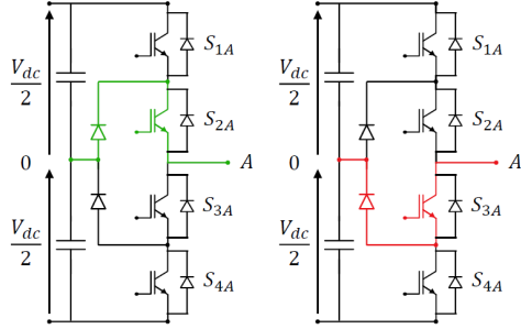
Fig. 2. Zero operating stage
