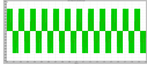
Fig. 8. Pole voltages and modulating signal
