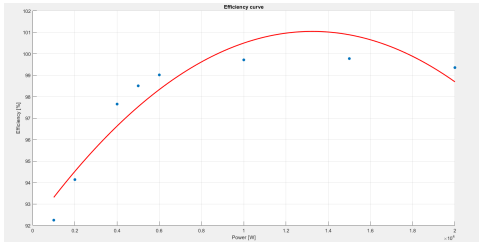
Fig. 22. Inverter efficiency curve
