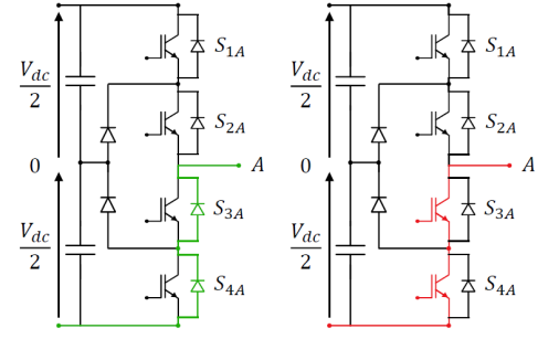
Fig. 3. Negative operating stage
