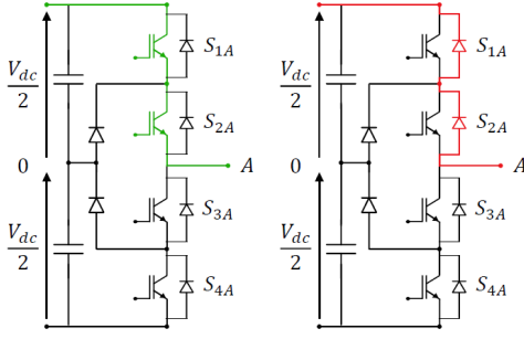
Fig. 1. Positive operating stage
