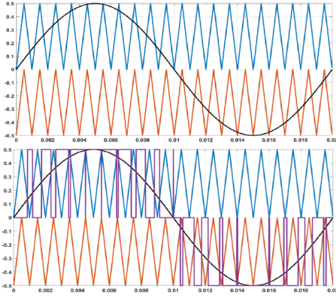
Fig. 4. Single leg PD
