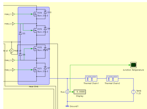
Fig. 19. Temperature simulation
