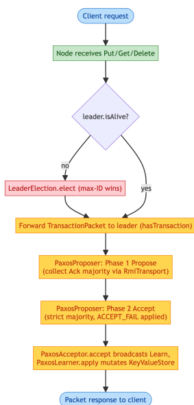
Figure 2: Transaction Lifecycle
