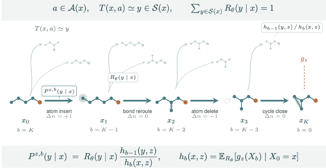
Figure 1: Overview of COMPOSE. The executor maps legal edits a \in \mathcal{A}(x) to canonical molecular successors y \in \mathcal{S}(x) , and the goal-independent kernel R_\theta(y | x) defines the reference process. Finite-horizon control reweights each transition by its remaining future value, P^{z,b}(y | x) = R_\theta(y | x) h_{b-1}(y, z) / h_b(x, z) , without introducing transitions outside the support of R_\theta .
