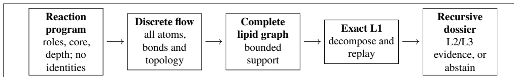
Figure 3: FORGE generates complete ionizable-lipid graphs within reaction-program coordinates. The reaction program specifies how molecular regions participate in an assembly without choosing their structures from a finite inventory. FORGE generates the complete molecular graph, verifies that the specified reaction reconstructs it, and recursively expands unavailable precursors until every branch terminates in evidence-qualified starting materials or the framework abstains. Exact replay and route closure are computational checks and do not establish experimental synthesis success.
