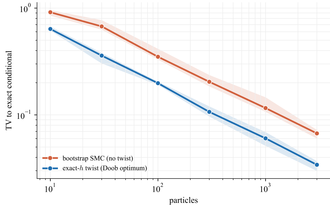
Guidance recovers the exact conditional (measured against ground truth)
