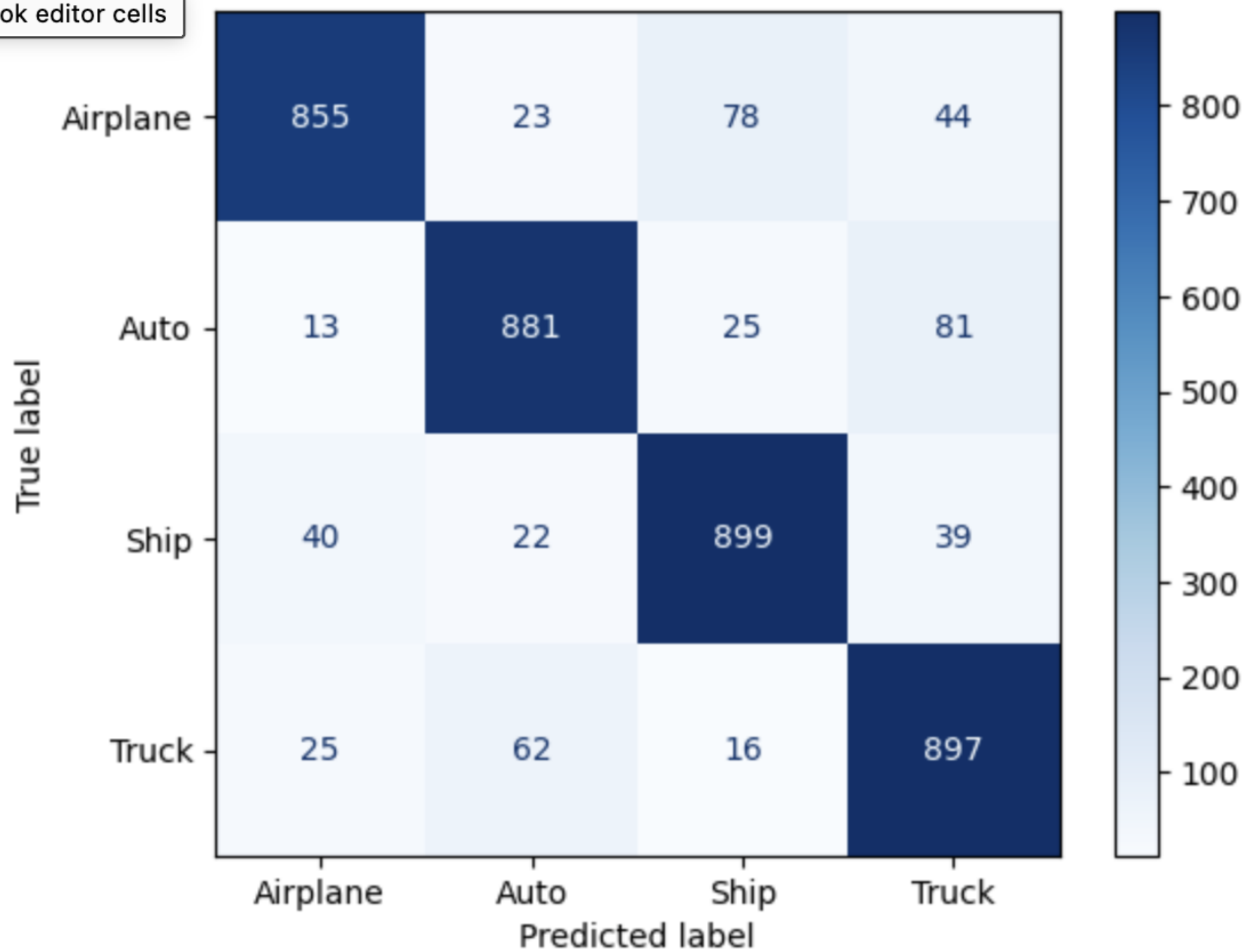
Confusion Matrix (Best Model)
