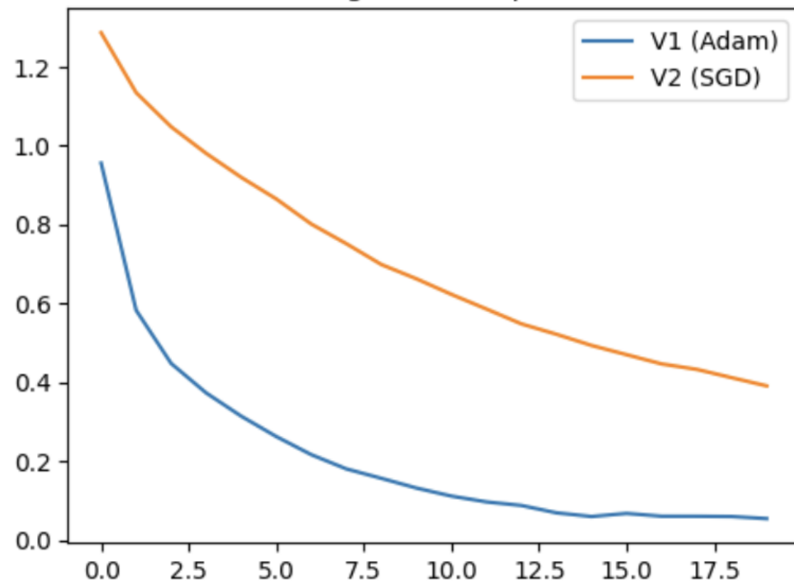
Training Loss Comparison
