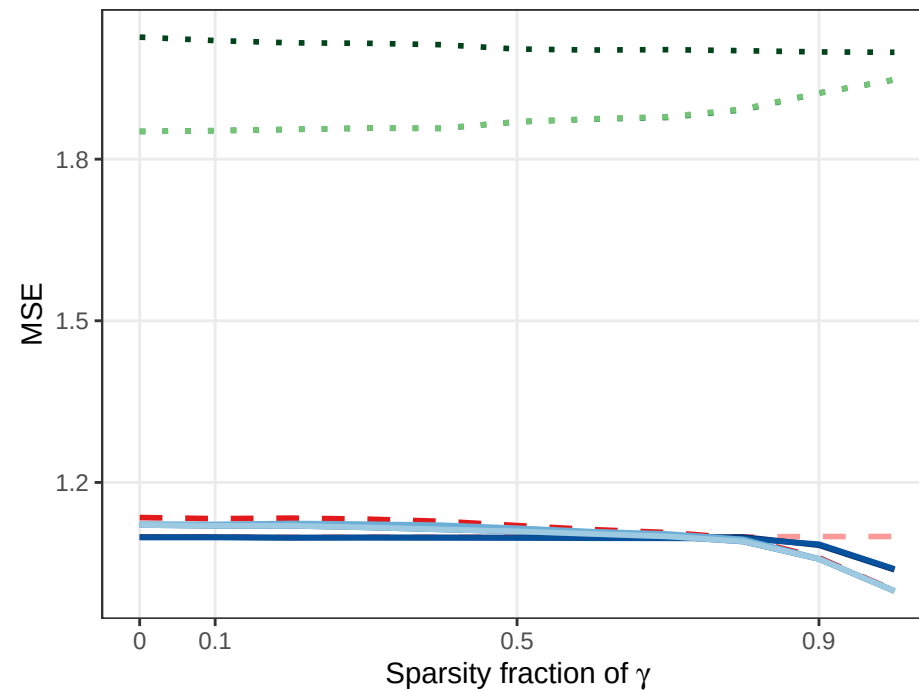
\gamma = 0.8, N=20, T^* = 16, H = 4
