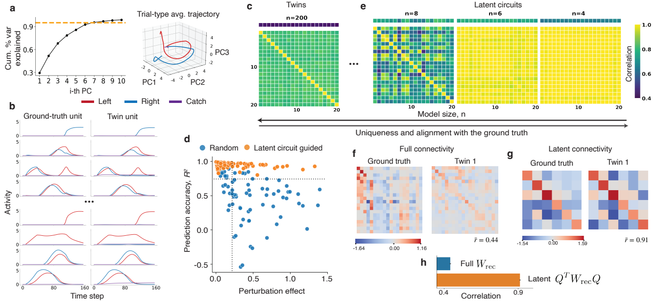
Fig 1: (a) The ground-truth RNN has low-dimensional dynamics during the task, with the first 7 PCs explaining over 95% of variance. (b) Trial-type averaged responses of example units in the ground-truth RNN (left) and one of its twins (right) show the one-to-one correspondence. (c) Correlation coefficients between W_{\text{rec}} of 20 best-fitting twin RNNs (square matrix) and between W_{\text{rec}} of each twin and the ground-truth RNN (top row). (d) Deviation from the normal task trajectories elicited by perturbations in the ground-truth RNN (x-axis) versus the accuracy of the twin in predicting the ground-truth RNN trajectories during the same perturbations (y-axis). The twin fails to reliably predict random perturbations (blue), but accurately predicts perturbations along columns of Q identified by a 6-dimensional latent circuit (orange). (e) Same as c for latent circuit models of varying dimension n . (f) The full recurrent connectivity W_{\text{rec}} vastly disagrees between the ground-truth RNN and its twins, shown for one example twin. (g) The latent low-dimensional connectivity, identified as Q^T W_{\text{rec}} Q , is highly similar between the ground-truth RNN and its twins, shown for the same example twin as in f. (h) Correlation coefficients between the latent connectivity Q^T W_{\text{rec}} Q of the ground-truth RNN and all twins are high (orange, \bar{r} = 0.91 ) despite low correlations between their full connectivity W_{\text{rec}} (blue, \bar{r} = 0.44 ).
