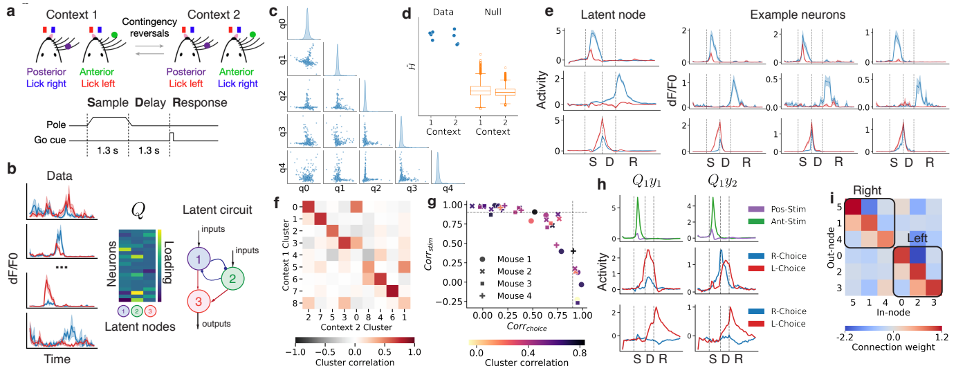
Fig 1: a , Task structure and contexts, adapted from [1]. b , Latent circuit inference identifies a subspace Q with task-relevant dynamics and a low-dimensional RNN that generates the dynamics within this subspace. Q defines the mapping between the latent nodes and neural activity patterns. c , Scatter plots of neuron loadings on pairs of columns q_i of Q show that each neuron is strongly weighted onto a single column, forming axis-aligned clusters. d , Q -matrices show significantly higher Hoyer sparsity compared to null (5,000 random rotations of Q , p < 10^{-10} ), confirming that neurons form non-overlapping clusters. e , The activity profiles of neurons in each cluster (right) closely resembled that of the corresponding latent node (left), confirming that latent nodes represent functional neural subpopulations, shown for three example nodes (rows). f , Matrix G^* summarizes how clusters identified in Context 1 (rows) align with clusters in Context 2 (columns), shown for an example animal. Diagonal entries quantify how well cluster membership is preserved across contexts for matched cluster pairs. g , Across animals, the cluster membership of neurons remained largely stable across contingencies (color-coded). Most clusters maintained their temporal dynamics and selectivity for either stimulus (high on y -axis) or choice (high x -axis). Dashed lines mark 0.9. Some clusters changed their selectivity and dynamics, while still maintaining stable membership (to the left and below 0.9 lines). h , Examples clusters that retained their temporal profile and selectivity (top: stable stimulus encoding, bottom: stable choice encoding). Example cluster that changed dynamics and selectivity after relearning (middle). i , Inferred latent recurrent connectivity w_{\text{rec}} revealed feedforward excitation (below the diagonal) and feedback inhibition (above the diagonal), forming two chains selective for the left and right choice, shown for an example animal.
