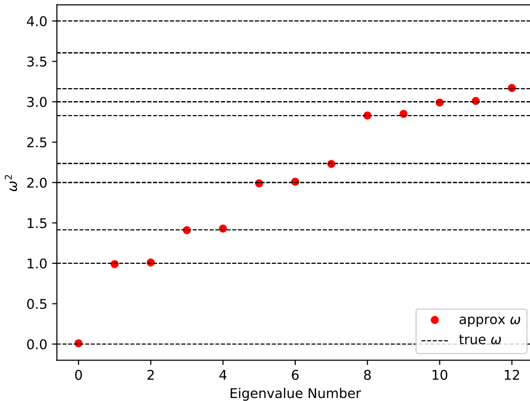
Comparing Exact and Computed \omega ( N = 128 )
