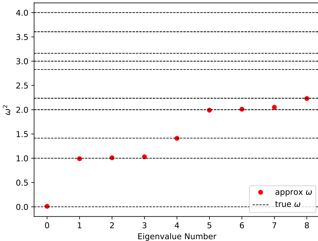
Comparing Exact and Computed \omega ( N = 32 )
