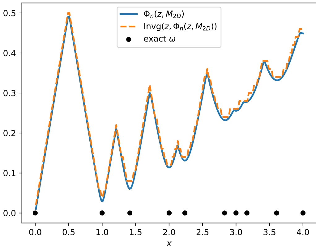
Approximations of \Phi_n(z, M_{2D}) , \text{Inv}g(z, \Phi_n(z, M_{2D})) , and \omega ( N = 32 )
