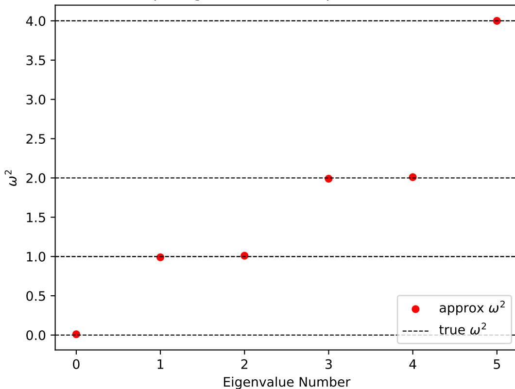
Comparing Exact and Computed \omega^2 ( N = 1 )
