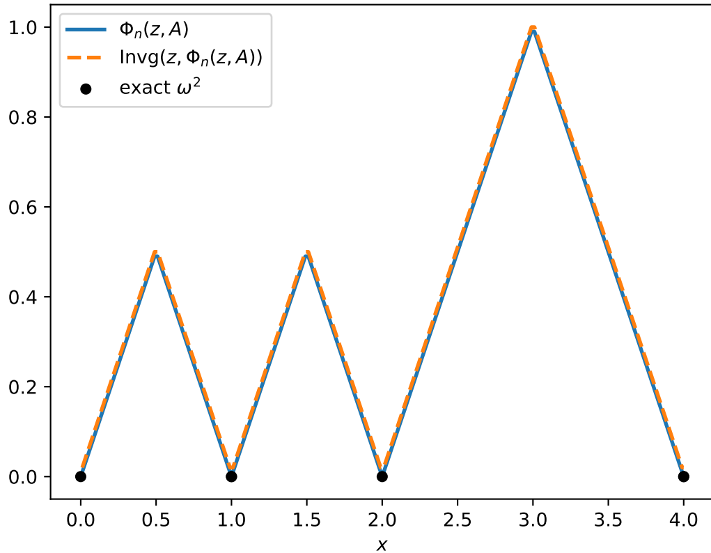
Approximations of \Phi_n(z, A) , \text{Invg}(z, \Phi_n(z, A)) , and \omega^2 ( N = 1 )
