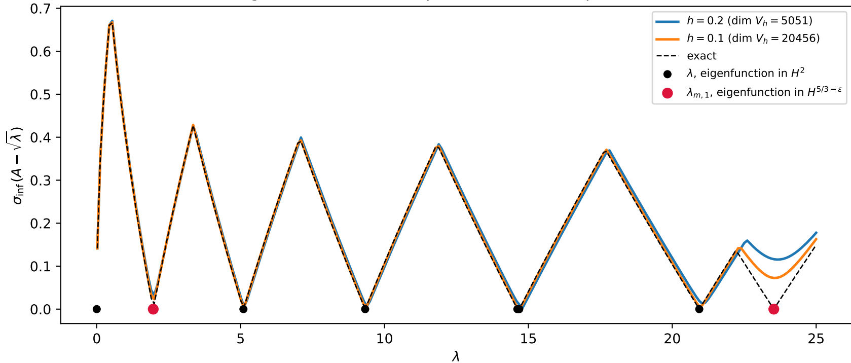
Dirac folding of the NEUMANN Laplacian, \text{CG}_5 \times \text{RT}_5 , pizza slice ( \omega = 3\pi/2 )
