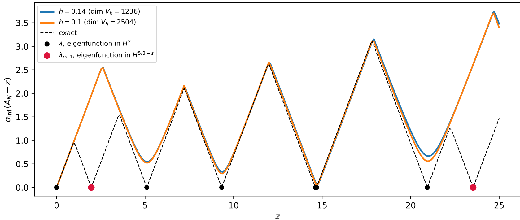
Folded Neumann Laplacian, Argyris, pizza slice ( \omega = 3\pi/2 )
