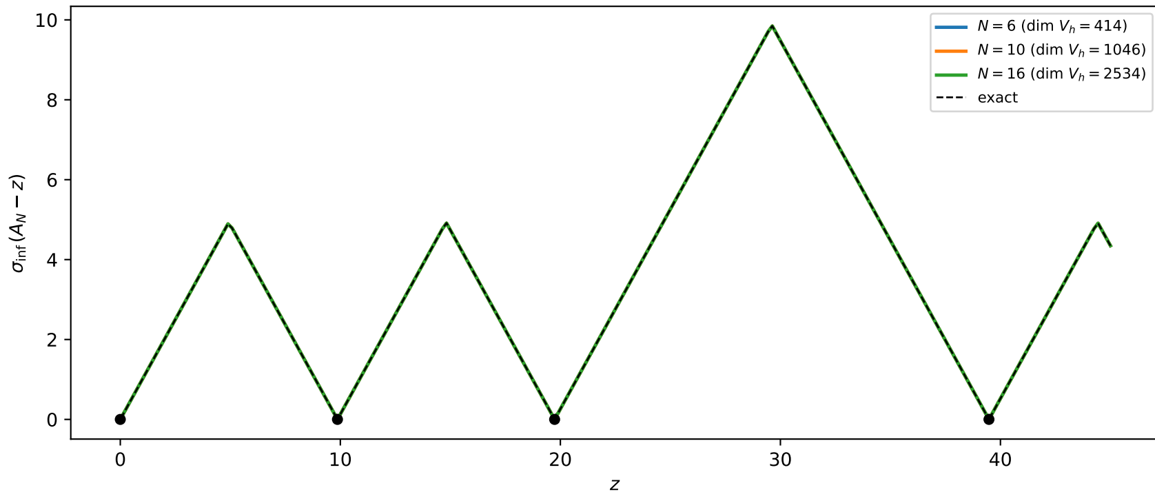
Folded Neumann Laplacian, Argyris, unit square
