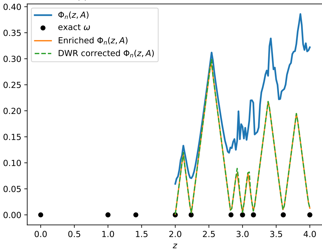
Approximations of \Phi_n(z, A) and \omega ( N = 32 )
