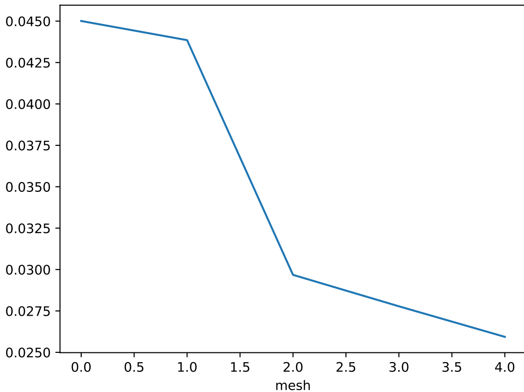
Error estimate over each mesh for z = 3.1000000000000001
