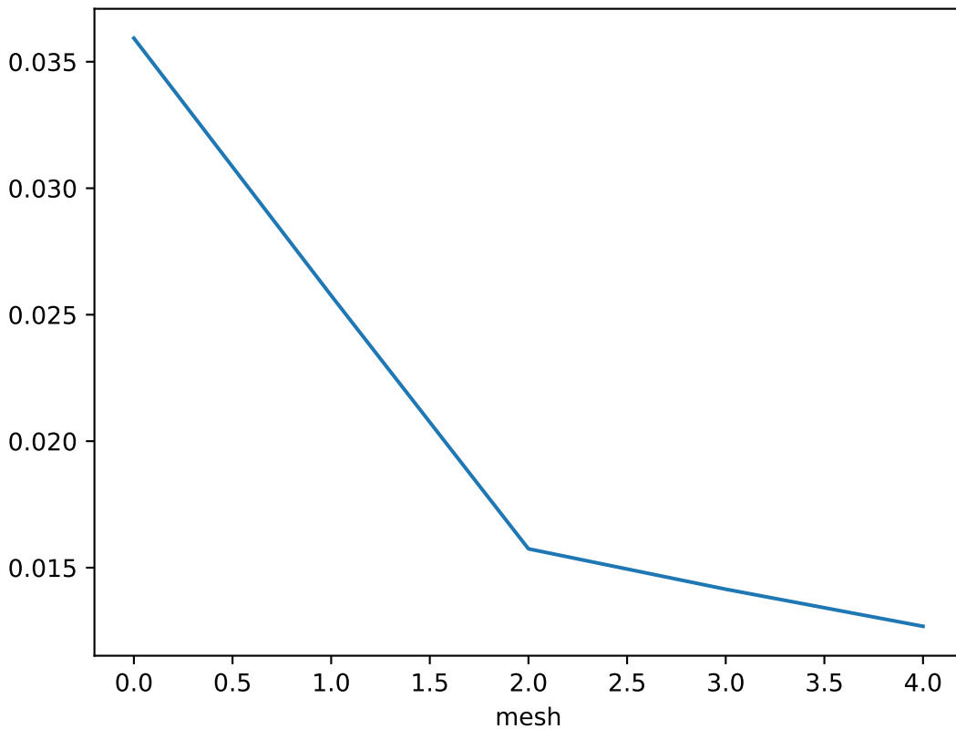
Error estimate over each mesh for z = 2.6800000000000006
