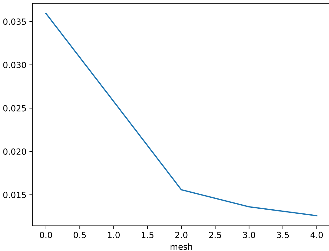
Error estimate over each mesh for z = 2.7000000000000006
